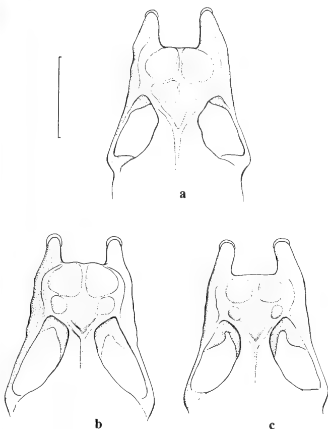
Fig. 2 Dorsal view of rostral part of skulls of a.) R. malayanus (BMNH 3.2.6.83 [holotype]), b.) R. s. stheno (BMNH 98.3.13.1 [holotype]) and c.) R. s. microglobosus (HNHM 98.1.1. [paratype]). Scale = 5 mm.
