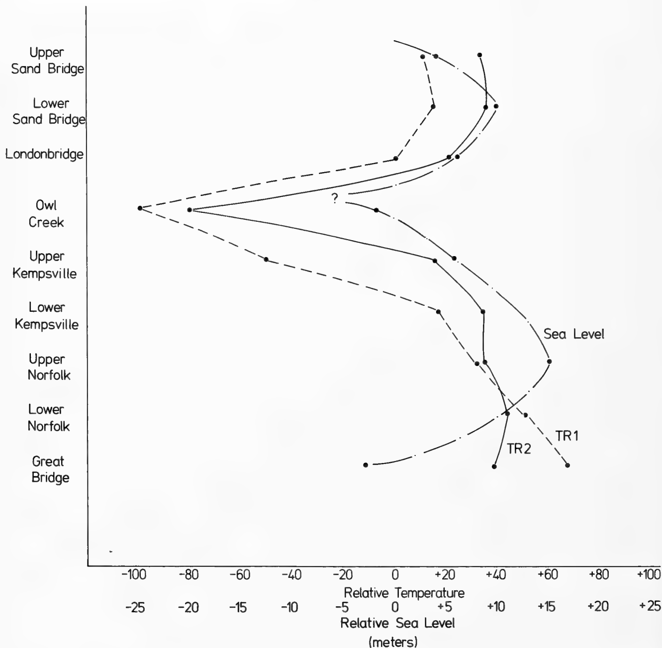
Text-figure 6. Inferred relative sea water temperature (based on formulas TR 1 and TR 2 ; see text and Table 12) and relative sea level for stratigraphic units in the study area. Both temperature curves indicate a time lag between temperature and sea level changes with changes in inferred sea temperature preceding changes in sea level.
