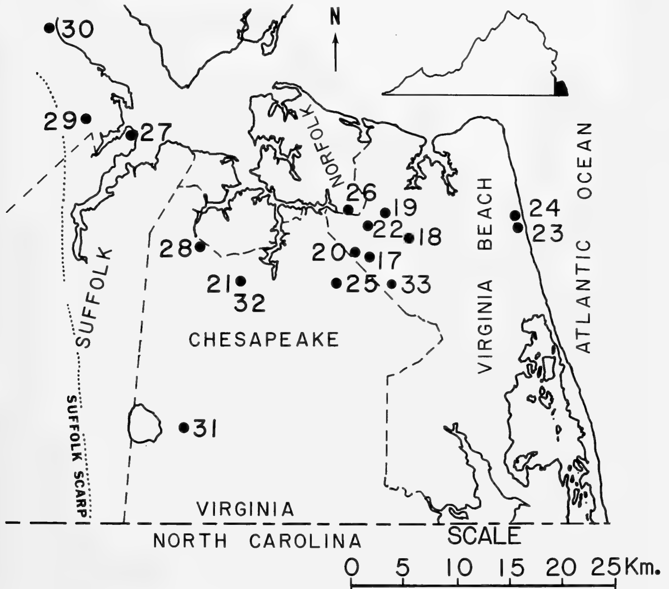
Text-figure 1.—Map of study area, southeastern Virginia, showing locations of collecting localities.
