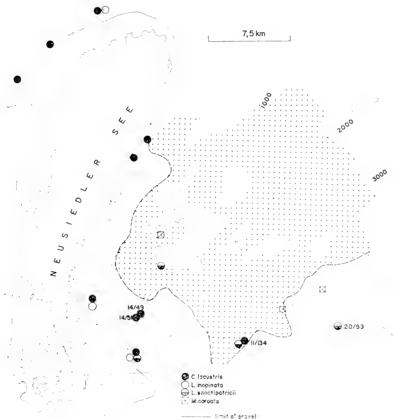
Text-fig. 3. — Localities of subfossil Cytherissa lacustris , Limnocythere sanctipatricii , Limnocythere inopinata , and Metacypris cordata east and west of Neusiedlersee (its configuration presented together with the extent of the Phragmites belt). Numbers indicate the drilling profiles carried out by ÖMV in 1971. Dotted area: extent of Pleistocene gravel. Broken lines: Depth of rock. From Löffler (1972).
