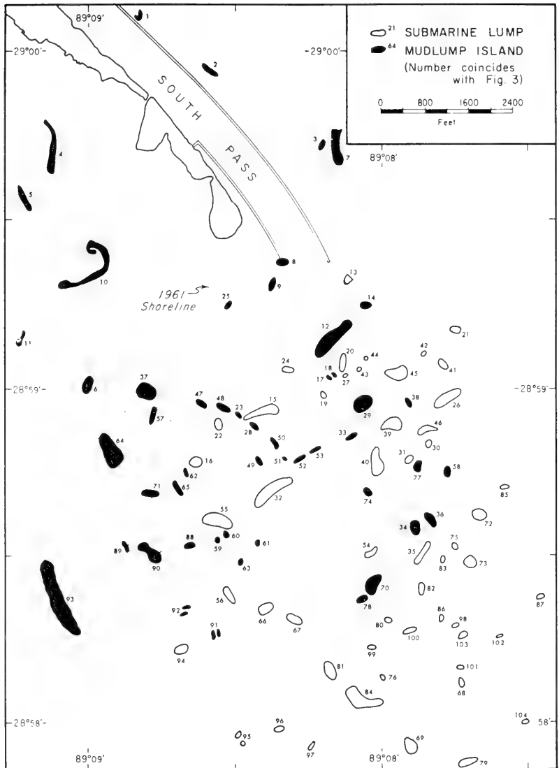
Text-figure 1. Mudlump distribution South Pass. Data from 123 maps dated between 1867-1961. (After Morgan, 1963, fig. 2.)
