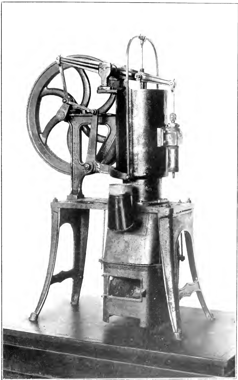
ERICSSON HOT-AIR PUMPING ENGINE. 1905
