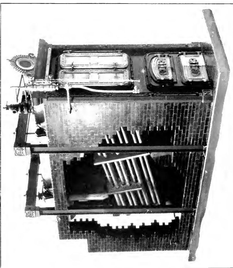
NATIONAL WATER-TUBE BOILER, 1885 Model (U.S.N.M. no. 309374). See p. 115.
