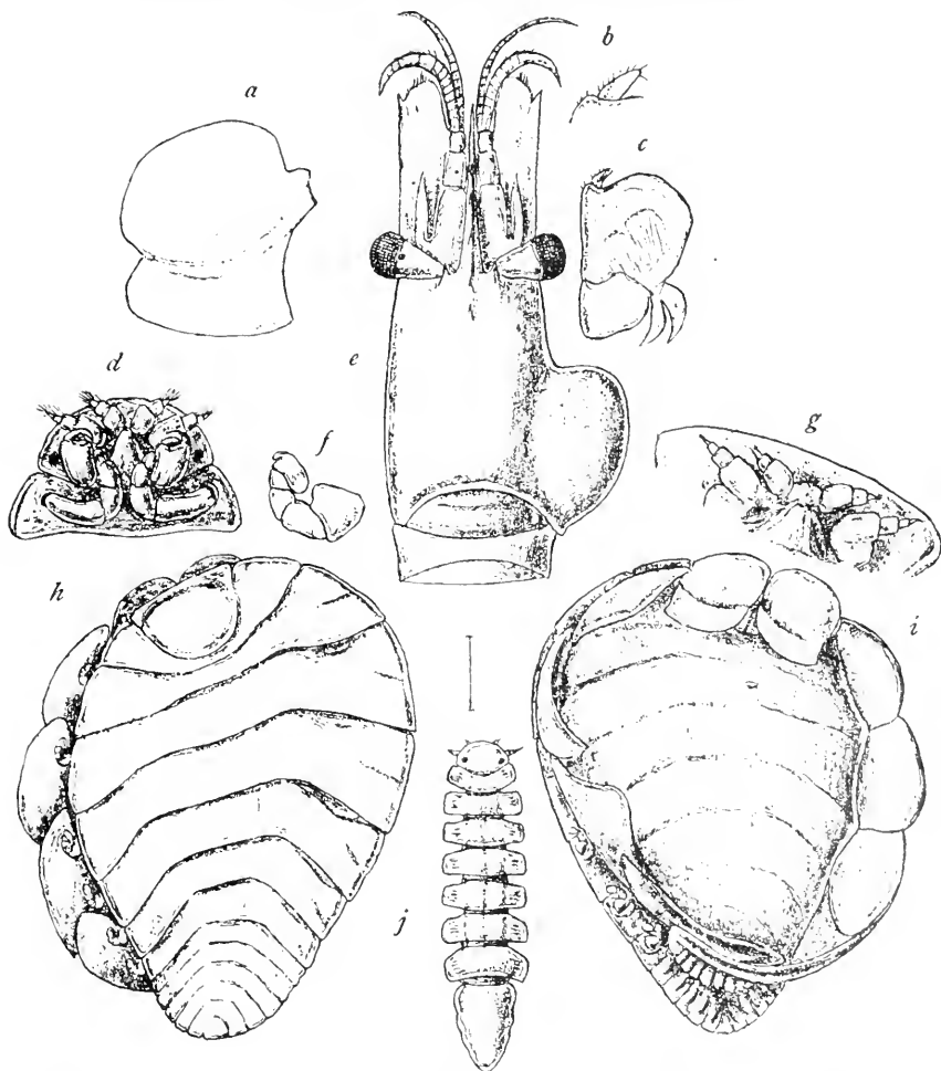
FIG. 628.—BOPYROIDES HIPPOLYTES (AFTER SARR). a , FIRST INCUBATORY PLATE. b , PALP OF MAXILLIPED. c , MAXILLIPED. d , HEAD OF MALE (VENTRAL VIEW). e , ANTERIOR PART OF SPECIMEN OF SPIRONTOCARIS POLARIS INFESTED WITH THIS PARASITE. f , LEG. g , ANTERIOR PART OF HEAD OF FEMALE (VENTRAL VIEW). h , DORSAL VIEW OF FEMALE. i , VENTRAL VIEW OF FEMALE. j , DORSAL VIEW OF MALE.
