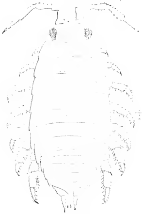
FIG. 710.—SCYPHACELLA ARENICOLA (AFTER HARGER). — 12.
