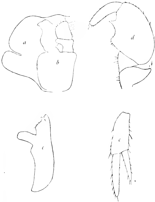
FIG. 162.—MANCASELLUS MACROURUS (AFTER GARMAN). a , OUTLINE OF ONE SIDE OF HEAD. b , ONE OF SECOND GENITAL PLATES OF MALE. c , MANDIBLE. d , HAND. e , UROPOD.
