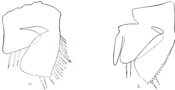
FIG. 333.— PARADYNAMENE BENJAMENSIS . a , FIRST PLEPOD OF MALE. — 15 \frac{1}{2} . b , SECOND PLEPOD OF MALE. — 15 \frac{1}{2} .
