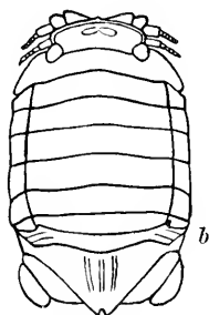
FIG. 327.—DYNAMENE DILATATA. a, HEAD AND FIRST THORACIC SEGMENT. · 13 \frac{1}{2} . b, DORSAL VIEW. · 10 \frac{1}{2} .
