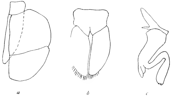
FIG. 500.—STENETERIUM STEBBINGI. a , THIRD PLEPOD OF MALE. b , FIRST PLEPOD OF MALE. c , SECOND PLEPOD OF MALE. — 77 \frac{1}{2} .
