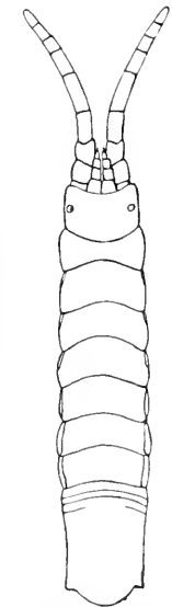
FIG. 458.—CLEANTIS HEATHII. \times 6\frac{1}{2} .
