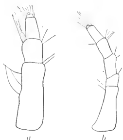
FIG. 13.—TANAIS ALASCENSIS. a , FIRST ANTENNA. \times 39 . b , SECOND ANTENNA. \times 39 .
