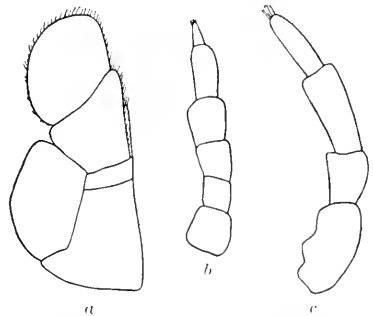
FIG. 140.—EDOTEA ACUTA. a , MAXILLIPED. \times 51\frac{1}{2} . b , SECOND ANTENNA. \times 51\frac{1}{2} . c , FIRST ANTENNA. \times 51\frac{1}{2} .
