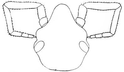
FIG. 711.—SCYPHACELLA ARENICOLA. HEAD WITH ANTENNA. — 27 \frac{1}{2} .
