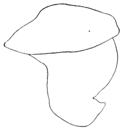
FIG. 626.—BOPYRINA UROCARIDIS. FIRST LAMELLA OF MARSUPIUM, RIGHT SIDE. \times 52 .
