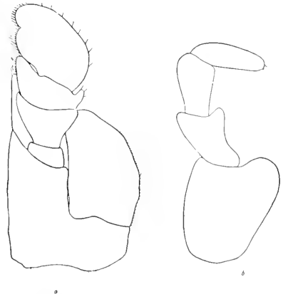
FIG. 397.— IDOTHEA OCHOTENSIS . a , MAXILLIPED. - 15 \mu . b , FIRST ANTENNA. - 15 \mu .
