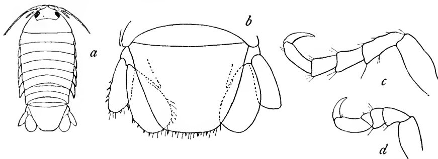
FIG. 87.— CIOROLANA OBTRUNCATA (AFTER MOORE). a , GENERAL FIGURE. b , ABDOMEN (LAST SEGMENT WITH UROPODA). c , SEVENTH LEG. d , FIRST LEG.
