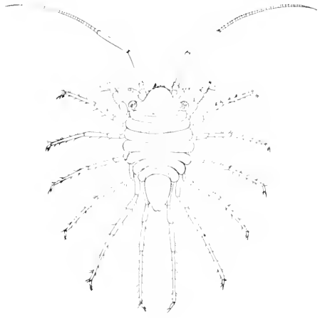
FIG. 538.—MUNNA FABRICII (AFTER HARGER). — 20.
