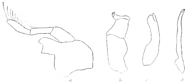
FIG. 220.— EGATHOA OCLATA . a , MANDIBLE. \times 51\frac{1}{2} . b , MAXILLIPED. \times 51\frac{1}{2} . c , SECOND MAXILLA. d , FIRST MAXILLA. \times 51\frac{1}{2} .
