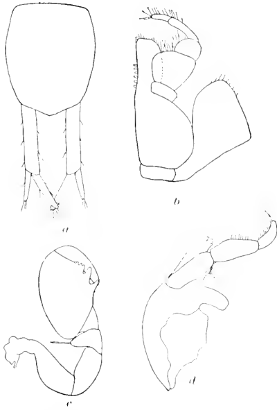
FIG. 191.— CECIDOTEA STYGIA . a , TERMINAL SEGMENT OF BODY AND UROPODA. \times 20\frac{1}{2} . b , MAXILLA. \times 38\frac{1}{2} . c , FIRST LEG. \times 20\frac{1}{2} . d , MANDIBLE. \times 38\frac{1}{2} .
