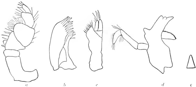
FIG. 105.—CIROLANIDES TEXENSIS. a , MAXILLIPED. \times 27\frac{1}{2} . b , FIRST MAXILLA. \times 27\frac{1}{2} . c , SECOND MAXILLA. \times 27\frac{1}{2} . d , MANDIBLE. \times 27\frac{1}{2} . e , FRONTAL LAMINA. \times 51\frac{1}{2} .
