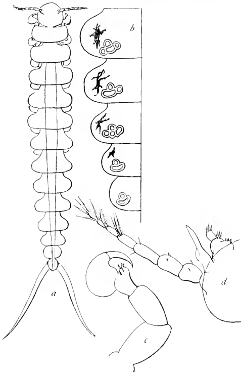
FIG. 560.—LEIDYA DISTORTA (AFTER LEIDY). a , DORSAL VIEW OF MALE. b , ABDOMINAL SEGMENTS OF MALE WITH PECULIAR APPENDAGES. c , RIGHT LEG OF MALE. d , HEAD OF MALE WITH ANTENNAE. ALL MAGNIFIED.
