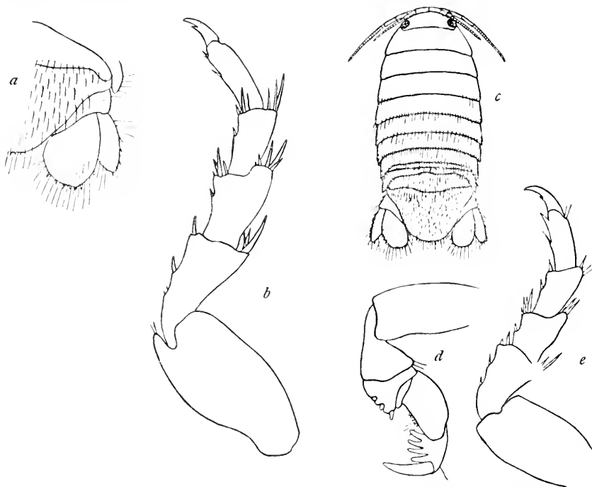
FIG. 110.—ALCIROA HIRSETA (AFTER MOORE). a , RIGHT SIDE OF TERMINAL ABDOMINAL SEGMENT WITH UROPOD. b , SEVENTH LEG. \times 40 . c , GENERAL FIGURE. \times 8 . d , FIRST LEG. \times 10 . e , FOURTH LEG. \times 40 .
