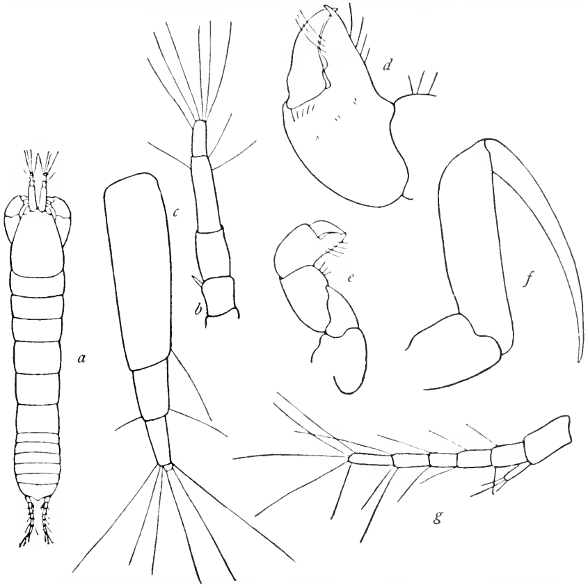
FIG. 29.—LEPTOCHEILIA DUBIA (AFTER MOORE). a , GENERAL FIGURE. \times 14 . b , FIRST ANTENNA. \times 77 . c , SECOND ANTENNA. \times 77 . d , CHELA. \times 77 . e , CHELIPED. \times 33 . f , END OF SECOND LEG. \times 77 . g , UROPOD. \times 77 . (Female).
