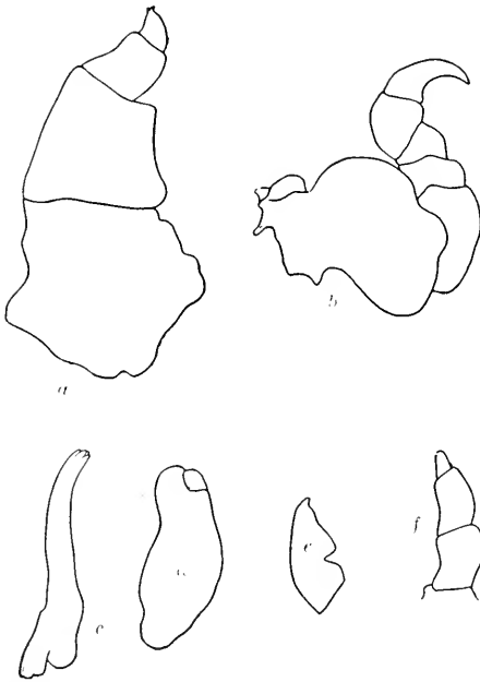
FIG. 264.— CYMOTHOA OESTRUM . a, MAXILLIPED. . . 15 \frac{1}{2} . b, SEVENTH LEG. . . 4 \frac{1}{2} . c, FIRST MAXILLA. . . 15 \frac{1}{2} . d, SECOND MAXILLA. . . 15 \frac{1}{2} . e, MANDIBLE. . . 15 \frac{1}{2} . f, PALP OF MANDIBLE. . . 15 \frac{1}{2} .
