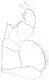
FIG. 378.—MESIDOTEA SABINI. MAXILLIPED. \times 11\frac{1}{2} .
