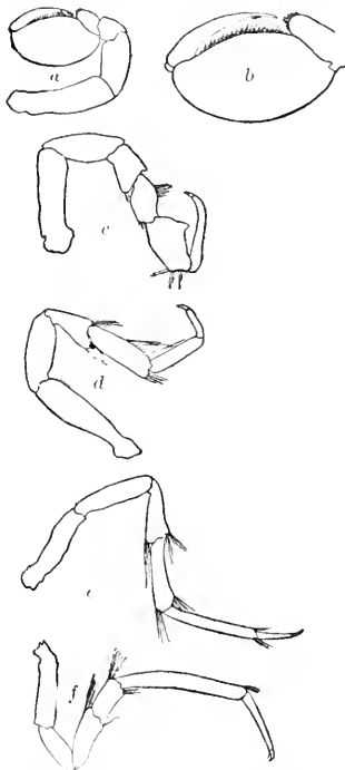
FIG. 289.— TECTICEPS ALASCENSIS . a , LEG OF FIRST PAIR. \times 5\frac{1}{2} . b , LAST TWO JOINTS OF SAME. \times 10\frac{1}{2} . c , LEG OF SECOND PAIR OF MALE. \times 5\frac{1}{2} . d , LEG OF THIRD PAIR. \times 5\frac{1}{2} . e , LEG OF SIXTH PAIR. \times 5\frac{1}{2} . f , LEG OF SEVENTH PAIR. \times 5\frac{1}{2} .
