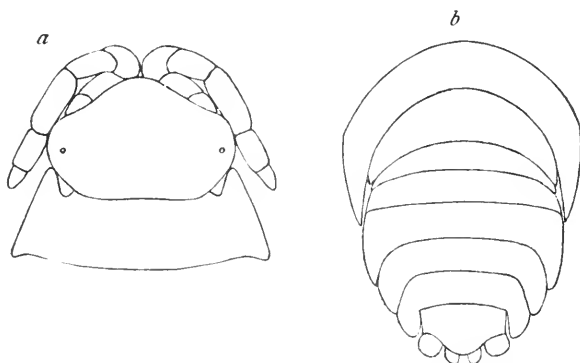
FIG. 709.—UROPODIAS BERMUDENSIS. a, HEAD AND FIRST THORACIC SEGMENT. 62. b, ABDOMEN AND LAST TWO THORACIC SEGMENTS. 62.
