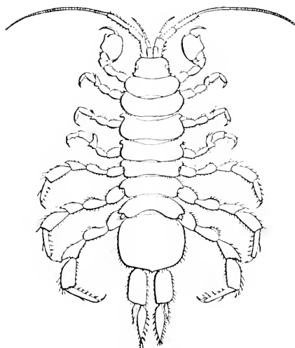
FIG. 472.—ASEILLUS COMMUNIS (AFTER SMITH).
