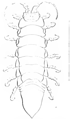
FIG. 398.—IDOTHEA PHOSPHOREA (AFTER HARGER). — 2.
