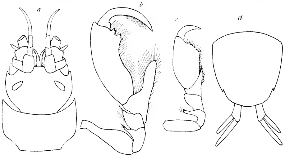
FIG. 199.— STENETRIUM STEBBINGI . a , HEAD AND FIRST THORACIC SEGMENTS. b , FIRST LEG OF MALE. c , FIRST LEG OF FEMALE. d , TERMINAL SEGMENT OF BODY AND UROPODA.
