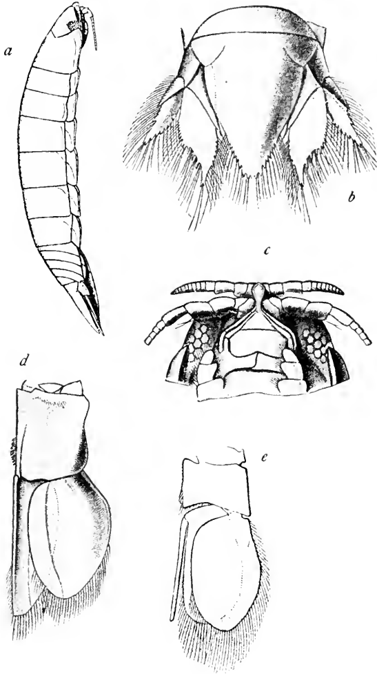
FIG. 100.— COSTIERA CYLINDRACEA (AFTER HANSEN). a , LATERAL VIEW OF FEMALE. b , POSTERIOR PART OF ABDOMEN OF ADULT FEMALE. c , ANTERIOR PART OF HEAD. d , LEFT PLEOPOD OF FIRST PAIR IN ADULT MALE. e , LEFT PLEOPOD OF SECOND PAIR IN ADULT MALE. (ENLARGED.)
