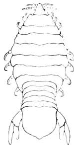
FIG. 232.—ANILOCRA PLEBIA (AFTER SCHICÆDTE AND MEINERT). YOUNG FEMALE. (ENLARGED.)
