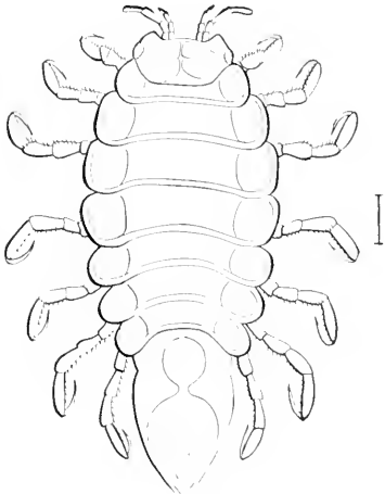
FIG. 41.—EDOTEA TRILOBA (AFTER HARGER). \times 10 .
