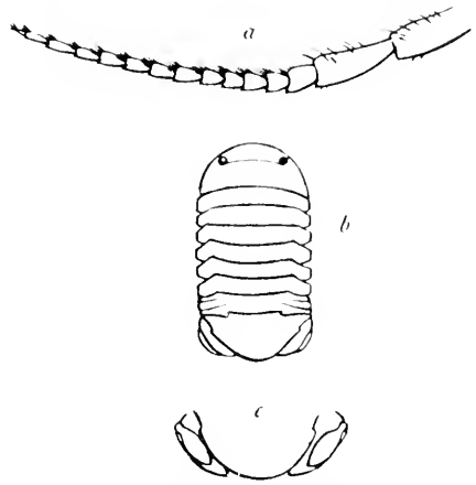
FIG. 315.— EXOSPILIEROMA OREGONENSIS (AFTER DANAI). a , SECOND ANTENNA. b , GENERAL FIGURE. c , ABDOMEN (UNDERSIDE). (TAIL ENLARGED.)
