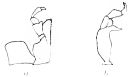
FIG. 181.—ASEILLUS ATTENUATUS. a, MANILLIPED. b, MANDIBLE.
