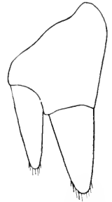
FIG. 738.—TRICHONISCUS PAPILLICORNIS. UROPODA OF LEFT SIDE. \times 77 .
