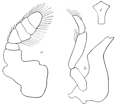
FIG. 138.—ALCIRONA KREBSII. a , MAXILLIPED. \cdot \frac{1}{51\frac{1}{2}} . b , MANDIBLE. \cdot \frac{1}{51\frac{1}{2}} . c , FRONTAL LAMINA. \cdot \frac{1}{51\frac{1}{2}} .
