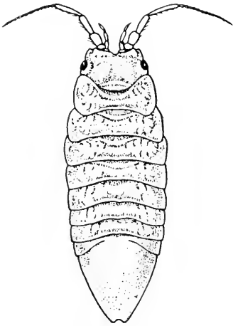
FIG. 122.— SYNIDOTEA MARMORATA (AFTER BENEDICT). . . 24.
