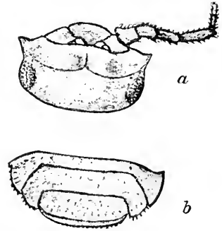
FIG. 647.—TYLOS LATREILLI (AFTER DOLLEFS). a, HEAD WITH ANTENNA. b, LAST TWO SEGMENTS OF ABDOMEN. (ENLARGED.)
