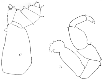
FIG. 727.— LIGYDA PALLASHI . a , MAXILLIPED. \times 20 . b , FIRST LEG OF MALE. \times 71 .
