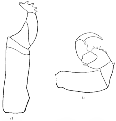
FIG. 150.— EGA ANTILLENIS . a , MAXILLIPED. \times 27\frac{1}{2} . b , LEG OF SECOND PAIR. \times 9\frac{1}{2} .
