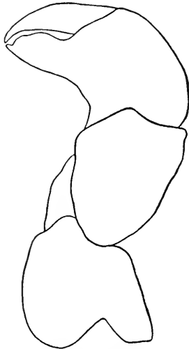
FIG. 17.—TANAIIS NORMANI. FIRST GNATHOPOD. \times 44 .
