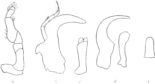
FIG. 132.—EXOCORALLANA ANTILLESIS. a , MAXILLIPED. \times 27\frac{1}{2} . b , MANDIBLE. \times 27\frac{1}{2} . c , SECOND MAXILLA. \times 27\frac{1}{2} . d , FIRST MAXILLA (OUTER AND INNER LOBE). \times 27\frac{1}{2} . e , FRONTAL LAMINA. \times 27\frac{1}{2} .
