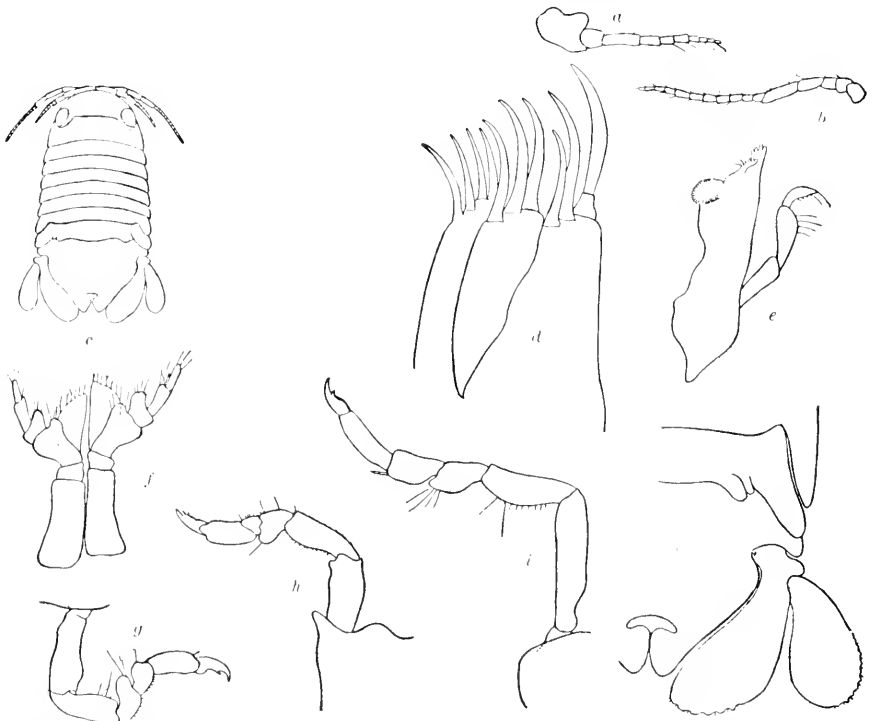
FIG. 320.—DYNAMENE PERFORATA (AFTER MOORE). a, FIRST ANTENNA. b, SECOND ANTENNA. c, MALE. d, TIP OF MAXILLA. e, MANDIBLE. f, MAXILLIPEDS. g, FOURTH LEG. h, FIRST LEG. i, SEVENTH LEG. j, PART OF TERMINAL SEGMENT OF ABDOMEN WITH TROCHOD.
