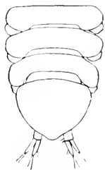
FIG. 508.—JANIROPSIS CALIFORNICA. TERMINAL PART OF BODY. - 27.
