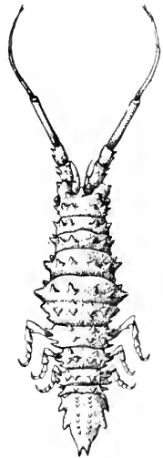
FIG. 371.—PLEUROPRION MURDOCHI (AFTER BENEDICT), p. 31.
