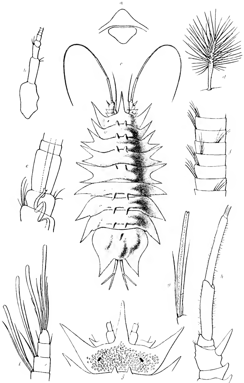
FIG. 516.— IOLELLA SPECTOSA (AFTER BOVALLIUS). a , LABRUM. b , INNER ANTENNA. \times 20 . c , DORSAL VIEW OF ANIMAL. \times 4 . d , AUDITORY BRISTLE FROM THE THIRD JOINT OF THE PEDUNCLE OF THE INNER ANTENNA. \times 160 . e , FIRST JOINTS OF THE FLAGELLUM OF THE INNER ANTENNA. \times 160 . f , SOME ARTICLES OF THE FLAGELLUM OF THE OUTER ANTENNA. \times 60 . g , AN OLFACTORY GLAND OF SAME. \times 260 . h , PEDUNCLE OF OUTER ANTENNA. \times 15 . i , THE LAST JOINTS OF SAME. \times 200 . j , HEAD. \times 10 .
