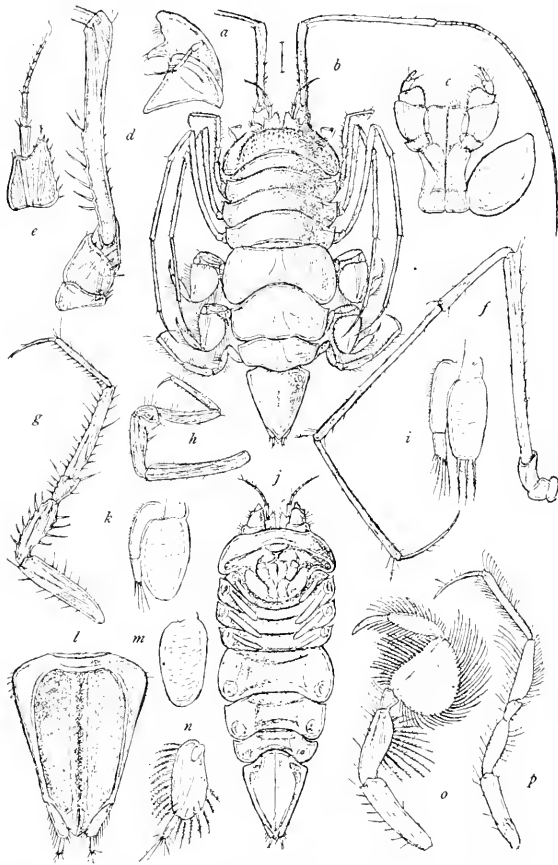
FIG. 549.— ILYARACHNA HIRTIPEIS (AFTER SARS). a , MANDIBLE. b , DORSAL VIEW OF FEMALE. c , MAXILLIPEDS. d , SECOND ANTENNA. e , FIRST ANTENNA. f , SECOND ANTENNA. g , SECOND LEG. h , FIRST LEG. i , THIRD PLEOPOD. j , VENTRAL VIEW OF FEMALE. k , FOURTH PLEOPOD. l , ABDOMEN (VENTRAL VIEW). m , FIFTH PLEOPOD. n , UROPOD. o , FIFTH LEG. p , SEVENTH LEG.
