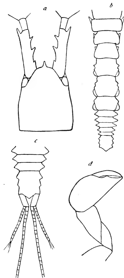
FIG. 37.— APSUEDES PROPINQUUS . a , HEAD. b , SEGMENTS OF THORAX AND ABDOMEN. c , LAST FOUR SEGMENTS OF BODY AND PART OF UROPODA. d , FIRST GNATHOPOD.
