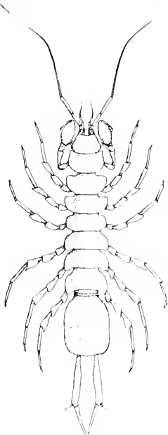
FIG. 190.—CÆCIDOTEA STYGIA (AFTER HAY).
