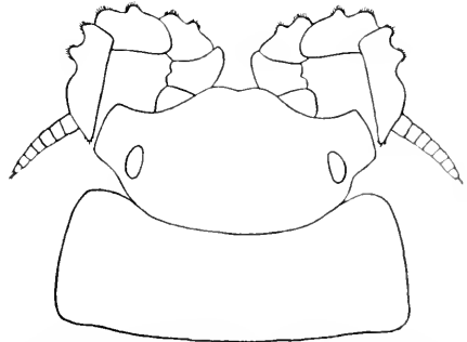
FIG. 731.—TRICHONISCUS PAPILLICORNIS. HEAD AND FIRST THORACIC SEGMENT. \times 11 .
