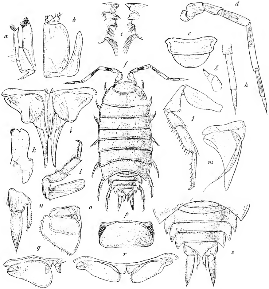
FIG. 674.— METOPONORTHUS PRUINOSUS (AFTER SARRS). a , FIRST MAXILLA. b , MAXILLIPED. c , MANDIBLES. d , SECOND ANTENNA. e , ANTERIOR LIP. f , DORSAL VIEW OF MALE. g , FIRST ANTENNA. h , FLAGELLUM. i , FIRST PLEPOD OF MALE. j , SEVENTH LEG. k , SECOND MAXILLA. l , FIRST LEG. m , SECOND PLEPOD OF MALE. n , UROPOD. o , THIRD PLEPOD OF FEMALE. p , HEAD. q , SECOND PLEPOD OF FEMALE. r , FIRST PLEPODS OF FEMALE. s , ABDOMEN WITH UROPODA.
