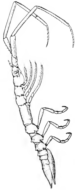
FIG. 369.— ARCTURUS BAFFINI VAR. TUBEROSUS (AFTER BENEDICT). 1/2.
