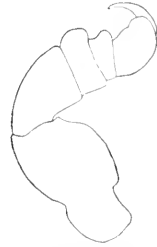
FIG. 258.— INDUSA CARINATA . LEG OF SEVENTH PAIR. · 7.
