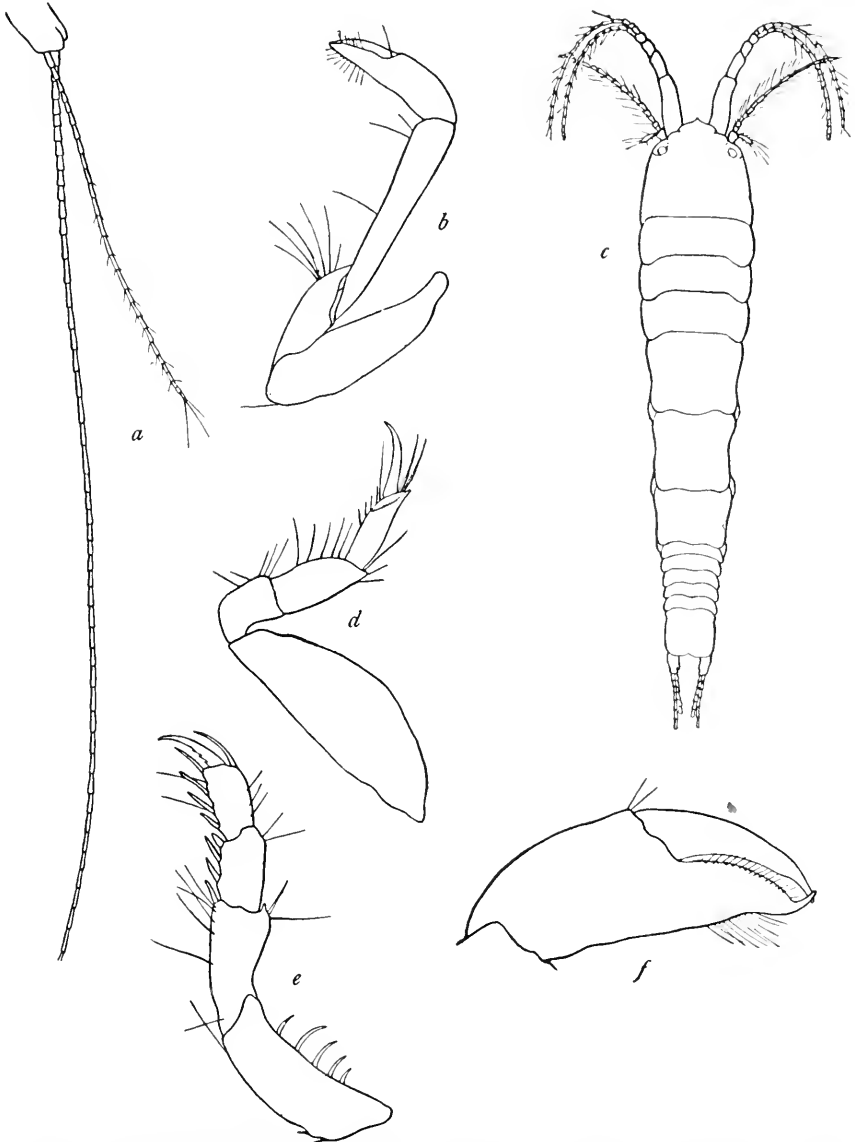
FIG. 34.— APEUDES SPINOSUS (AFTER MOORE). a , UROPOD. b , FIRST LEG. c , GENERAL FIGURE. d , SEVENTH LEG. e , SECOND LEG. f , CHELA. (ALL ENLARGED.)
