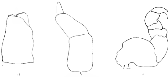
FIG. 244.— MEINERTIA GAUDICHAUDI . a , SECOND MAXILLA. 33. b , PALE OF MANDIBLE. 33. c , LEG OF SEVENTH PAIR. 33.
