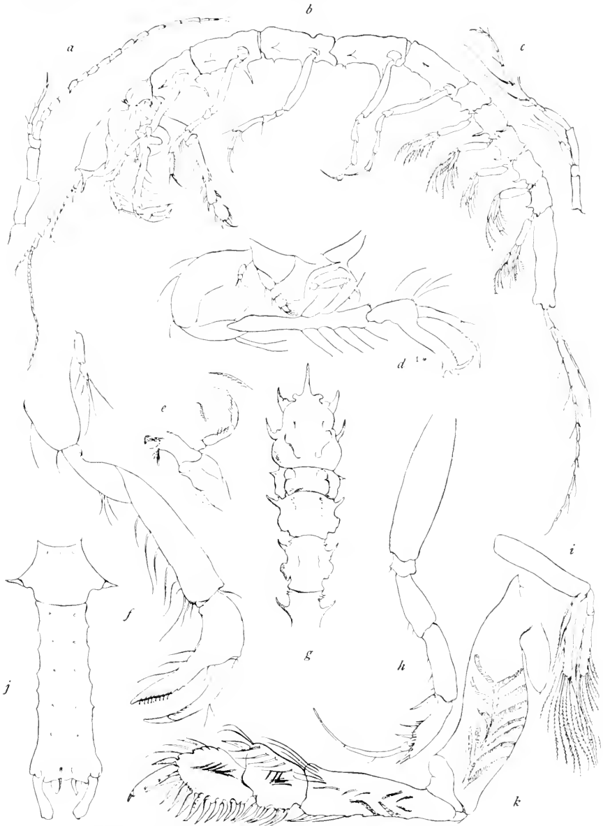
FIG. 35.—APSEUDES GRACILIS (AFTER NORMAN AND STERRING). a , UPPER ANTENNA. b , LATERAL VIEW. c , LOWER ANTENNA. d , SIDE VIEW OF MOUTH PARTS AND AN ABNORMALLY DEVELOPED FIRST GNATHOPOD. e , MANDIBLE. f , FIRST GNATHOPOD. g , ANTERIOR PART OF BODY, FROM ABOVE. h , FIFTH LEG. i , PLEOPOD. j , LAST SEGMENT OF ABDOMEN. k , SECOND GNATHOPOD.
