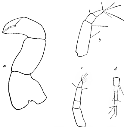
FIG. 28.—LEPTOCHELIA SAVIGNYI. FEMALE. a , FIRST LEG. b , FIRST ANTENNA. c , SECOND ANTENNA. d , UROPOD. \times 77\frac{1}{2} .
