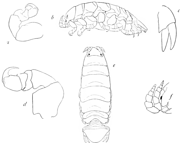
FIG. 216.—MEINERTIA DEPLANATA (AFTER BOVALLIUS). a , FIRST LEG. b , LATERAL VIEW OF FEMALE. c , UROPOD. d , SEVENTH LEG. e , DORSAL VIEW OF FEMALE. f , HEAD WITH BOTH ANTENNAE. (ENLARGED.)
