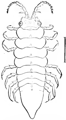
FIG. 429.—SYNIDOTEA NODULOSA (AFTER HARGER). X 4.
