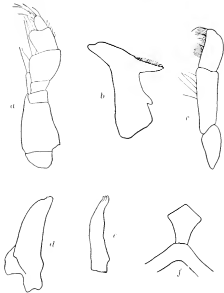
FIG. 145.—TRIDENTELLA VIRGINIANA. a , MAXILLIPED. \times 51\frac{1}{2} . b , MANDIBLE. \times 51\frac{1}{2} . c , PALP OF MANDIBLE. \times 51\frac{1}{2} . d , SECOND MAXILLA. e , FIRST MAXILLA (OUTER LOBE). \times 51\frac{1}{2} . f , FRONTAL LAMINA. \times 27\frac{1}{2} .
