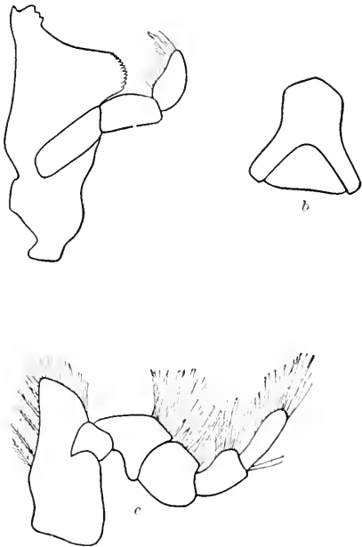
FIG. 293.—SPHÆROMA QUADRIDENTATUM. a , MANDIBLE. \times 41 . b , FRONTAL LAMINA AND CLYPEUS. \times 23 . c , MAXILLIPED. \times 11 .
