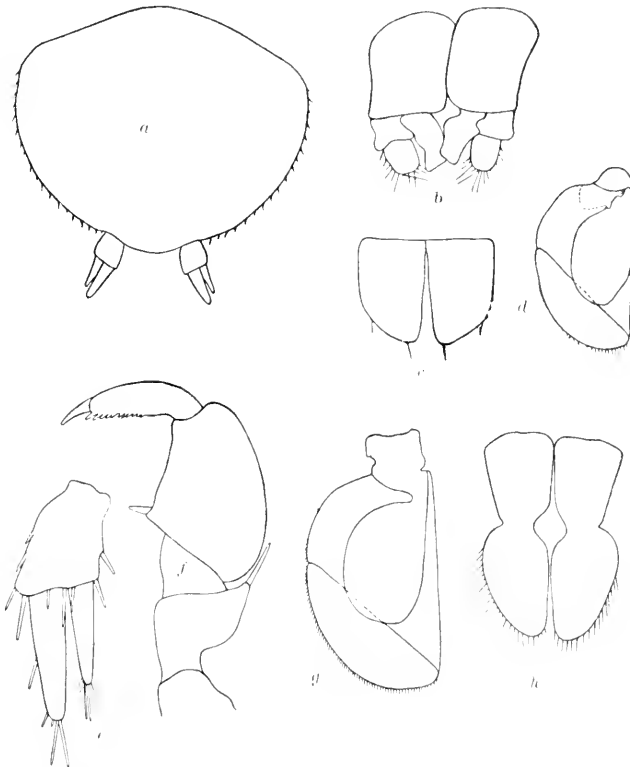
FIG. 460.—MANCASELLUS BRACHYURUS. a , ABDOMEN WITH UROPODA. — 9½. b , SECOND PLEOPOD OF MALE. — 27½. c , FIRST PLEOPOD OF FEMALE. — 27½. d , THIRD PLEOPOD OF MALE. — 15½. e , UROPOD. — 27½. f , FIRST LEG. — 27½. g , THIRD PLEOPOD OF FEMALE. — 15½. h , FIRST PLEOPOD OF MALE. — 27½.
