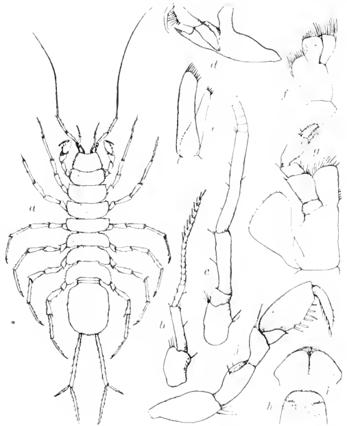
FIG. 185.—CÆCIDOTEA RICHARDSONÆ (AFTER HAY). a, DORSAL VIEW. b, FIRST ANTENNA. c, SECOND ANTENNA. d, MANDIBLE. e, FIRST MAXILLA. f, SECOND MAXILLA. g, MAXILLIPED. h, UPPER LIP. i, LOWER LIP. j, GNATHOPOD.
