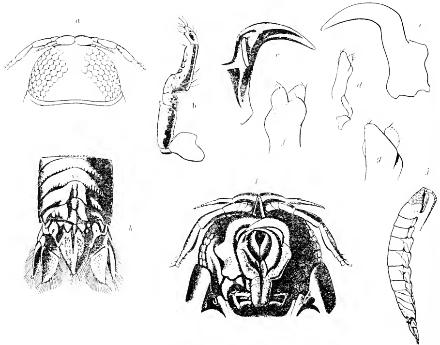
FIG. 131.—EXOCORALLANA ANTILLENSIS (AFTER HANSEN). a , HEAD OF ADULT MALE. \times 11 (FROM ABOVE). b , LEFT MAXILLIPED OF SAME. \times 21 . c , LEFT MANDIBLE, PALP OMITTED (VENTRAL SIDE). \times 21 . d , LEFT MAXILLA (SECOND PAIR). \times 24 . e , LEFT MANDIBLE (BASAL PART OMITTED). \times 24 (FROM ABOVE). f , DISTAL PART OF LEFT MAXILLA OF SECOND PAIR (VENTRAL SIDE). \times 59 . g , DISTAL PART OF SAME (FROM ABOVE). \times 6 . h , ABDOMEN. \times 6 . i , HEAD (VENTRAL SIDE). \times 11 . j , ADULT MALE (LATERAL VIEW). \times 11 .
