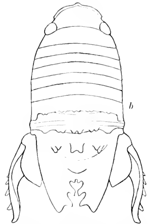
FIG. 336.—CILICEA CORDATA (MALE). a, HEAD AND FIRST THORACIC SEGMENT. b, DORSAL VIEW. . 8.
