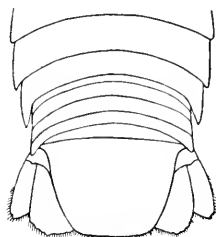
FIG. 88.— CIOROLANA OBTRUNCATA . ABDOMEN AND LAST TWO THORACIC SEGMENTS.
