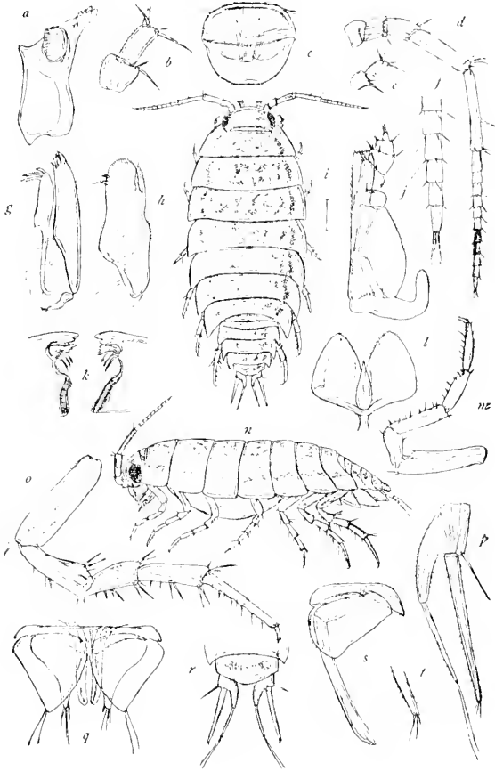
FIG. 730.— LIGIDIUM HYPNORUM (AFTER SAUS). a , MANDIBLE. b , FIRST ANTENNA. c , ANTERIOR LIP. d , SECOND ANTENNA. e , FIRST ANTENNA. f , FLAGELLUM OF SECOND ANTENNA. g , FIRST MAXILLA. h , SECOND MAXILLA. i , DORSAL VIEW OF FEMALE. j , MAXILLIPED. k , MANDIBLES. l , POSTERIOR LIP. m , FIRST LEG. n , LATERAL VIEW OF FEMALE. o , SEVENTH LEG. p , UROPOD. q , FIRST PLEOPOD OF FEMALE. r , LAST SEGMENT OF ABDOMEN AND UROPODA. s , SECOND PLEOPOD OF MALE. t , EXTREMITY OF OUTER BRANCH OF UROPOD.
