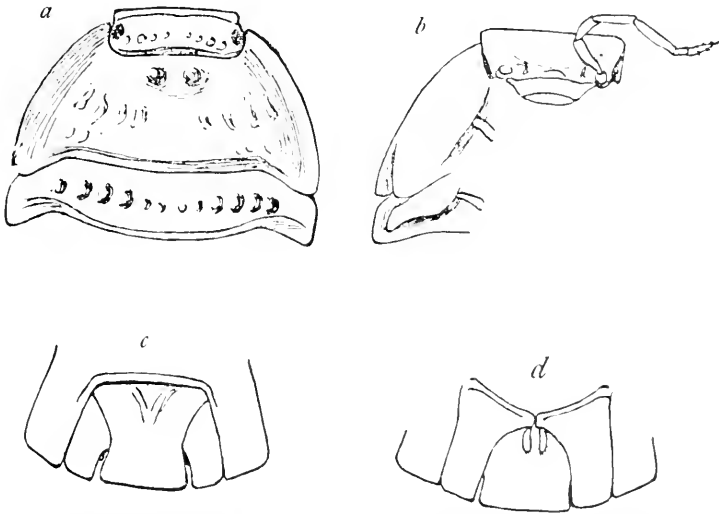
FIG. 600.— CUBARIS CINCTA (AFTER DOLLEUS). a , HEAD AND FIRST TWO SEGMENTS OF THORAX (UPPER SIDE). b , THE SAME (UNDERSIDE). c , FIFTH AND SIXTH SEGMENTS OF ABDOMEN AND UROPODA (UPPER SIDE). d , THE SAME (UNDERSIDE).
