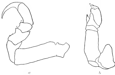
FIG. 166.— ÆGA ARCTICA . a , LEG OF SECOND PAIR. · 27 \frac{1}{2} . b , MAXILLIPED. · 15 \frac{1}{2} .
