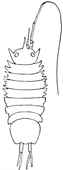
FIG. 518.—IOLELLA LIBBEYI (AFTER ORTMANN). 6.
