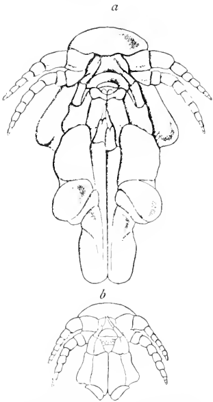
FIG. 233.—OLENOCRA PEREGUSTATOR (AFTER SCHLEDTE AND MEINERT). a , HEAD OF FEMALE SHOWING ANTENNAE AND MOUTH PARTS. b , HEAD OF MALE SHOWING SAME. (ENLARGED.)
