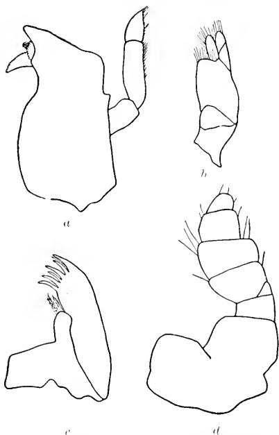
FIG. 89.— CIOROLANA OBTRUNCATA . a , MANDIBLE. b , SECOND MAXILLA. c , FIRST MAXILLA. d , MAXILLIPED. ALL \times 51\frac{1}{2} .
