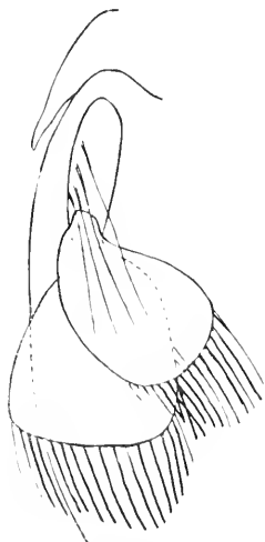
FIG. 111.—BRANCHIOPUS LITTORALIS. (AFTER MOORE). UROPODA FROM BELOW.
