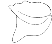
FIG. 603.—PROBOPYRUS FLORIDENSIS. FIRST LAMELLA OF MARSUPIUM. \times 10 .
