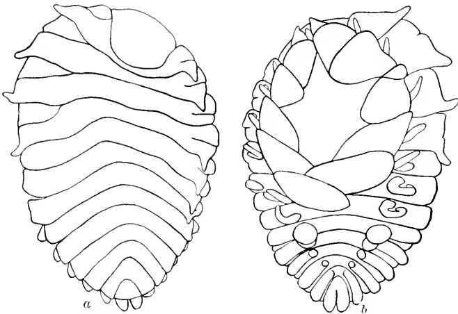
FIG. 596.— ARGELIA PUGETTENSIS . a , DORSAL VIEW OF IMMATURE FEMALE. b , VENTRAL VIEW OF SAME. \cdot 14\frac{1}{2} . (SECOND POST-LARVAL STAGE.)
