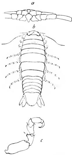
FIG. 160.— Ega tenuipes (AFTER SCHIEDETE AND MEINERT). a , FRONTAL MARGIN WITH ANTENNAE AND FRONTAL LAMINA. b , YOUNG FEMALE. c , RIGHT LEG OF SECOND PAIR. (ALL ENLARGED.)
