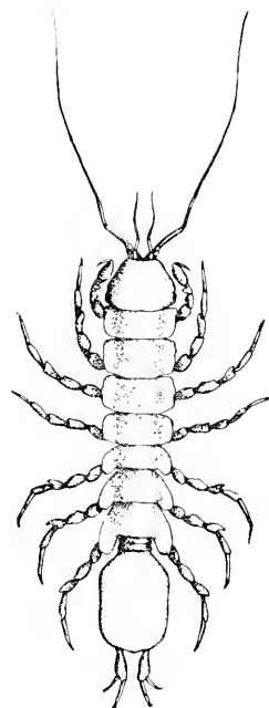
FIG. 393.—CÆCIDOTEA NICKAJACKENSIS (ALTER HAY). METCALF, GEORGIA, SPECIMEN.
