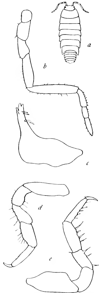
FIG. 600.—PHILOSCLIA CULEBRÆ (AFTER MOORE). a, DORSAL VIEW. b, SECOND ANTENNA. c, MANDIBLE. d, FIRST LEG.
