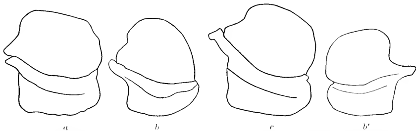
FIG. 630.— BOPYROIDES HIPPOLYTES . FIRST LAMELLA OF MARSUPIUM FROM SPECIMENS FOUND ON: a , SPIRONTOCARIS SPINUS FROM EASTPORT, MAINE. \times 14\frac{1}{2} . b , SPIRONTOCARIS SPINUS FROM BAY OF ISLANDS, ADAKH, ALASKA. \times 23 . c , SPIRONTOCARIS SECURIFRONS FROM THE HAWAIIAN ISLANDS. b' , SPIRONTOCARIS SPINUS FROM BAY OF ISLANDS, ADAKH, ALASKA. \times 23 .
