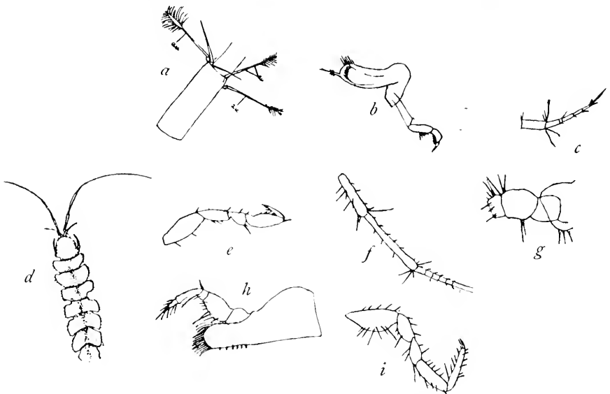
FIG. 10.—CÆCIDOTEA SMITHSII (AFTER ULRICH). a , BASAL SEGMENT OF UPPER ANTENNA, SHOWING AUDITORY SPINES. b , MAXILLA (?) ACCORDING TO ULRICH. c , UPPER ANTENNA. d , PORTION OF BODY. e , FIRST LEG. f , PORTION OF LOWER ANTENNA. g , BASAL PORTION OF SAME. h , LABRUM. i , SECOND LEG.
