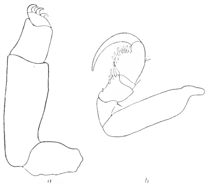
FIG. 202.— ROCINELA LATICAUDA . a , MAXILLIPED. \cdot 27\frac{1}{2} . b , LEG OF SECOND PAIR. \cdot 9\frac{1}{2} .
