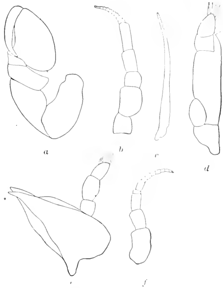
FIG. 57.— CALATHURA BRANCHIATA . a, FIRST LEG. \times 11\frac{1}{2} . b, SECOND ANTENNA. \times 20 . c, FIRST MAXILLA. \times 39 . d, MAXILLIPED. \times 39 . e, MANDIBLE. \times 39 . f, FIRST ANTENNA. \times 20 .
