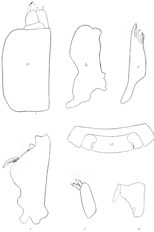
FIG. 689.— CUBARIS MURINA . a, MAXILLIPED. 514. b, SECOND MAXILLA. 514. c, FIRST MAXILLA (OUTER LOBE). 514. d, TERMINAL SEGMENT WITH UROPODA. 153. e, MANDIBLE. 514. f, FIRST MAXILLA (INNER LOBE). 514. g, UROPOD. 271. (FROM UNDERSIDE.)
