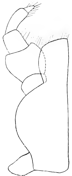
FIG. 470.—MANCASELLUS DANIELSI, MAXILLIPED. (GREATLY ENLARGED.)
