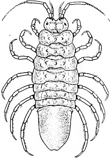
FIG. 412.— SYNIDOTEA PALLIDA (AFTER BENEDICT). \times 21 .
