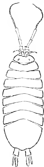
FIG. 180.—ASELLUS HOPPINÆ (AFTER FAXON). (— 4).
