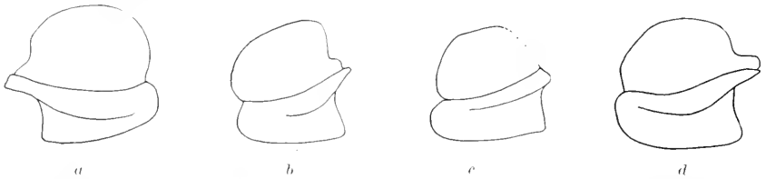
FIG. 592.— ARGELIA PUGETTENSIS . FIRST INCUBATORY PLATE FROM SPECIMENS FOUND ON: a , NECTOCRANGON CRASSA FROM OFF CAPE NEWENHAM, ALASKA. · 9½. b , NECTOCRANGON CRASSA FROM ALASKA. 9½. c , CRAGO NIGROMACULATA FROM SAN DIEGO BAY, CALIFORNIA. · 9½. d , CRAGO NIGRICAUDA FROM OFF CAPE JOHNSON. · 9½.
