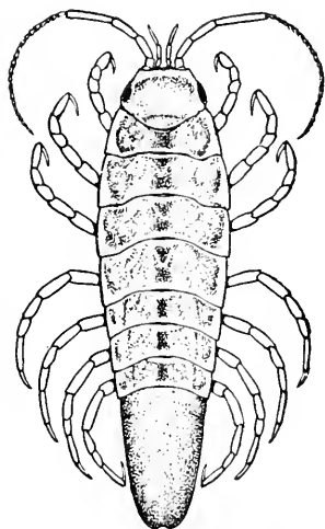
FIG. 127.—SYNIDOTEA HARFORDI (AFTER BENEDICT). \times 3\frac{1}{2} .
