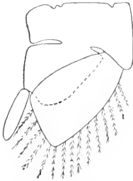
FIG. 338.— CILICEA CORDATA . SECOND PLEPOD OF MALE. - 153.
