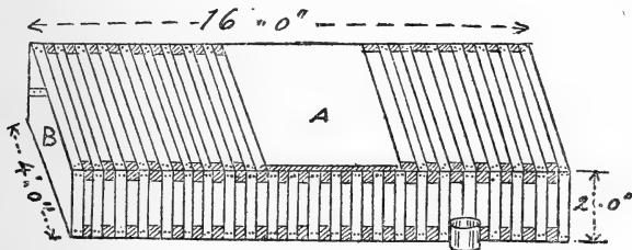
MOVABLE POULTRY YARD. FIG. 50.
