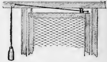
GATE DEVICE. FIG. 34.
