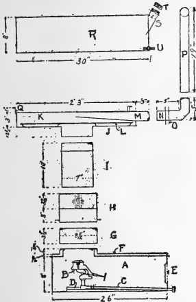
FIG. 10.—Section plan of the parts of the gasoline heater
