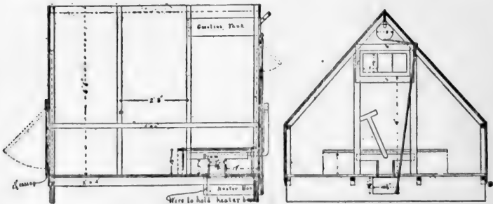
SIDE VIEW BROODER-HOUSE. FIG. 8. SECTIONAL VIEW. FIG. 9.
