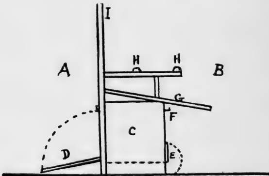
INSIDE HOUSE ARRANGEMENT. FIG. 47.
