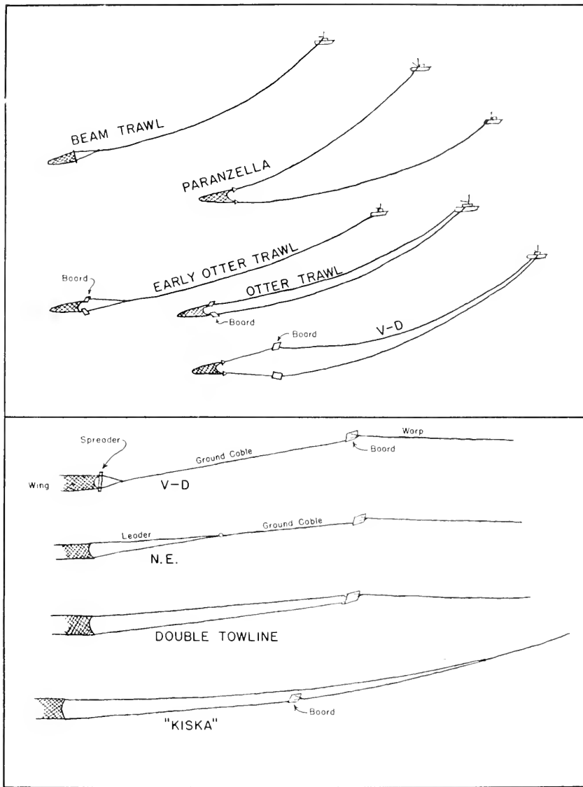
FIGURE 152. Sketch to show beam and paranzello trawls, two forms of early otter trawls, and the improved V-D type. Lower half of the figure illustrates four methods of placing the otter board in advance of the net wing. Drawing by the author.
