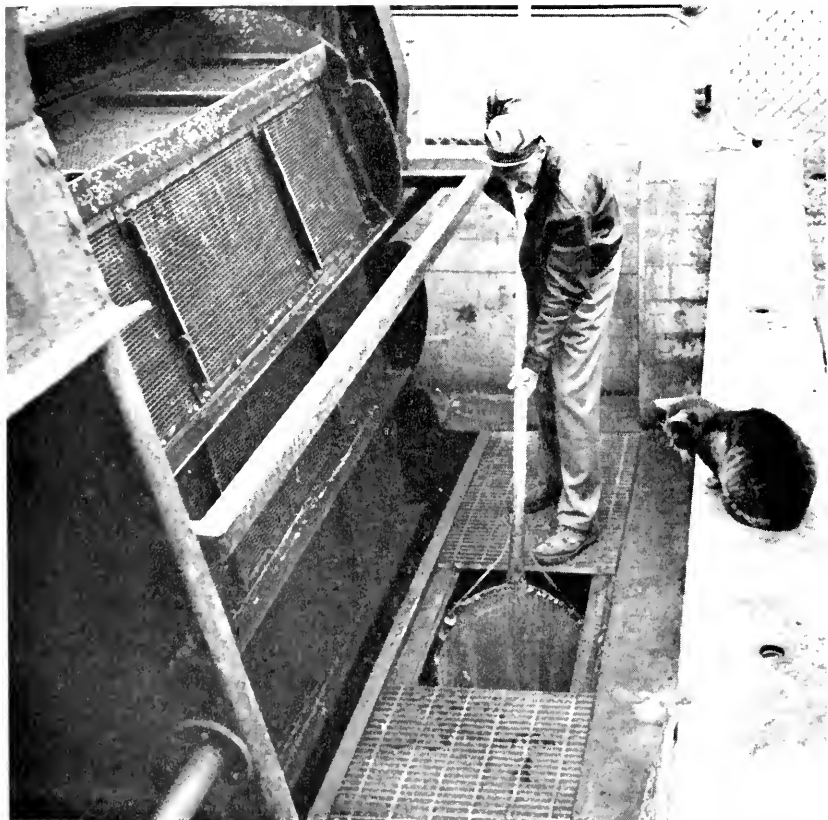
FIGURE 2. The junior author hauling up the collecting net from the sump in front of the revolving trash screen. Photograph by Toshia Asaeda, November, 1954.
