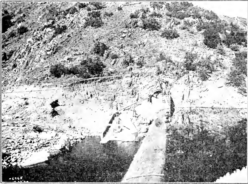
FIG. 28. Newly built fishway built by Southern California Gas & Coal Co. at Kern River plant No. 3. Built according to plans furnished by the Fish and Game Commission.
