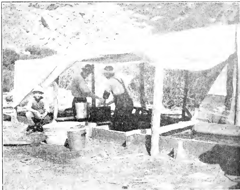
FIG. 7. Spawning rainbow trout at the Rae Lakes Egg-collecting Station.
