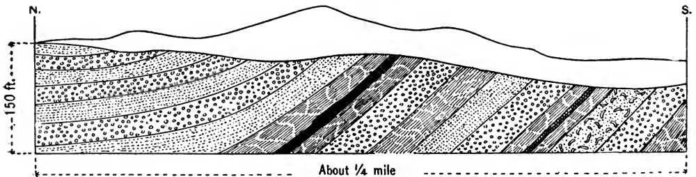
Fig. 8.—Northern slope of anticline cut by railroad two miles northwest of Bradley. The thin seam of lignite has gypsum mixed with it. The fossils are limpets, turritellas, and various clam and oyster shells.
