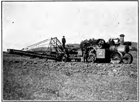
STREET GRADING OUTFIT IN OPERATION AT NEWARK
