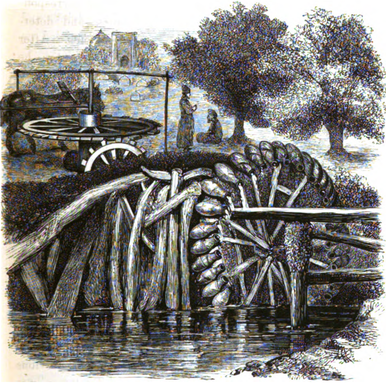
IRRIGATION WHEEL.
