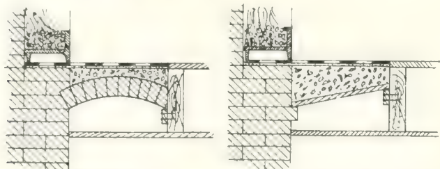
Fig. 1. With Brick Arch. Fig. 2. Without Brick Arch: Section Showing Foundations of Brick Tiling
