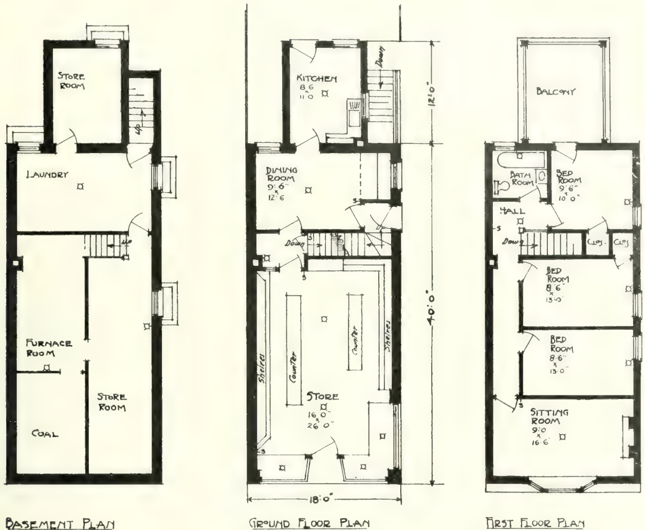
BASEMENT PLAN
