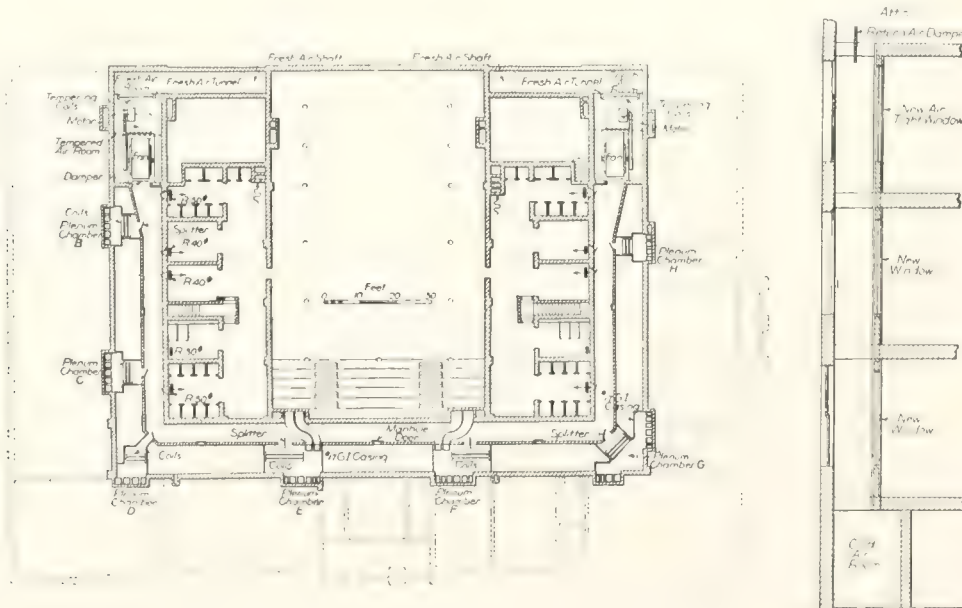
Basement Plan of New Building showing Heating and Ventilating Scheme
