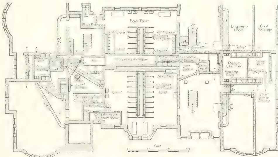
Remodeled Scheme of Heating and Ventilating in Old High School Building
