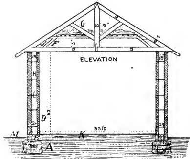
FIG. 1309.—ICE-HOUSE.
