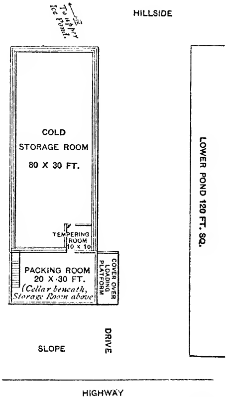
FIG. 1270.—GROUND PLAN OF HOUSE, WITH SURROUNDINGS.
