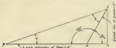
Fig. 4.—Calculating Gears, Shafts Acute.
