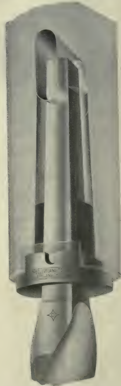
Fig. 2.—Shank, Collet and Spindle in Combination.
