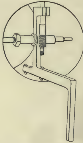
Fig. 4.—Caliper Adjusted to Wheel.
