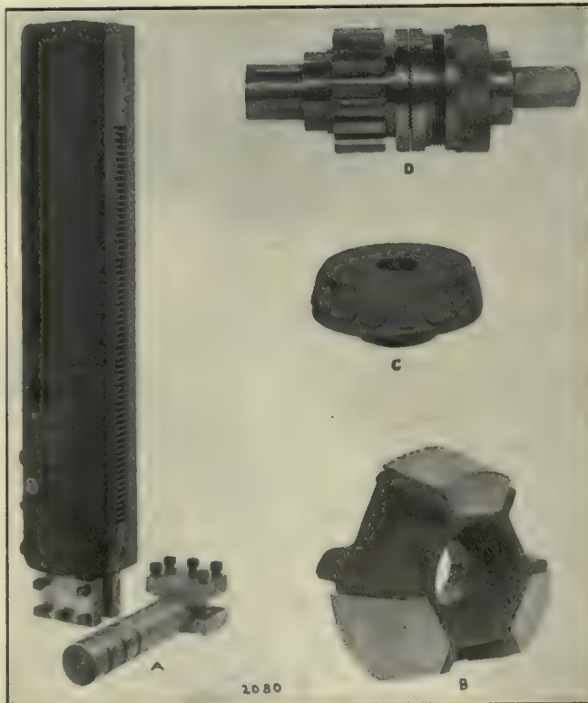
Fig. 3.—Details of New Model Boring and Turning Mills, Colburr Machine Tool Co.
