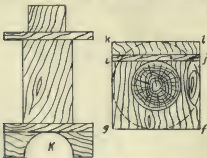
Fig. 3 d.—Pipe Patterns.
