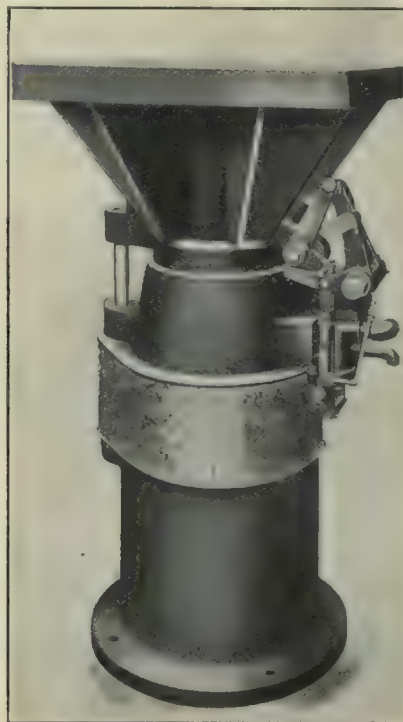
Fig.1.—Tabor Shockless Jarring Machine.
