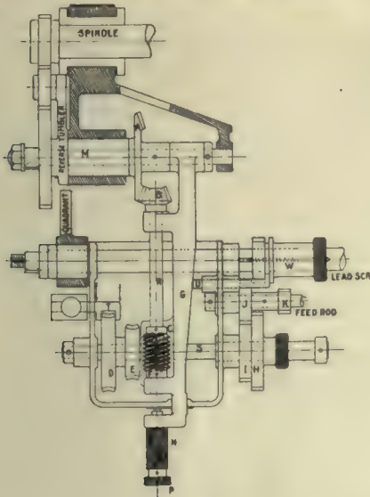
Fig. 2.—Diagram of Positive Feed.
