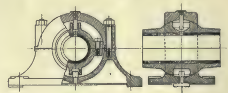
Fig. 2.—Bearing for Hardinge Conic Mill.
