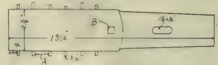
Fig. 3.—Multiple Tool.
