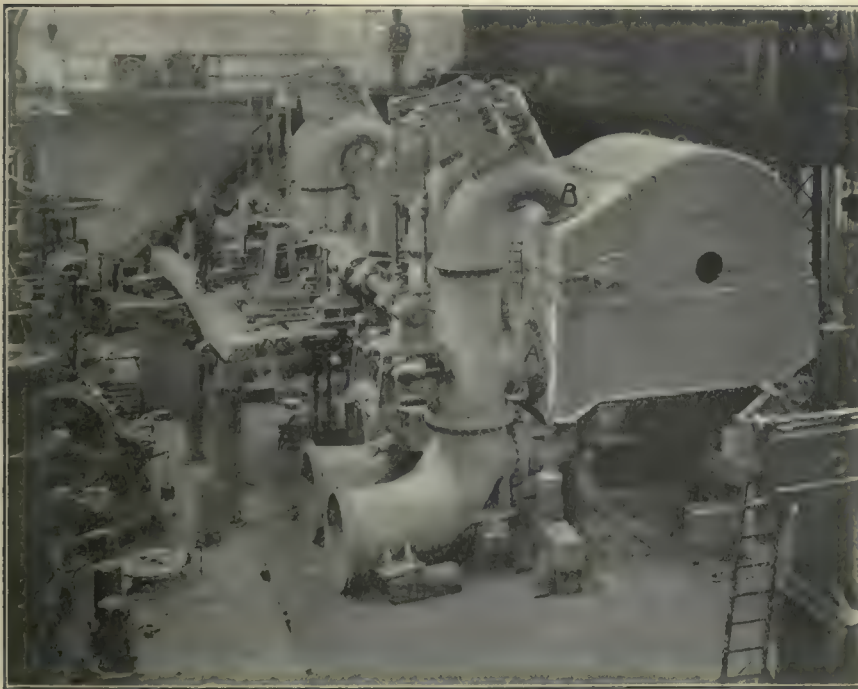
A 10,500 h.p. Impulse Water Wheel.
