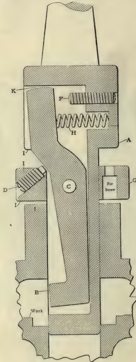
An Inside Facing Tool.
