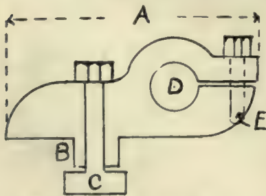
End View, Boring Bar Holder.
