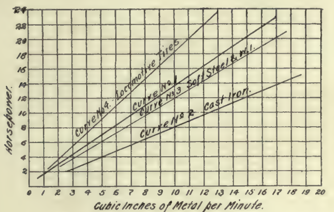
CHART OF HORSE-POWER REQUIRED TO REMOVE METAL
