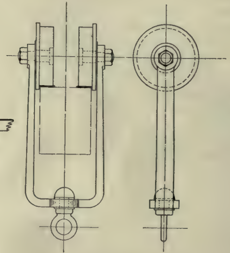
Fig. 2.—Runner Complete.
