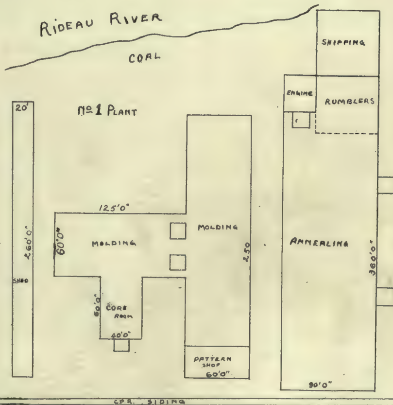
Plant No. 1.—Smith's Falls Malleable Castings Co.
