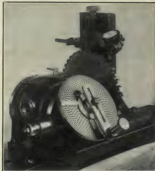
Fig. 5.—Testing Accuracy of Worm Teeth.
