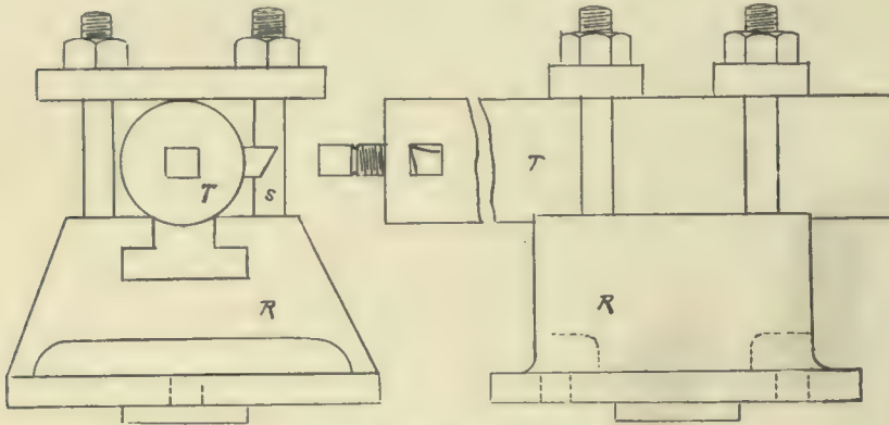
Fig. 1.—Arrangement of Tool.
