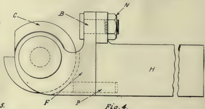
Thread Cutting Tool.
