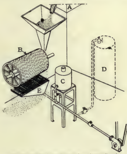
Apparatus Used in Preparing Core Sand.
