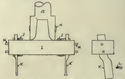
Fig. 4.—Boring or Ripping Tool for Crank Webs.
