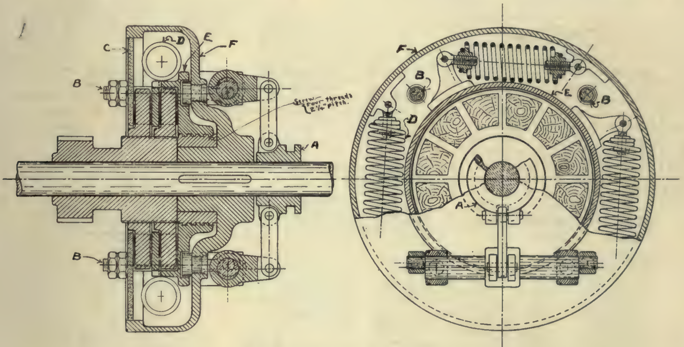
Automatic Relieving Friction Clutch.
