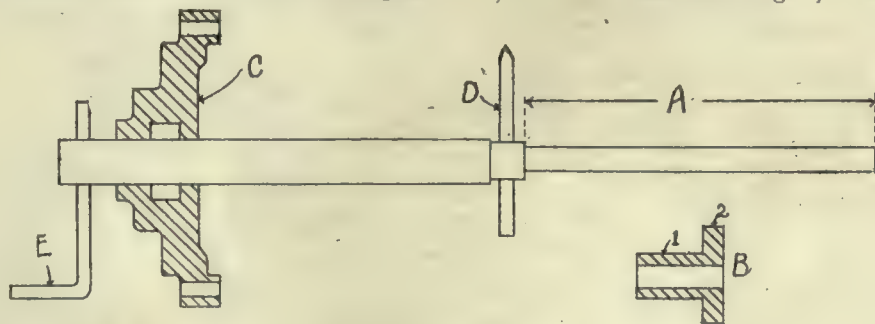
Cylinder Boring Bar.
