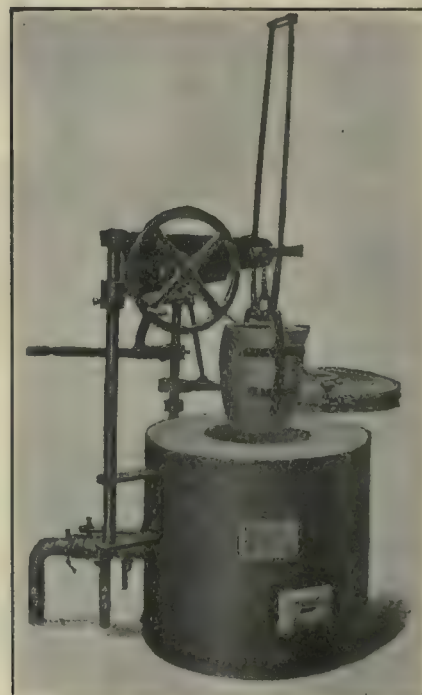
Fig. 2.—Crucible Raised and in Position to be Lowered Into Pot.
