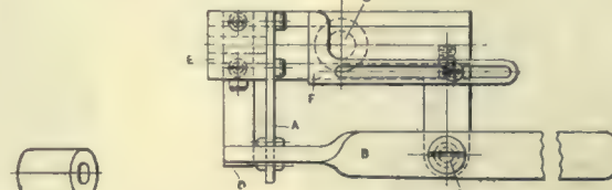
CUTTING-OFF TOOL.—FIG. 3.
