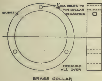
BRASS COLLAR
