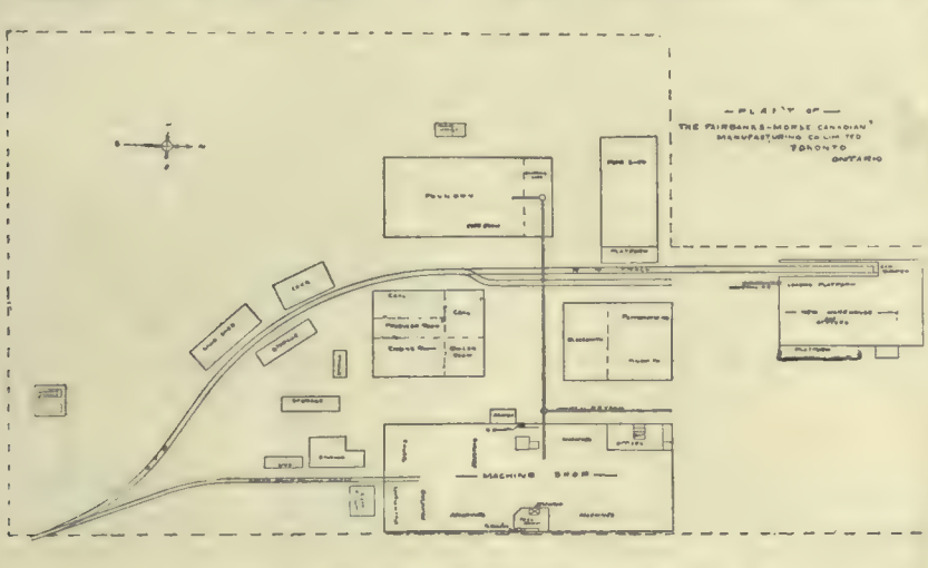
Layout of the Fairbanks-Morse Toronto Plant.
