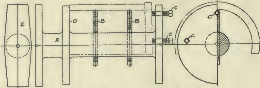
Fig. 8.—Jig for Turning Locomotive Brasses.
