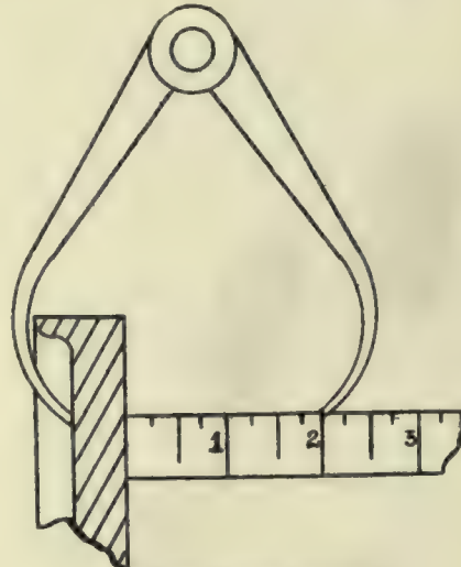
Calipering Flange Casting.
