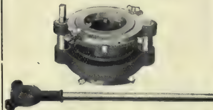
No. 60, cuts 2 1/2, 3, 3 1/2, 4, 4 1/2, 5, and 6 inch pipe
