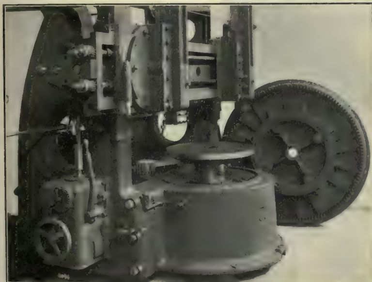
Fig. 1.—Detail of Table Spindle Bearing and Internal Drive as Used on 60 and 72 Inch New Model Mills.
