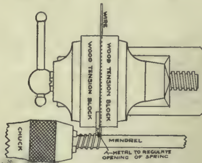
How to Wind an Open Spring.
