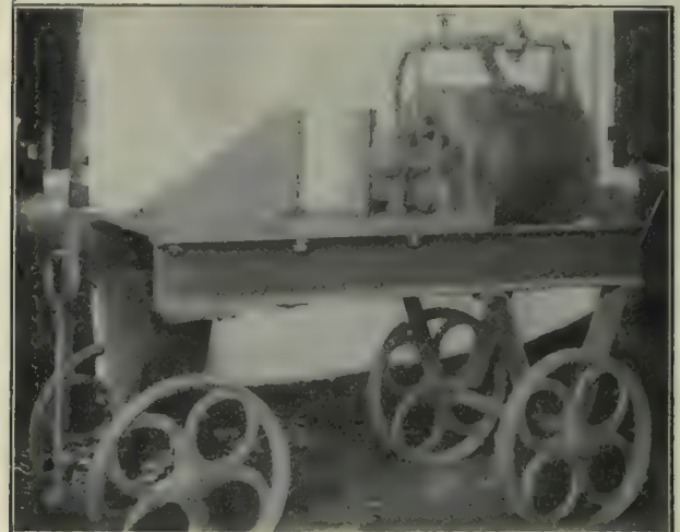
Fig. 10.—Portable Bulldozer.
