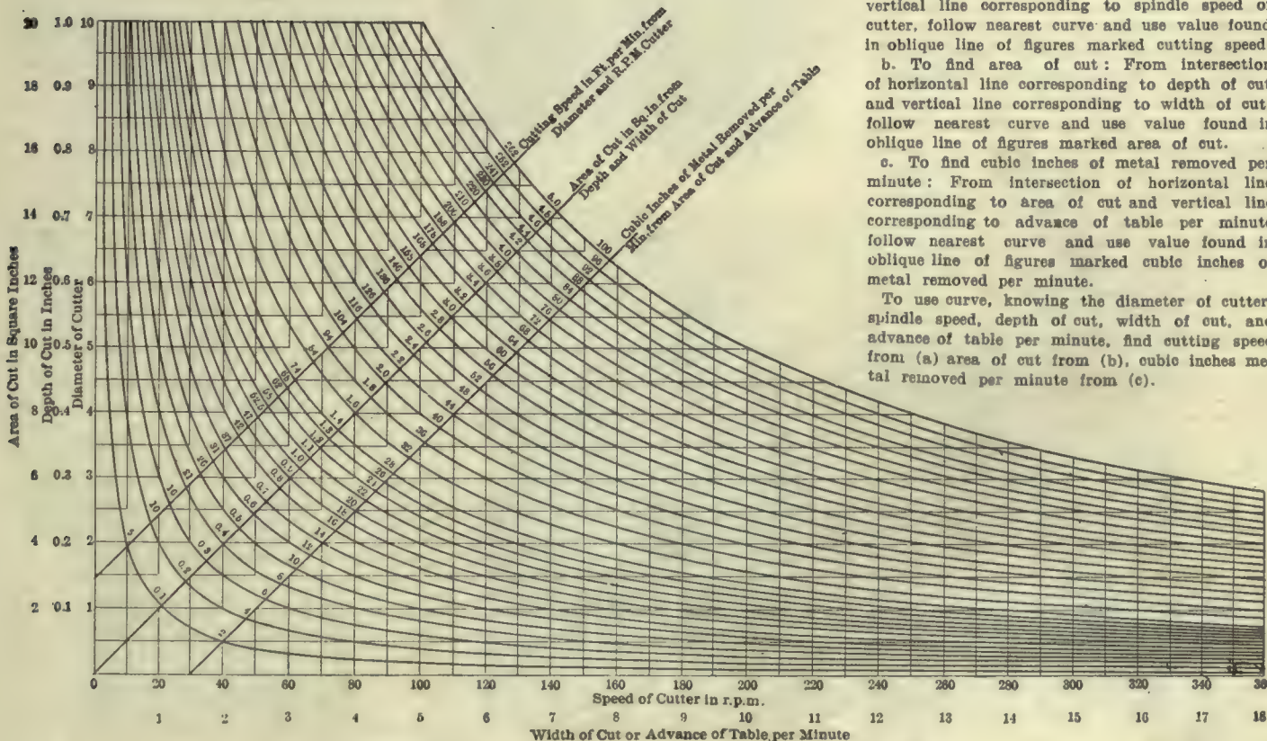
PLATE 3 MACHINE TOOL CALCULATOR FOR MILLING MACHINES
