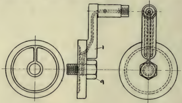
A Fine Piece of Cold Press Work.
