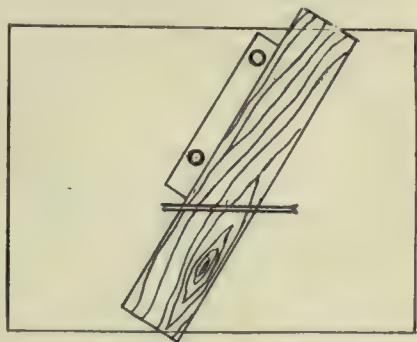
Fig. 1 i.—Pipe Patterns.
