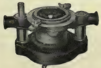
No. 41, cuts 2½, 3, 3½ and 4 in. pipe.
