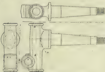
Automobile Steering Knuckle.
