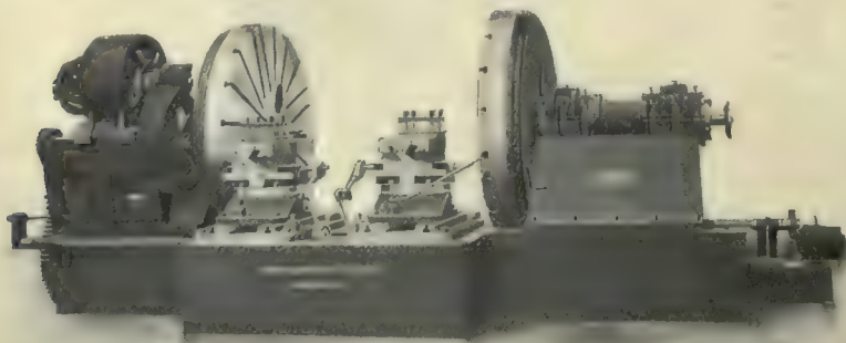
Fig. 15.—Heavy Wheel Lathe.
