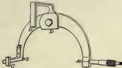
Fig. 1.—Caliper for Wheel Slats.
