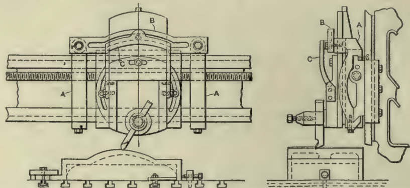
Planer Attachment Which Automatically Guides Tool in Planing Curved Surfaces.
