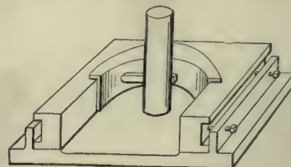
Fig. 1.—Boring Driving Boxes.
