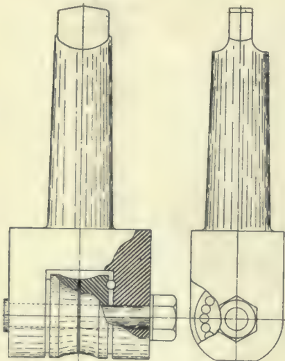
Fig. 2.—Heading Tool.
