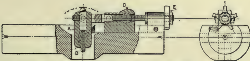
Compact Design of Spherical Boring Attachment for Lathe.
