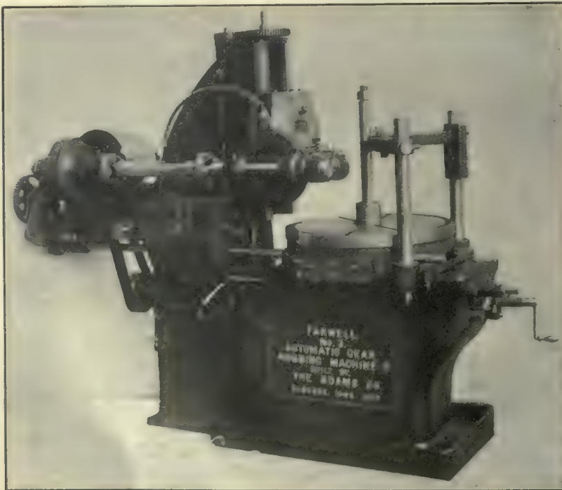
Farwell Gear Hobber.
