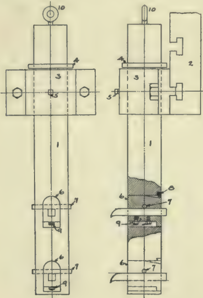
Slotting Bar.
