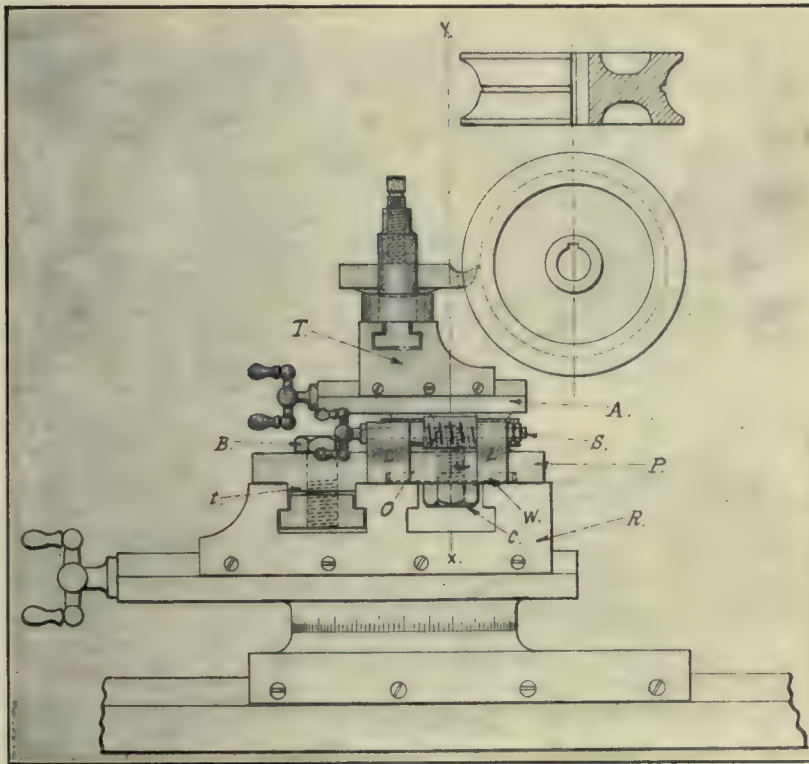
Turning Semi-Circular Grooves.
