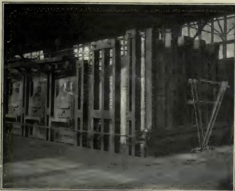
The Kirkwood Oil Fuel System as Applied to Open Hearth Furnaces.
