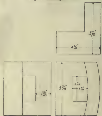
Fig. 4.—Chuck Extension.
