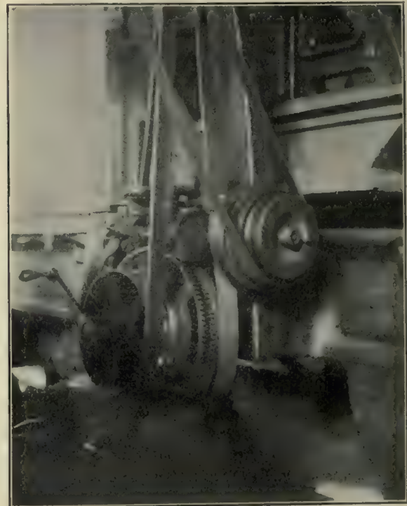
Fig. 2.—Driving Mechanism of Milling Machine and Planer.
