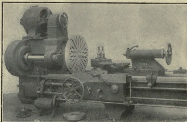
Fig. 4.—Bertram Interchangeable Lathe Fitted for Motor Drive.
