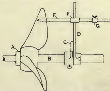
Practical Method of Obtaining Pitch of Propeller.
