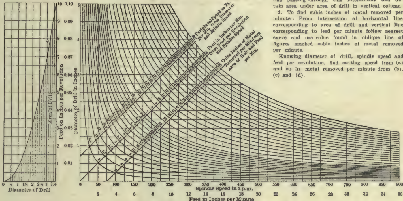
PLATE 2 MACHINE TOOL CALCULATOR FOR DRILLS
