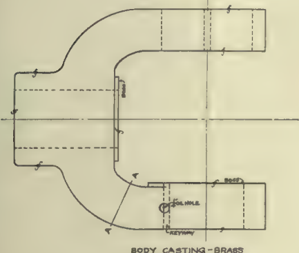
Fig. 5.—Right Angle Drilling Attachment.
