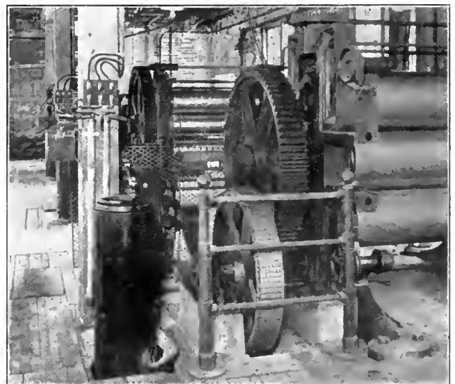
FIG. 4. SILENT CHAIN TRANSMISSION OF LARGE POWERS.
