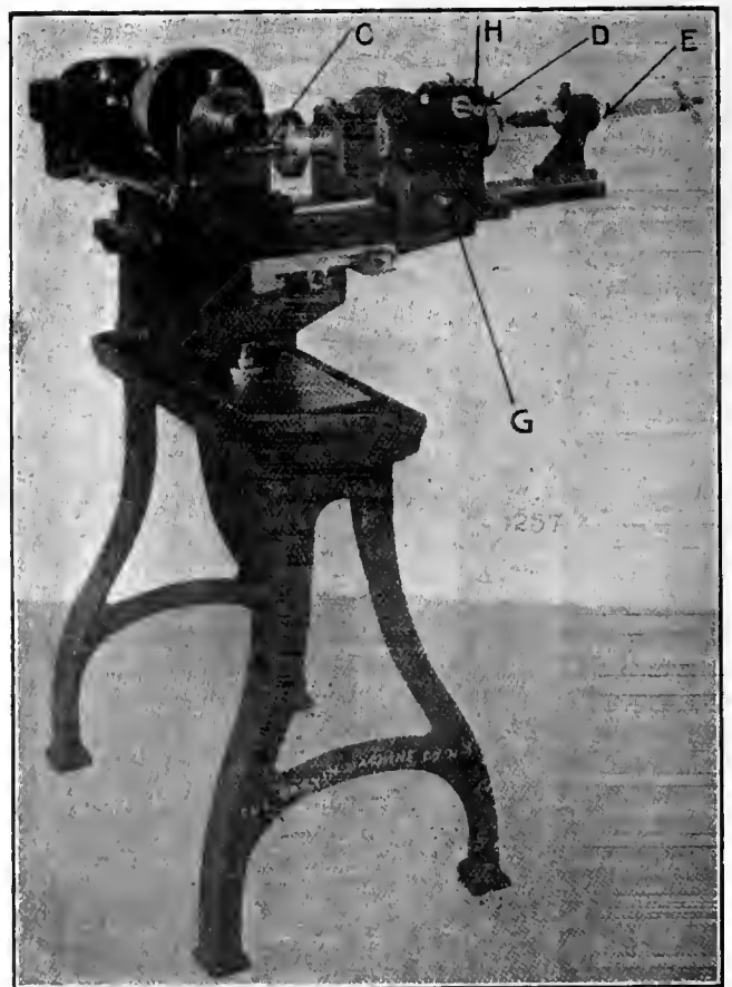
FIG. 2. 6-INCH CAM CUTTING MACHINE.
