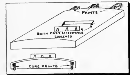
Fig. 3. The Value of Skeleton Patterns.
