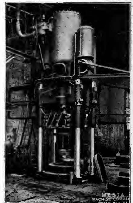
FIG. 4. MESTA-HANIEL & LUEG BENDING PRESS FOR BOILER HEADS AND FLANGING WORK.
