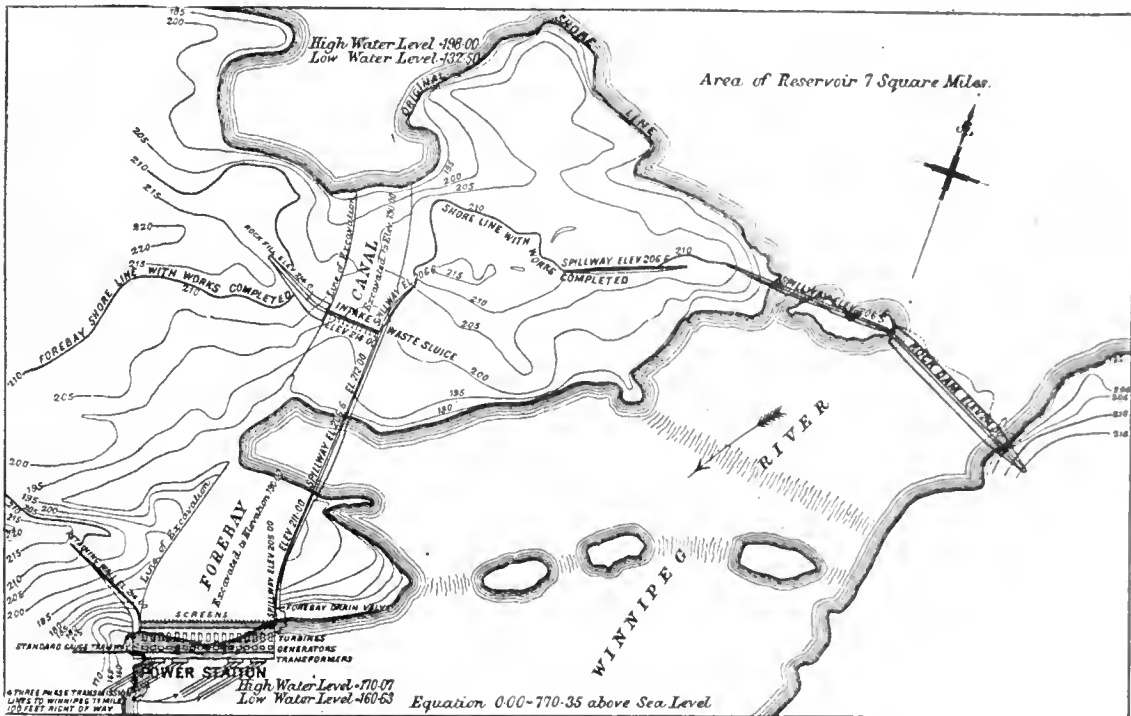
FIG. 1. PLAN OF WORKS AND POINT DU BOIS FALLS.
