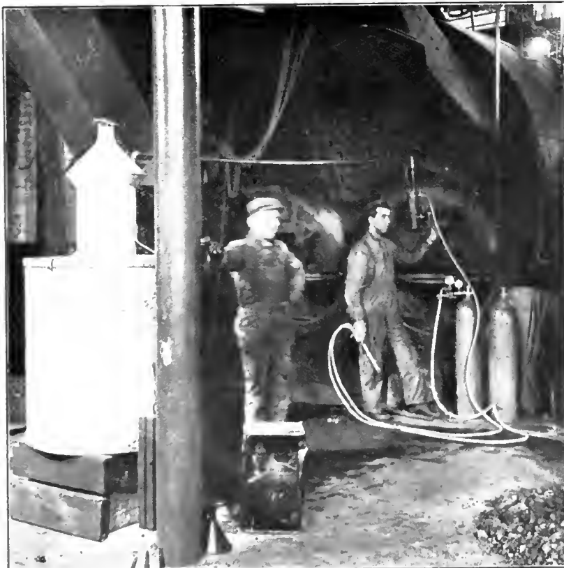
FIG. 3. PREPARING TO REPAIR A BOILER FRACTURE.
