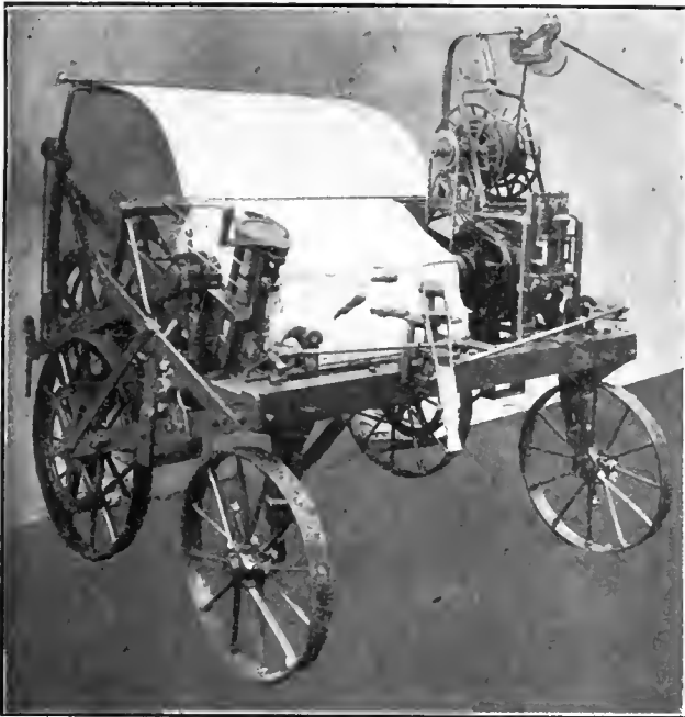
FIG. 1. FRONT VIEW OF SAND MIXING MACHINE.
