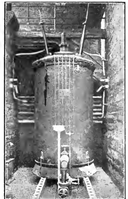
FIG. 27. 3,000 K.W. OIL-IMMERSED WATER-COOLED MAIN TRANSFORMER
