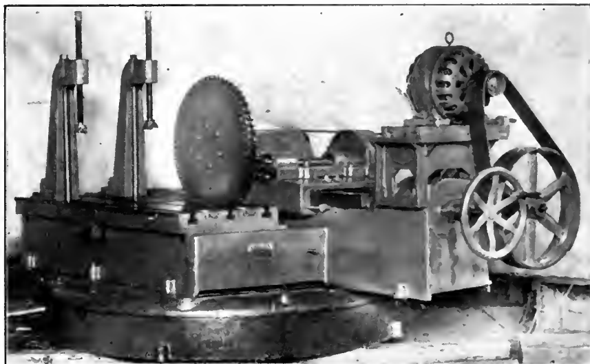
B COMBINATION SAW AND ROTARY PLANER.
