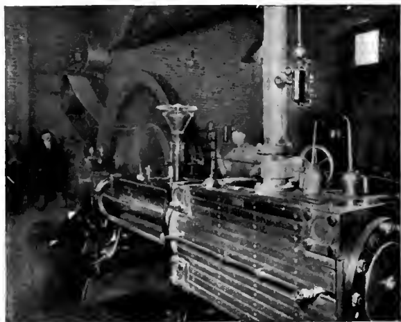
FIG. 3. TYPICAL EXAMPLE OF BELT DRIVE UNDER NON-SLIP TREATMENT.
