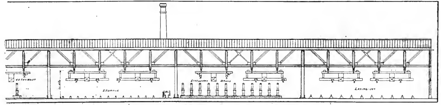
LONGITUDINAL SECTION THROUGH CENTRE OF SHOP.
