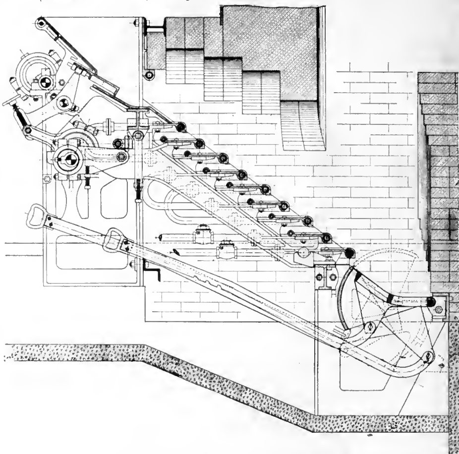
LONGITUDINAL SECTION OF FULTON STOKER.
