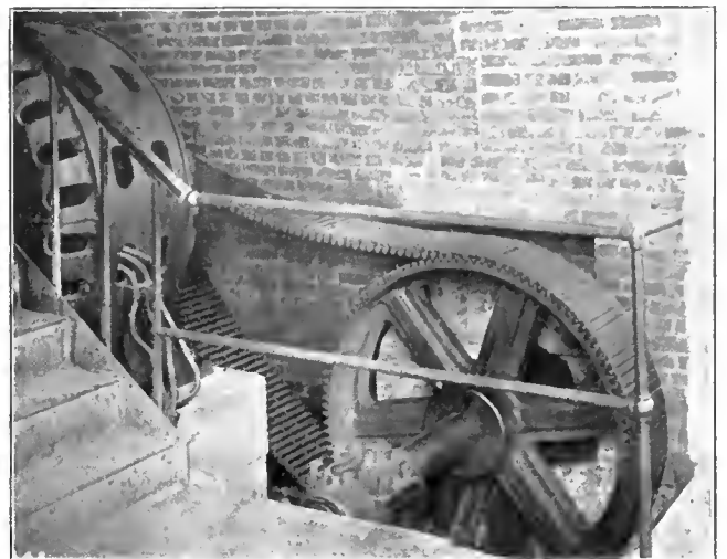
FIG. 2. SILENT CHAIN TRANSMISSION OF LARGE POWERS.
