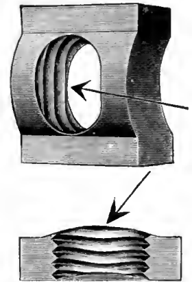
THIS CUT SHOWS AN EXAGGERATED CURVE IN THREAD PITCH—OR MORE THAN IS GIVEN IN PRACTICE, IN ORDER TO EMPHASIZE THIS FEATURE.
