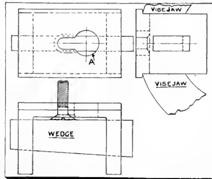
FIG. 3. FILING FIXTURES.
