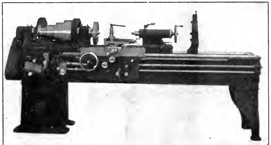
CINCINNATI QUICK CHANGE GEAR ENGINE LATHE WITH 3-STEP CONE AND DOUBLE BACK GEARS.
