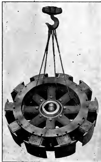
PROPER METHOD OF MAKING HITCH FOR TURNING REVOLVING FIELD. STRAIN BEING EQUALIZED.
