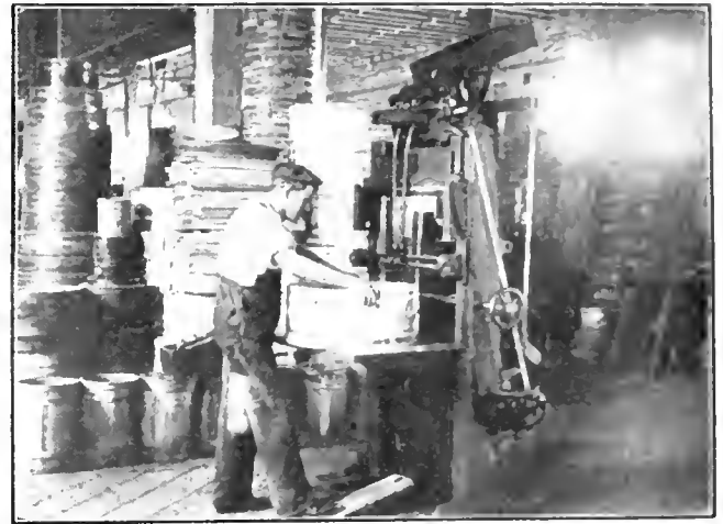
FIG. 6. WOOD PULLEYS BEING NAILED ON NAILING MACHINE.
