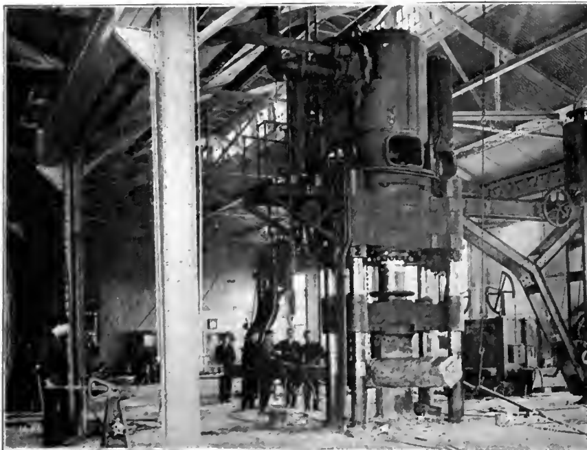
FIG. 1. 500 TON MESTA-HANIEL & LUEG PRESS AT WORK IN FORGE SHOP.
