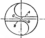
FIG. 1.—COMMON TYPE OF TWIST DRILL.
