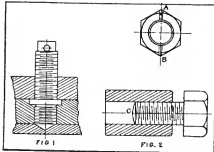
RIGHT AND WRONG WAY OF STUD DRIVING.
