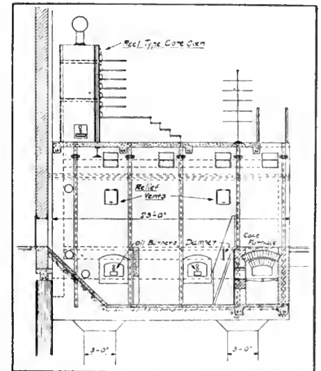
FIG. 4.—SECTION THROUGH FIRING PIT.
