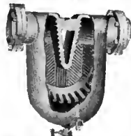
Steam and Oil Separator.
