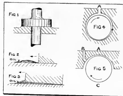
FIGS. 1 TO 5. FRICTION AND LUBRICATION.
