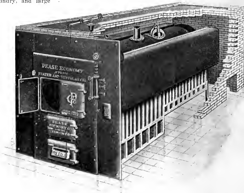
FIG. 9. "PEASE" ECONOMY STEAM HEATER AND VENTILATOR.
