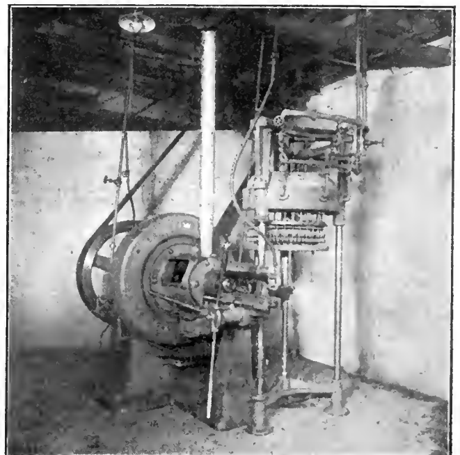
FIG. 2. SIDE VIEW OF HOT SWAGER.
