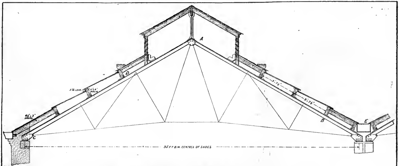
FIG. 3. ROOF FOR STEEL FOUNDRY, LANCASHIRE & YORKSHIRE RY., HORWICH.
