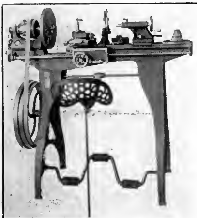
BARNES NO. 5 GAP LATHE.
