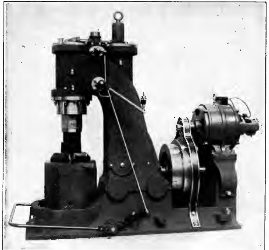
FIG. 1. BEECHE MOTOR DRIVEN AIR HAMMER.
