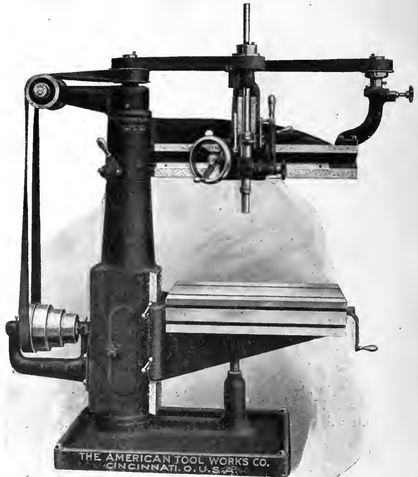
"AMERICAN" SENSITIVE RADIAL DRILL WITH ELEVATING TABLE.
