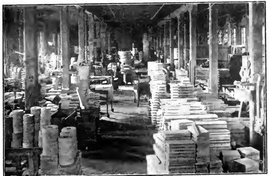
FIG. 4. VIEW ON MIDDLE FLOOR OF WOOD PULLEY FACTORY.
