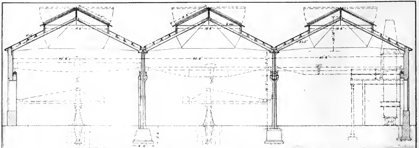
FIG. 9. ROOF OF IRON FOUNDRY, LOND ON & NORTH WESTERN RY. CREWELL
