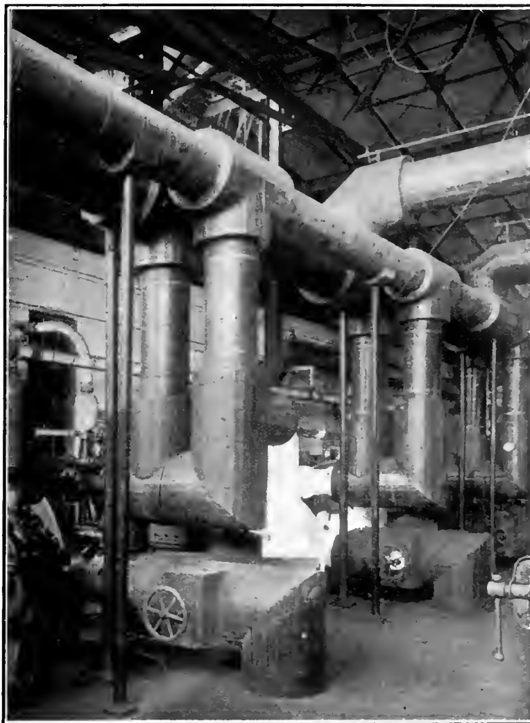
FIG. 1. CORK COVERING ON FLANGED BRINE PIPING AT STEEL CO. OF CANADA REFRIGERATING PLANT, HAMILTON, ONT. THE 8 IN. X 12 IN. SUCTION HEADERS ARE UNDER THE FLOOR.
