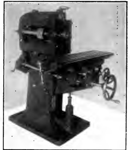
GARVIN TWO-SPINDLE PLAIN MILLING MACHINE.
