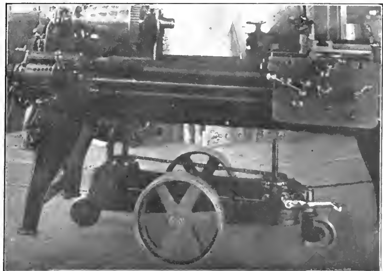
A LATHE TRUCK.
