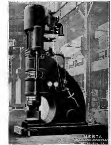
FIG. 3. MESTA-HANIEL & LUEG PRESS. BUILT FOR BROOKLYN NAVY YARDS.
