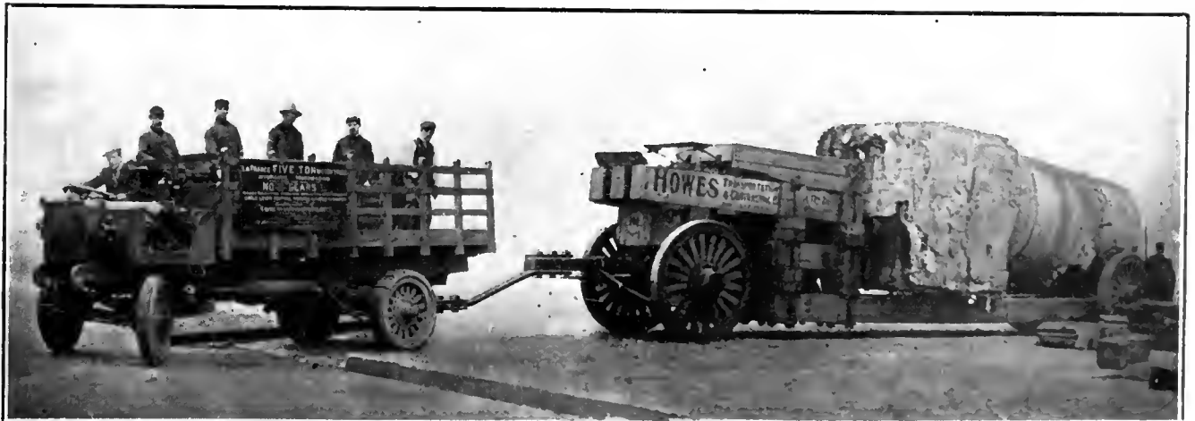
VIEW OF THE LA FRANCE TRUCK WITH ITS OWN LOAD AND THE TRAILING LOAD.
