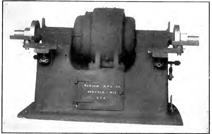
RANSOM MOTOR DRIVEN DRY GRINDER.
