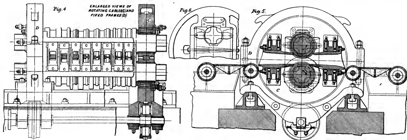
FIG. 4. ENLARGED VIEW OF ROTATING CABLES (C) AND FIXED FRAMES (D).
