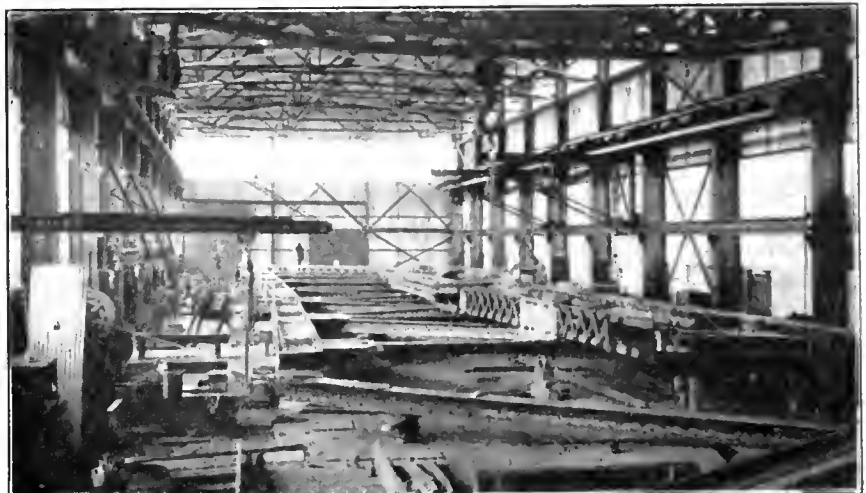
FIG. 5. GIRDER SHOP, LOOKING WEST. HERE IS SEEN UNDER CONSTRUCTION A 210 FT. RIVETED THROUGH LATTICE RAILWAY SPAN.
