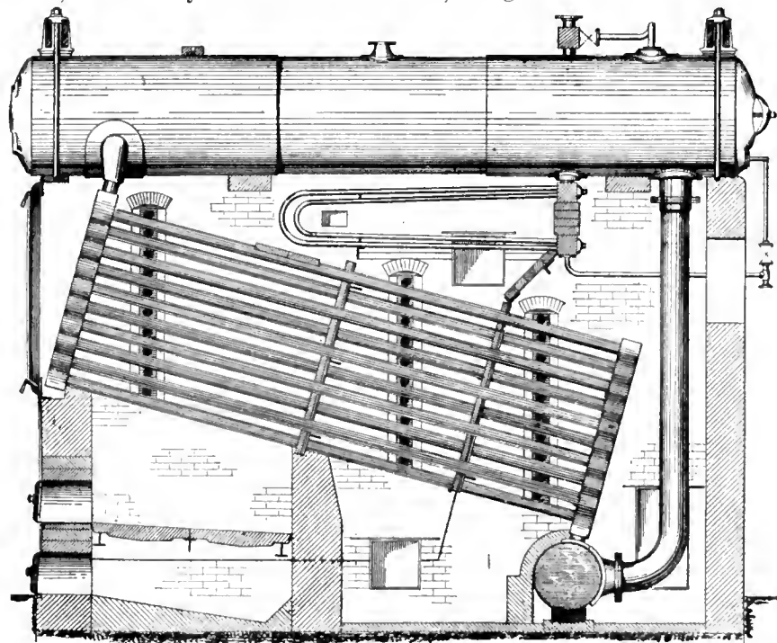
FIG. 1. GOLDIE & McCULLOCH STANDARD SECTIONAL WATER TUBE BOILER.
