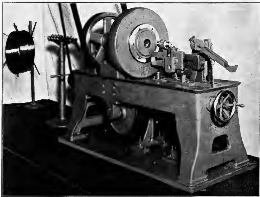
AUTOMOBILE WIRE WHEEL SPOKE SWAGING MACHINE.
