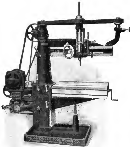
MOTOR-DRIVEN "AMERICAN" SENSITIVE RADIAL DRILL, WITH ELEVATING TABLE AND TAPPING ATTACHMENT.
