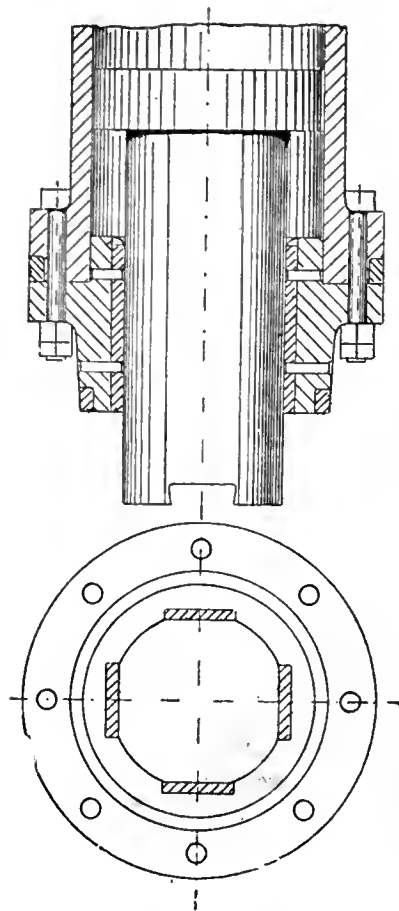
FIG. 2. RAM AND GUIDE, BEECHE AIR HAMMER.
