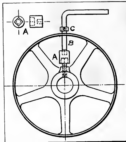
QUICK METHOD OF PUTTING SET SCREWS IN PULLEYS.
