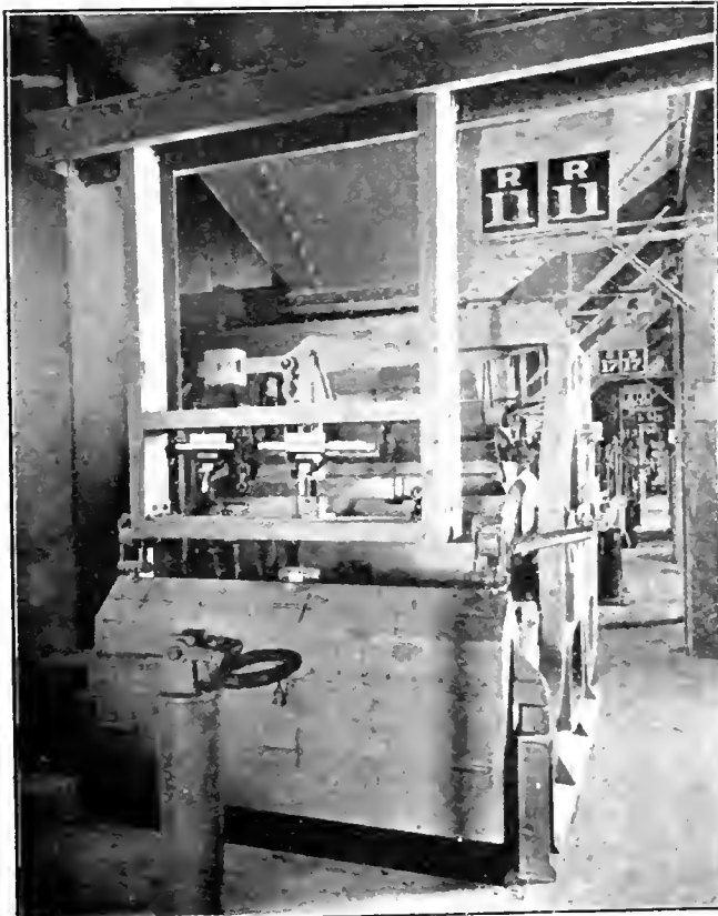
FIG. 8. AUTOMATIC WEIGHING MACHINE. 5,000 LBS. PER DRAFT
