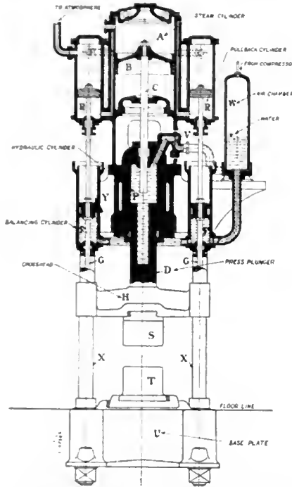
FIG. 2. SECTIONAL DRAWING OF MESTA-HANIEL & LUEG PRESS.
