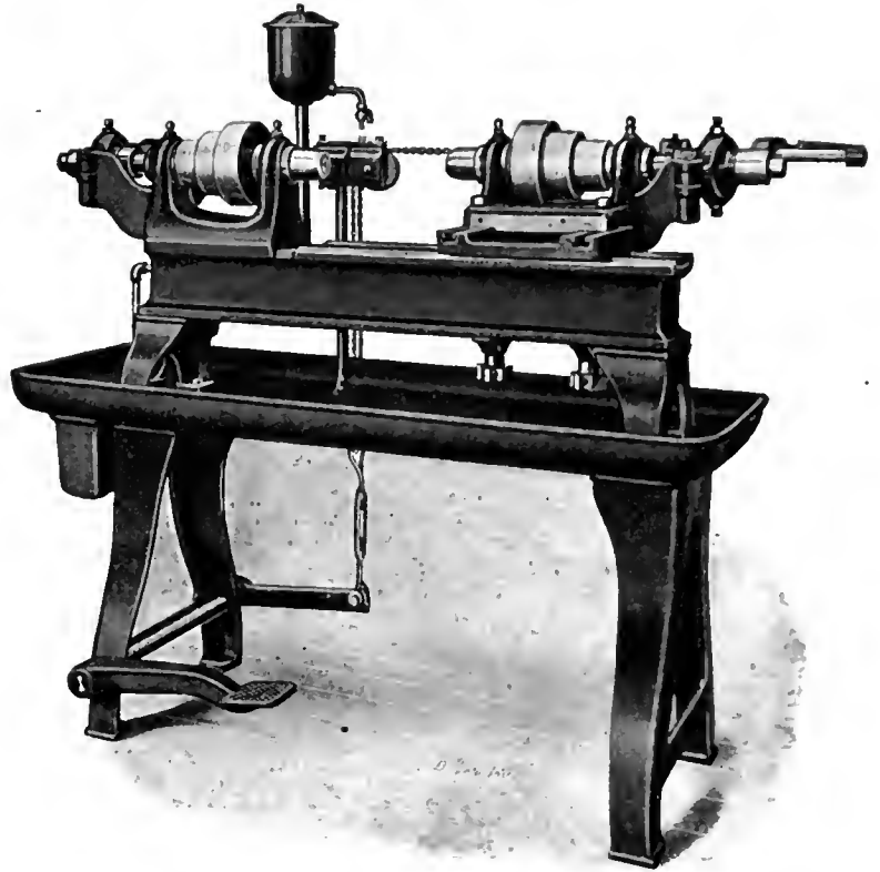
TWO SPINDLE DRILLING LATHE.
