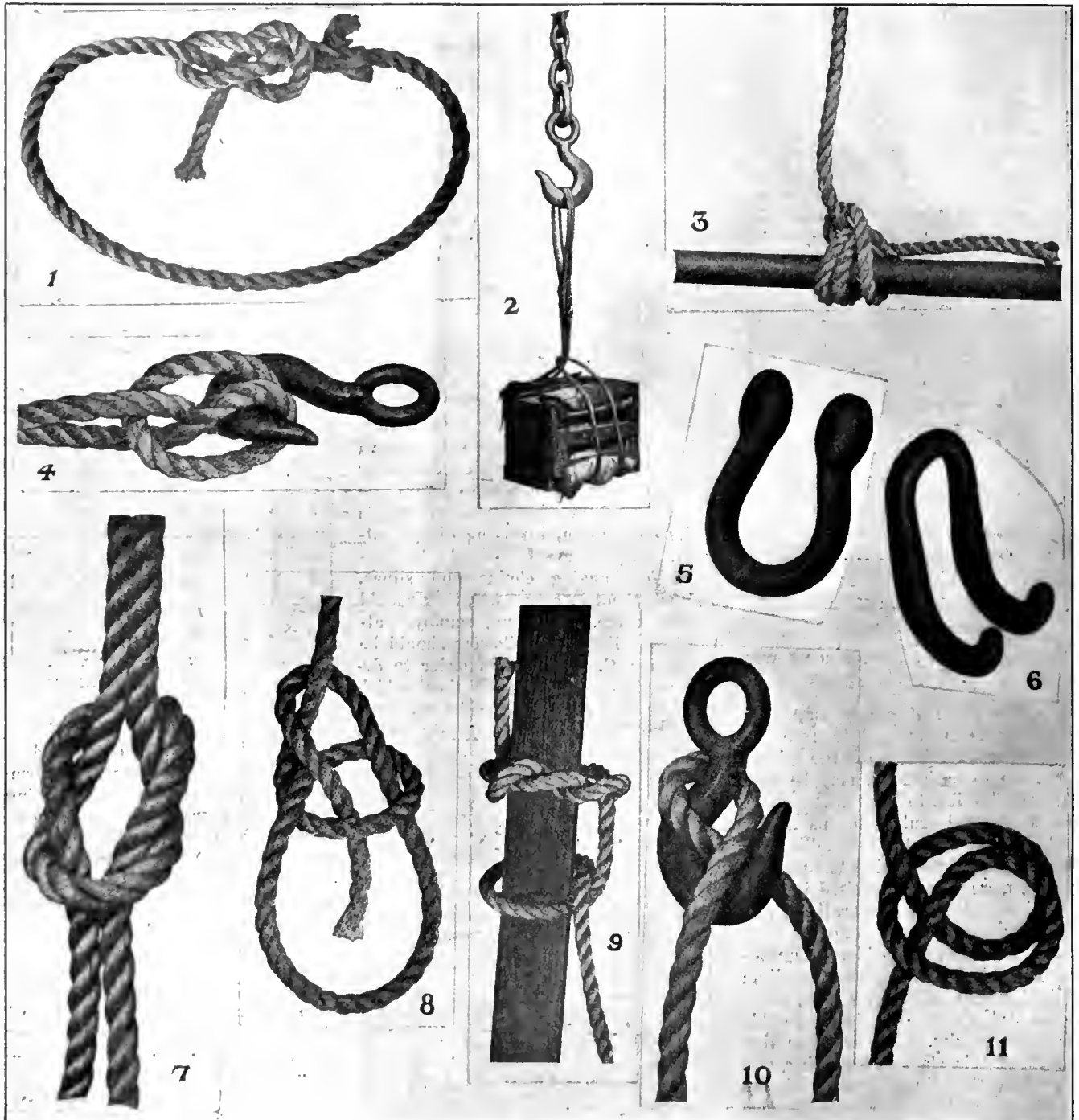
FIG. 1. SHEET BEND IN EYE. FIG. 2. DOUBLE CABLE SLING, RIGHT WAY TO LIFT LOAD. FIG. 3. STUDDING SAIL HITCH. FIG. 4. CLOVE OR DOUBLE HALF HITCH. FIG. 5. SHACKLE. FIG. 6. DOUBLE HOOK. FIG. 7. SQUARE OR REEF KNOT. FIG. 8. BOWLINE COMPLETE. FIG. 9. TIMBER HITCH AND HALF HITCH. FIG. 10. BLACKWALL HITCH. FIG. 11. CLOVE OR DOUBLE HALF HITCH.
