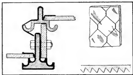
FIG. 12. SECTION THROUGH JOINTING OF SKYLIGHT WITH MAIN SASH FRAME. PENNYCOOK'S PATENT GLAZING.
