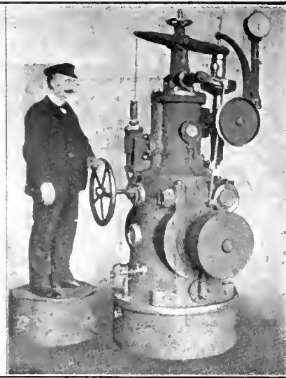
FIG. 18. EXCITER GOVERNOR.
