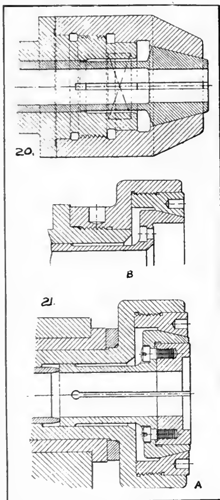
FIG. 20. SHOWING CLOSER FOR PUSH-OUT CHUCK OF SMALL DIAMETER.
