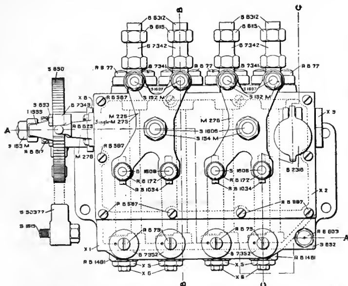
FIG. 1. MECHANICAL CYLINDER LUBRICATION. TOP VIEW.
