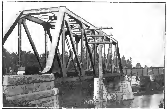
FIG. 7. THROUGH RIVETED LATTICE GIRDER SPAN AND THROUGH PLATE GIRDER SWING SPAN (IN THE DISTANCE), ERECTED OVER RIVER THAMES, AT CHATHAM, ONTARIO.
