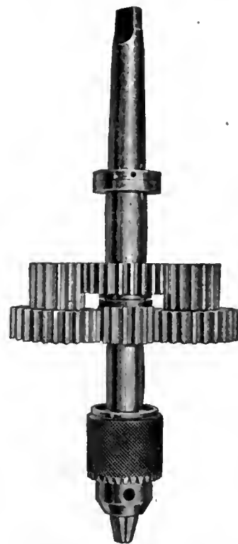
FIG. 4. ENTIRE MOVING PARTS OF SPEEDER. NOTE THE BALL-BEARING AT CENTRE.
