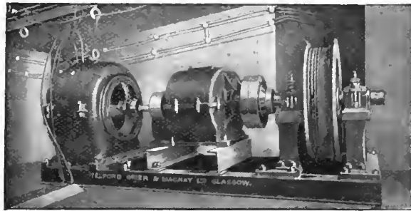
FIG. 2.—CHAIN REDUCTION GEARS.
