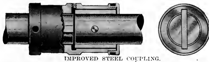
IMPROVED STEEL COUPLING.
