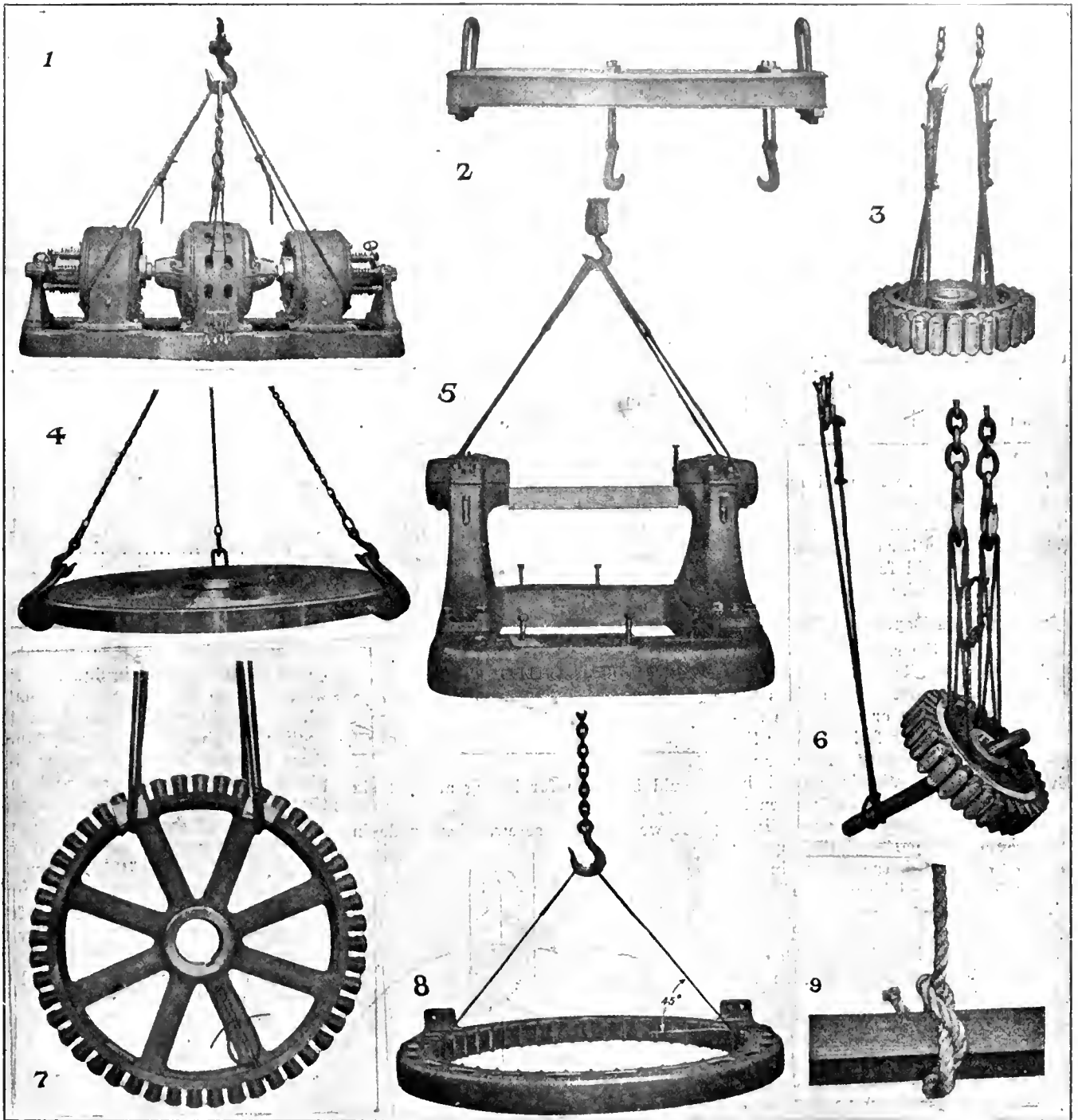
FIG. 1. PROPER WAY OF LIFTING THREE UNIT SET. FIG. 2. EQUALIZER USED WITH TWO CRANES. FIG. 3. METHOD OF LIFTING AND TURNING REVOLVING FIELDS, FIRST POSITION. FIG. 4. RIGHT WAY OF LIFTING PLATE WITH THREE HOOKS. FIG. 5. METHOD OF LIFTING BASE AND STANDARDS. FIG. 6. METHOD OF LIFTING AND TURNING REVOLVING FIELDS, SECOND POSITION. FIG. 7. RIGHT WAY TO LIFT REVOLVING FIELD. FIG. 8. 45 DEGREE ANGLE SLING, RIGHT WAY. FIG. 9. TIMBER HITCH.
