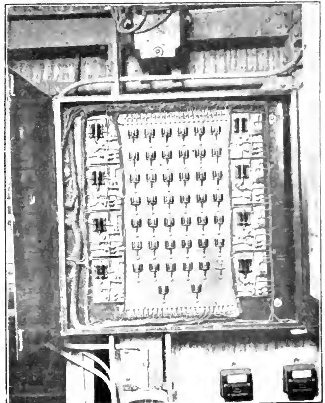
FIG. 12. RELAY PANEL FOR SIGNAL.
