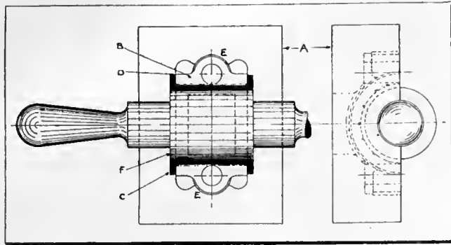
FIG. 1.—BABBITTING FIXTURES.
