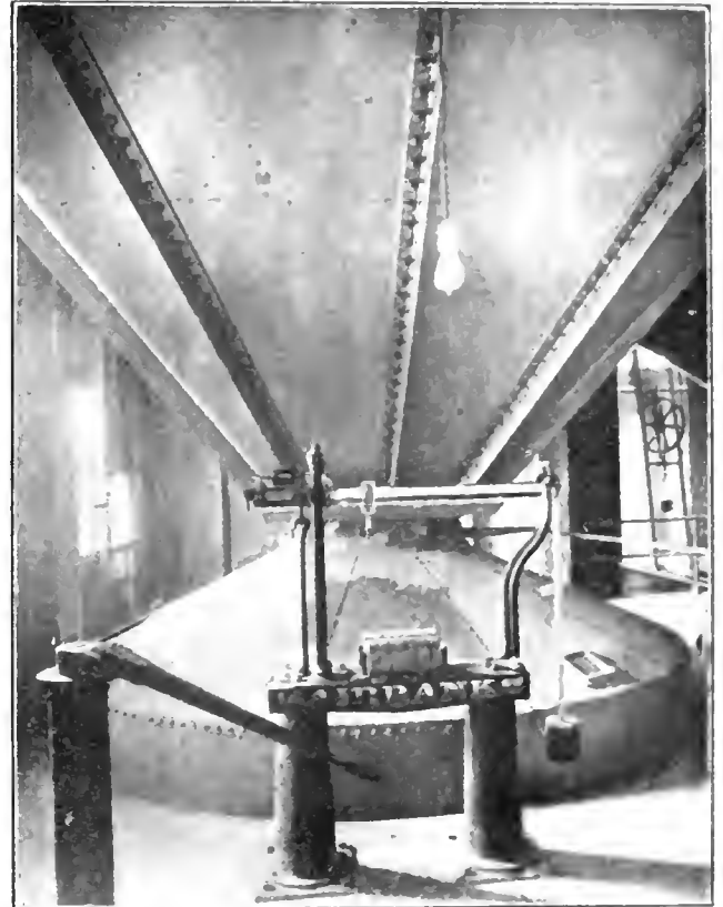
FIG. 7. 2,000 BUSHEL HOPPER SCALE.
