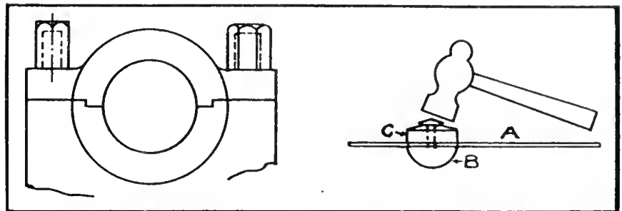
FITTING NUTS.
