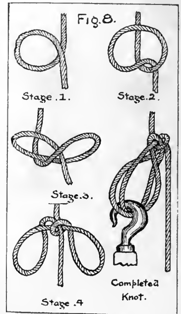
KNOTS AND SLINGS.
