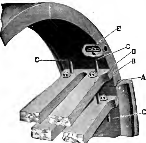
FIG. 7. DETAIL OF CONSTRUCTION OF "DODGE" WOOD PULLEY.
