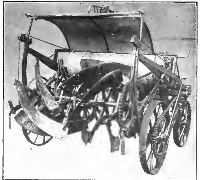
FIG. 2. REAR VIEW OF SAND MIXING MACHINE.
