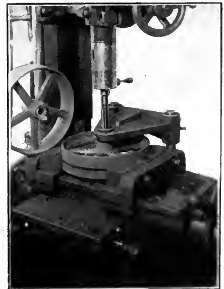
FIG. 3. GEAR AND PULLEY DRILLING AND REAMING FIXTURE.
