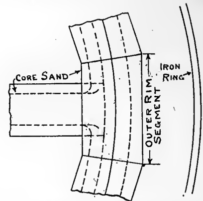
FIG. 9. METHOD OF MOULDING LARGE PULLEYS.
