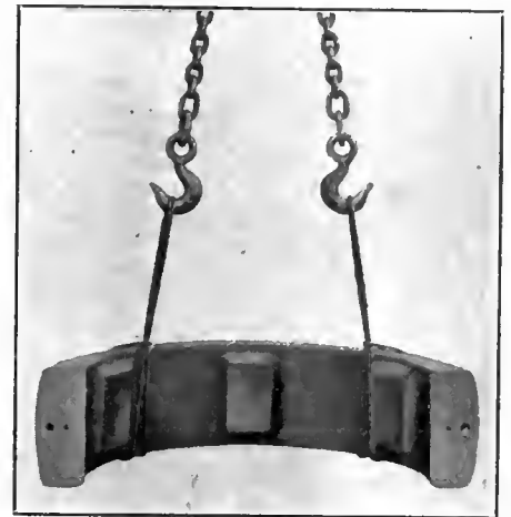
PROPER METHOD OF MAKING HITCH. THE FRICTION OF CABLE AROUND THE OBJECT GIVES APPROXIMATELY A TWO PART CABLE.
