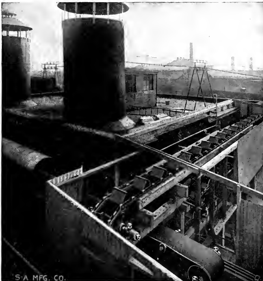
FIG. 1. CONVEYER-ELEVATOR AND BELT CONVEYER.
