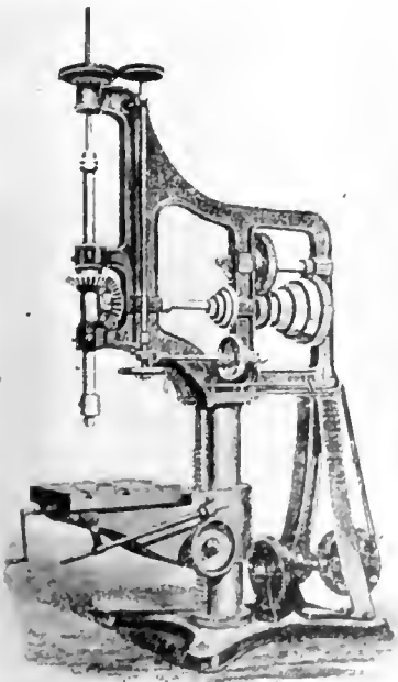
VERTICAL DRILL BUILT ABOUT THE YEAR 1869
