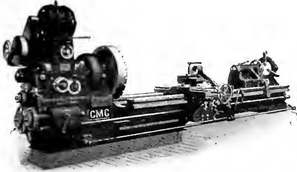
MOTOR-DRIVEN 36-INCH TRIPLE-GEARED ENGINE LATHE.
