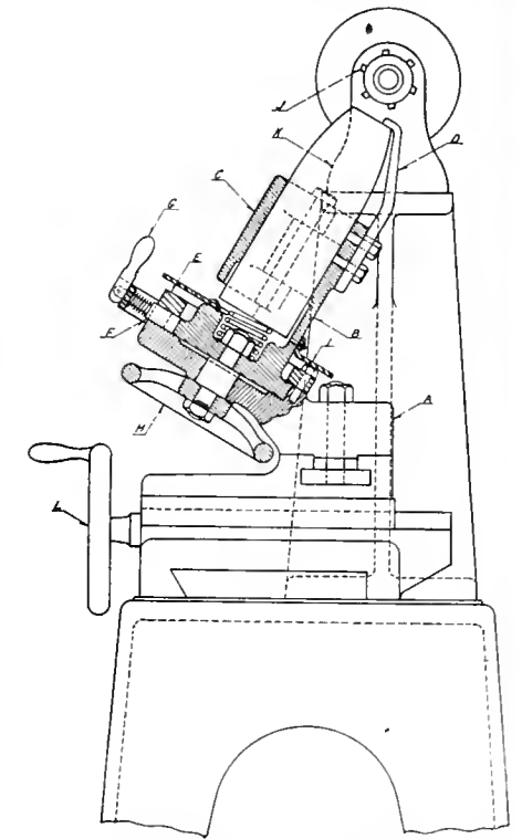
FIG. 12. SECTIONAL ELEVATION OF NOSE SLOTTING MACHINE.
