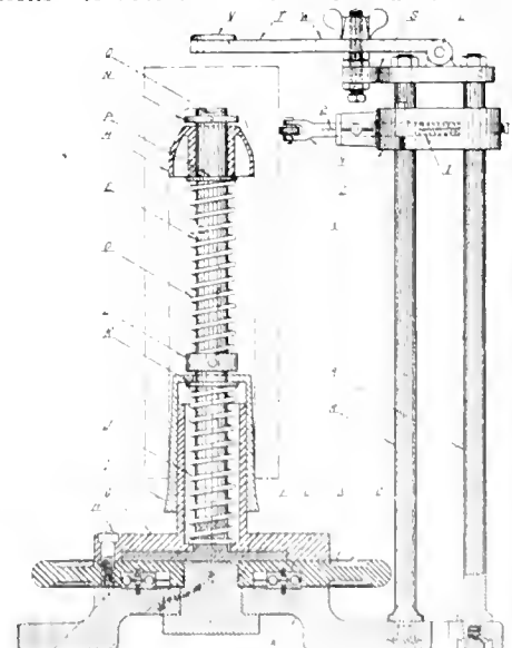
FIG. 2. CENTERING SHELLS.
