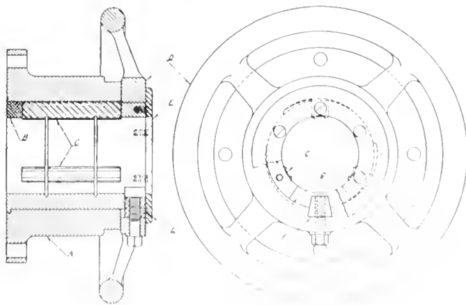
FIG. 8. COMPRESSION CHUCK.
