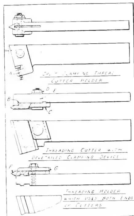
FIG. 16. GROUP OF CUTTERS AND HOLDERS USED FOR THREADING.
