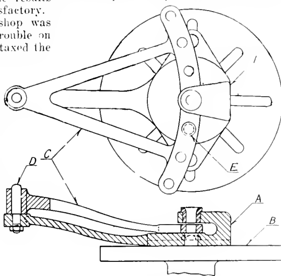
JIG FOR DRILLING SEXTANTS
