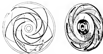
a—Flat. b—Perspective. Fig. 7. Flow Tangential and Spiral.
