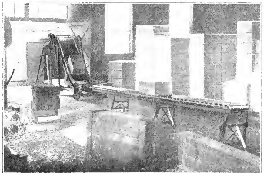
FIG. 5. CARRIERS DELIVERING TO INCLINE PLATFORM ELEVATOR LOADING CARS FROM STOCK PILE.
