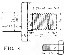
ASSEMBLY AND DETAIL OF ADAPTER FOR TIGHTENING SHELL NOSES.
