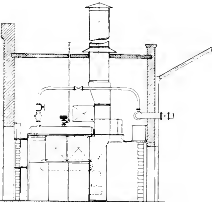
SIDE ELEVATION OF "HOWDEN" BOILER INSTALLATION AT BOROUGH OF BERMONDSEY ELECTRIC LIGHT STATION
