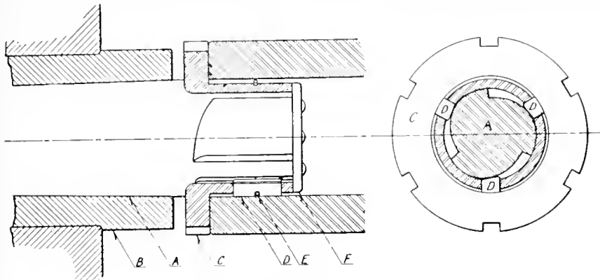
FIG. 1—EXPANDING ARBORS.
