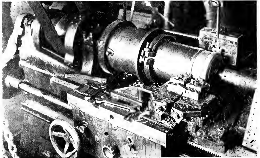
WAVING AND UNDERCUTTING- GRAY MFG. & MACHINE CO. ATTACHMENT.
