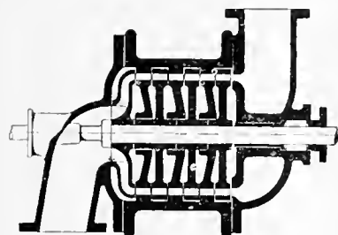
Fig. 11. Combined Axial and Spiral Flow.
