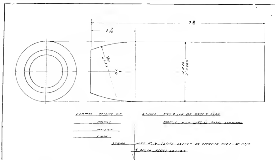
EIGHTH OPERATION—PROFILE AND OUTSIDE BODY FINISH.
