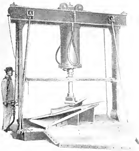
RECLAIMING PRESS FORMING HOPPER SHEETS FOR STEEL CARS.
