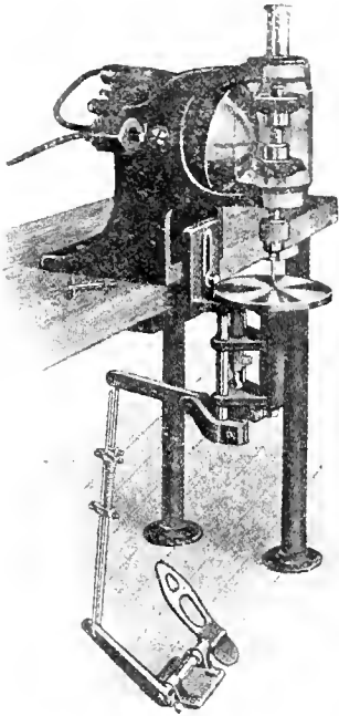
MOTOR DRIVEN BENCH TRAPPING MACHINE.
