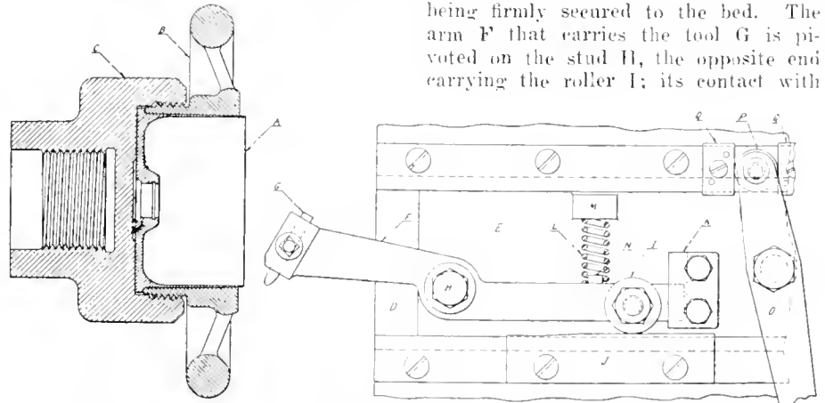
DEVICE USED IN MACHINING MOUTH OF 4.5 IN. CARTRIDGE CASES.
