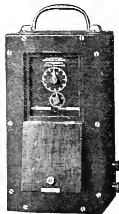
CYCLE COUNTER OR TIMING DEVICE
