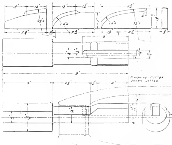
FIG. 5. TOOLS AND BAR FOR INSIDE NOSE PROFILE
