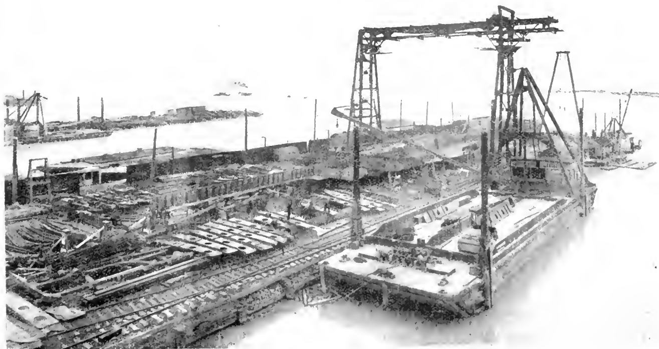
ELECTRICALLY OPERATED GANTRY AND SHIPBUILDING BERTH AT THOR IRON WORKS, TORONTO
