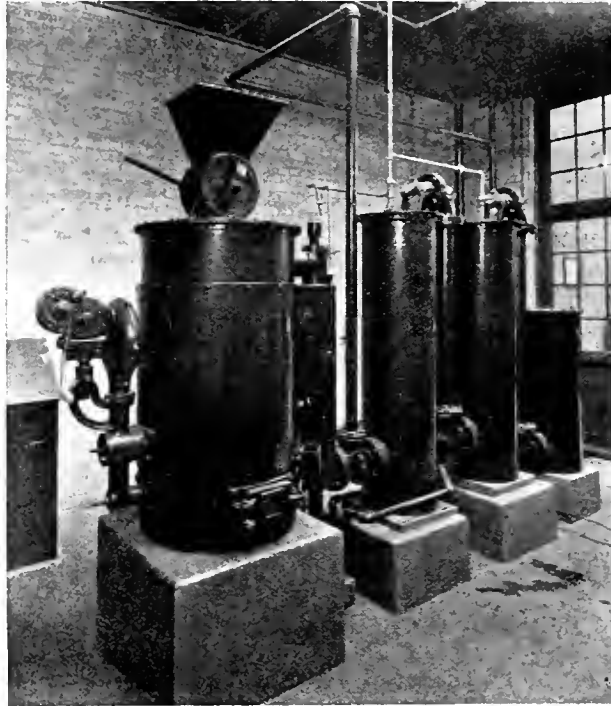
THERMODYNAMIC LABORATORY—SUCTION GAS PRODUCER PLANT.
