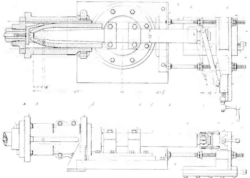
FIG. 6. ROUGH BORING ATTACHMENT ON "PETRIE" LATHE.
