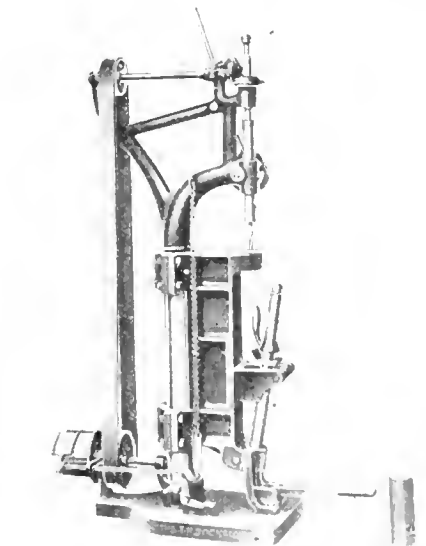
FIG. 2. CENTERING MACHINE WITH TILTING, EXPANDING ARBOR.
