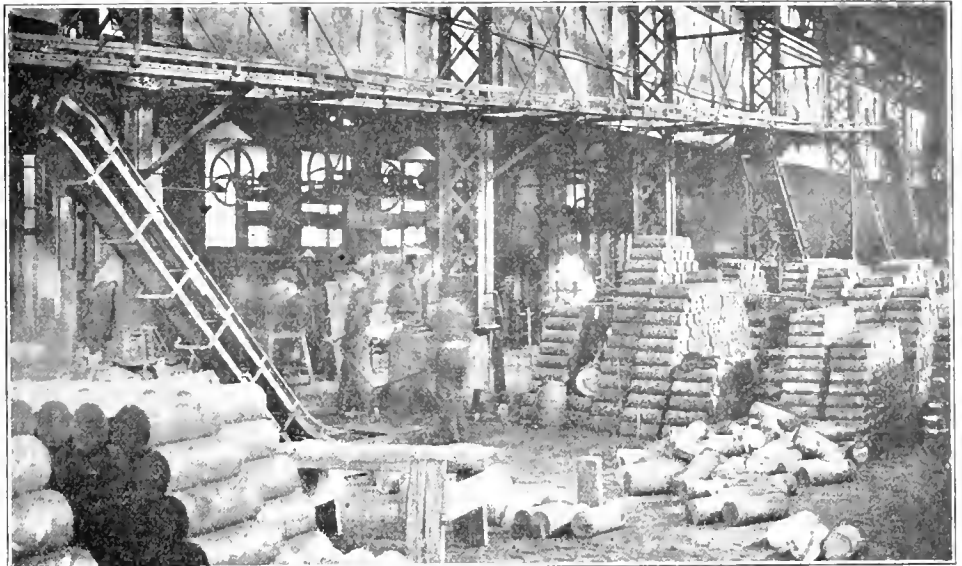
Steel Shell Forgings or Billets of any size or weight will move any distance or about curves upon our specially constructed Gravity Carriers and Incline or Horizontal power devices. No labor required.
