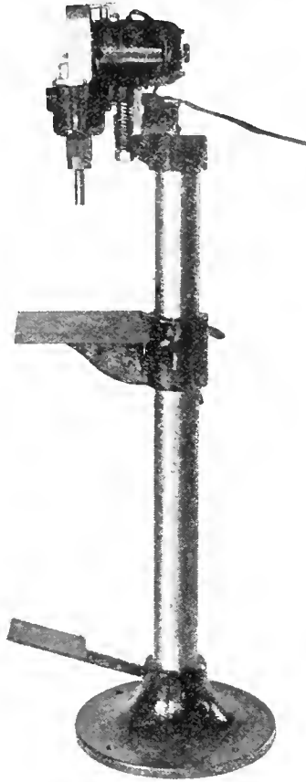
ELECTRIC RIVETER FOR SHELL BASE PLATES.
