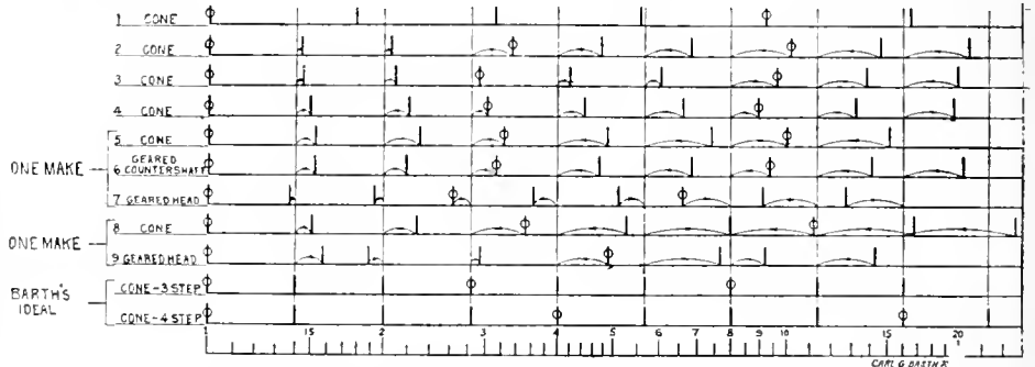
FIG. 7. LOGARITHMIC PLOT OF SINGLE COUNTERSHAFT SPEED SERIES OF NINE 16-INCH LATHES SUBMITTED BY VARIOUS MANUFACTURERS IN FEBRUARY, 1914.
