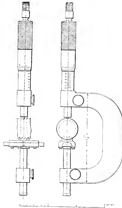
FIG. 5. APPARATUS FOR CORE DIAMETER MEASUREMENT.
