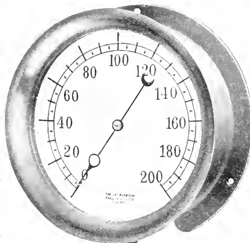
STEAM PRESSURE GAUGE.
