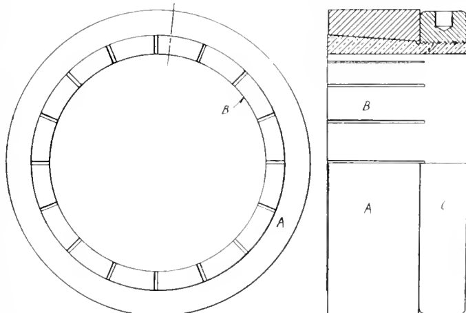
FIG. 9. STEADY HEAD BUSHING.
