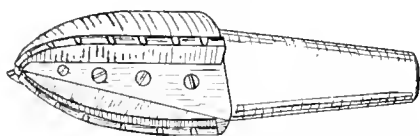
FIG. 7. ACORN TYPE OF HEAD FOR MACHINING INTERIOR PROFILE OF NOSE.
