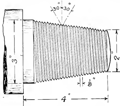
TYPE OF THREAD USED FOR COUPLING OIL WELL TOOLS.
