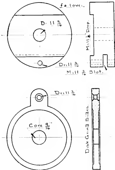
FIG. 4. GOVERNOR WEIGHTS.
