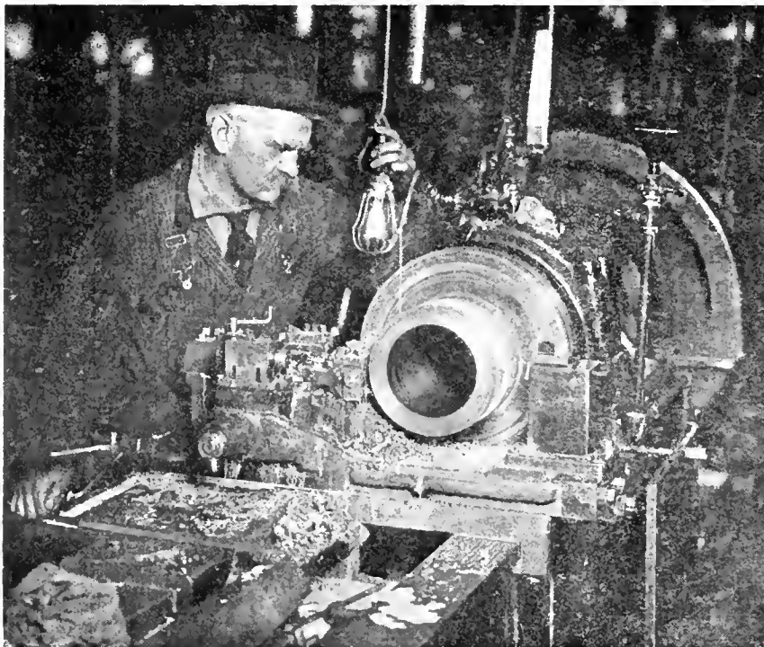
FIG. 7. WAVING AND GROOVING "R. & V." MACHINES.
