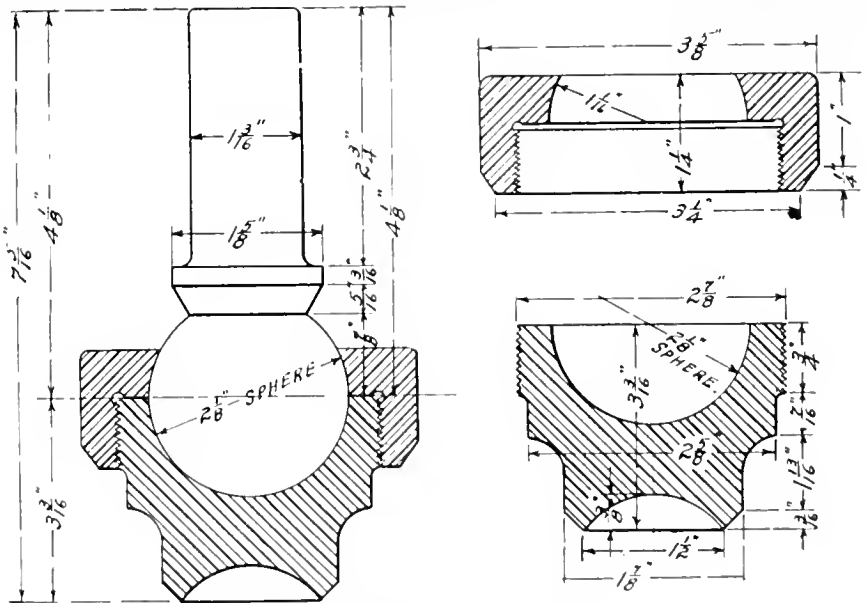
DETAILS OF ADJUSTABLE RIVET SNAP.
