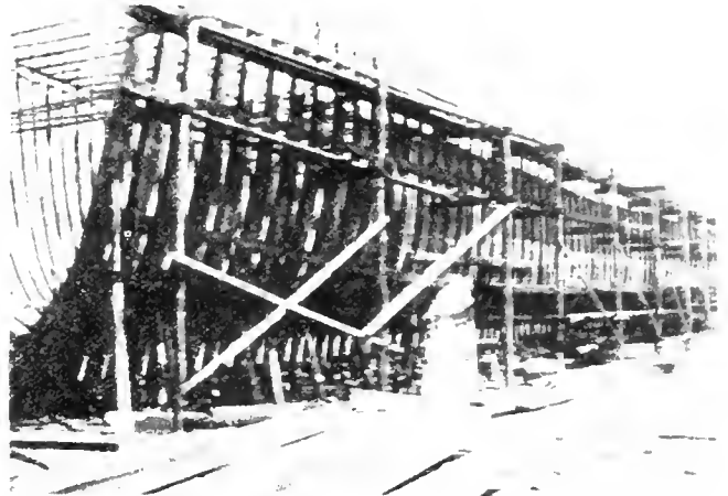
FIG. 2. NEARER VIEW OF A THREE-DECK STAGING.
