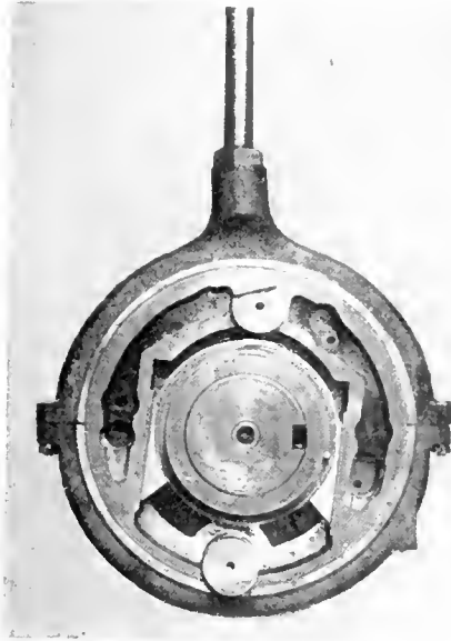
FIG. 8. ASSEMBLED GOVERNOR
