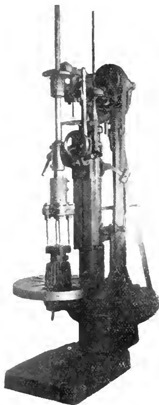
FIG. 1. MULTIPLE DRILL HEADS.
