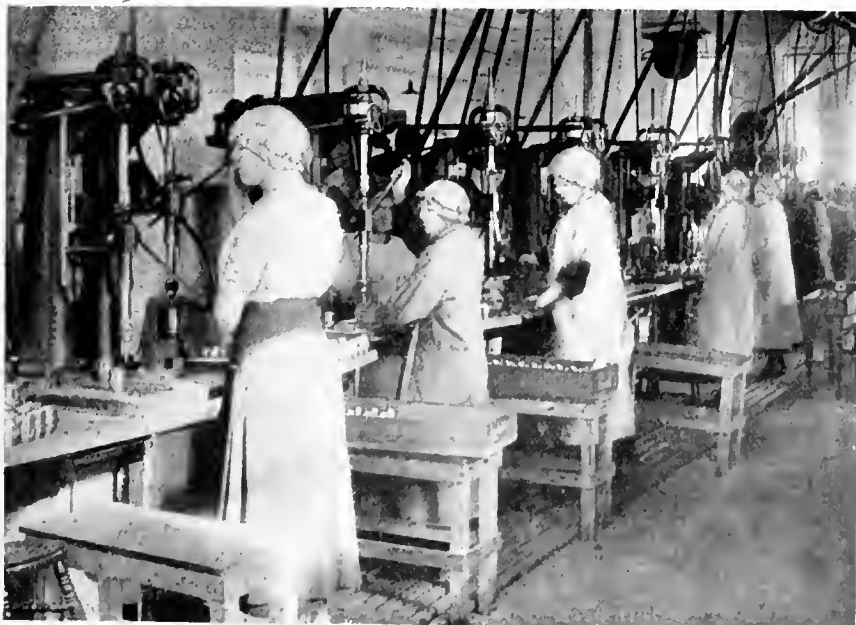
FIG. 5. BATTERY OF "HENRY & WRIGHT" DRILLS ON BODY DETAIL OPERATIONS.
