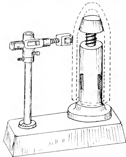
FIG. 2. GAUGING FIXTURE FOR CHECKING CONCENTRICITY OF FORGING
