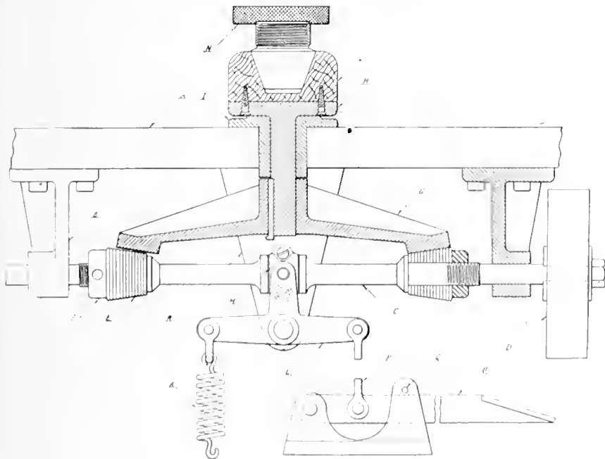
FIG. 11. GAUGING MACHINE FOR FUSE THREADS.
