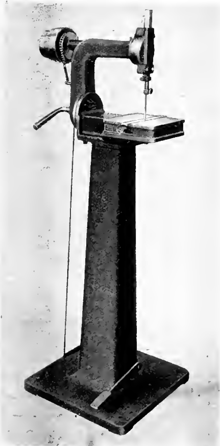
FILING MACHINE WITH OVERHUNG SWIVELING HEAD AND ADJUSTABLE FILE SUPPORT.
