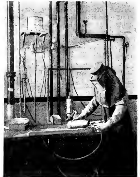
FIG. 13. PAASCHE AIR BRUSH EQUIPMENT FOR VARNISHING THE INTERIOR OF THE SHELLS.
