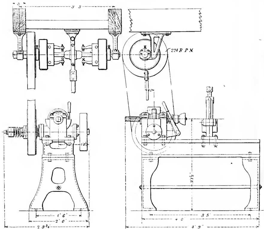
FIG. 2. INSTALLATION DETAIL OF SHELL NOSE TIGHTENING MACHINE.
