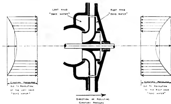
FIG. 18. EFFECTS OF GYROTORY PRESSURE ON END THRUST.
