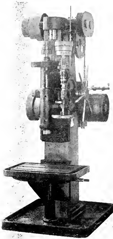
TRAVERSING HEAD VERTICAL DRILL PRESS WITH BELT FEED.
