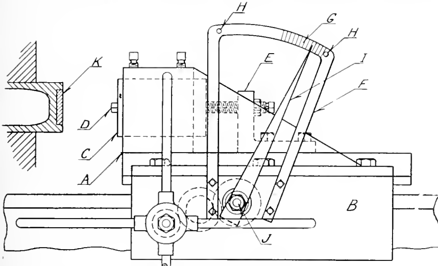
CUTTING SHELLS TO WEIGHT.
