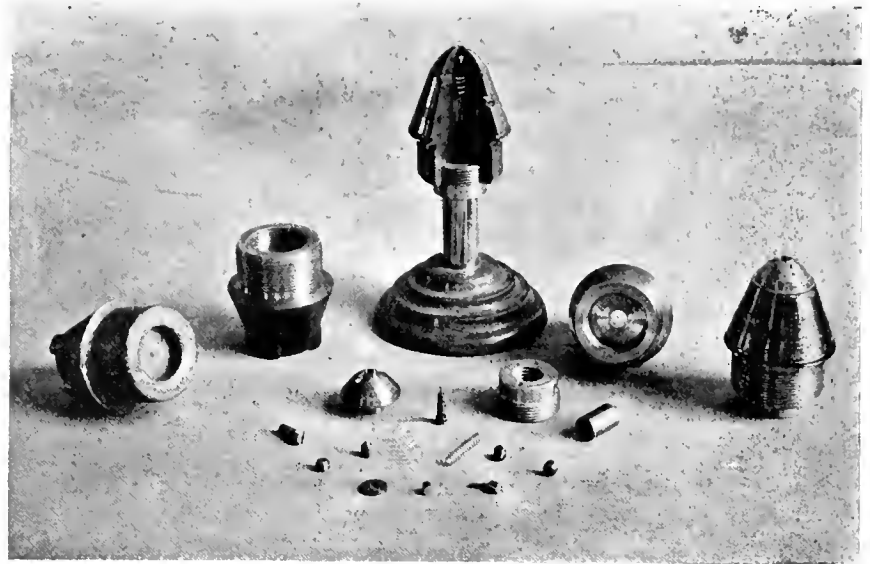
FIG. 13. VIEWS OF FUSE AND ITS COMPONENT PARTS.
