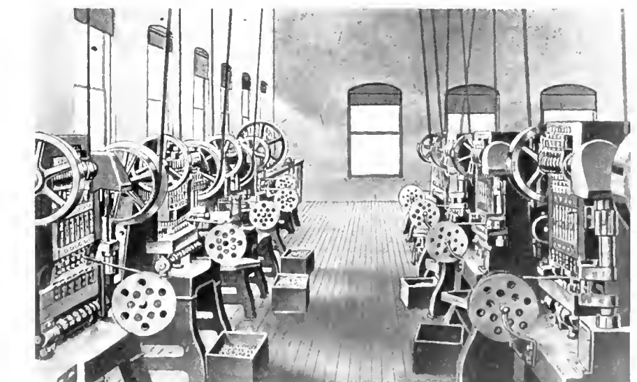
VIEW OF PRESS ROOM EQUIPPED WITH MULTIPLE PLUNGER PRESSES SLOWING REELS OF STOCK
