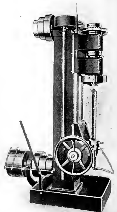
HOLLOW SPINDLE DRILLING MACHINE.
