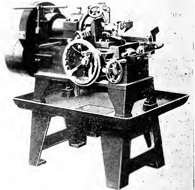
FIG. 9. GROOVING MACHINE WHICH GROOVES, WAVES, AND UNDERCUTS COMPLETE.
