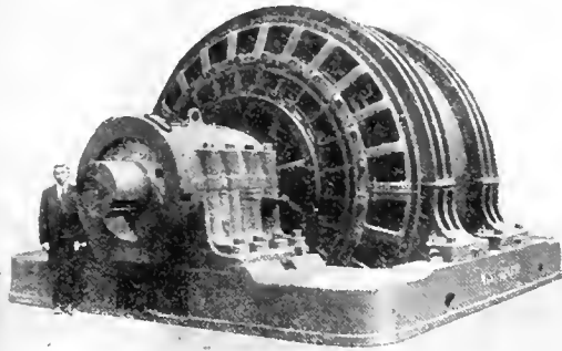
LARGE ELECTRIC MOTOR.
