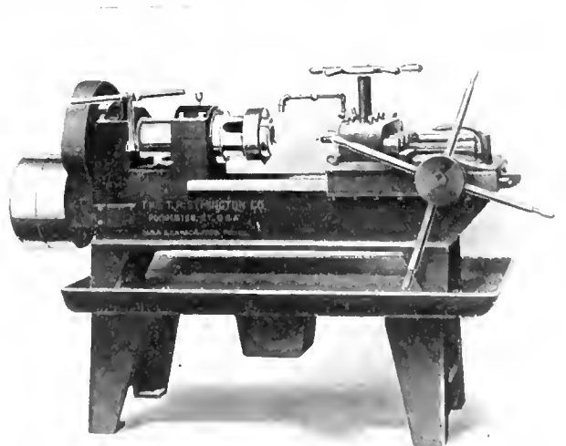
FIG. 7. FOUR TOOL MACHINE FOR MACHINING AND FINISHING THE INTERIOR
