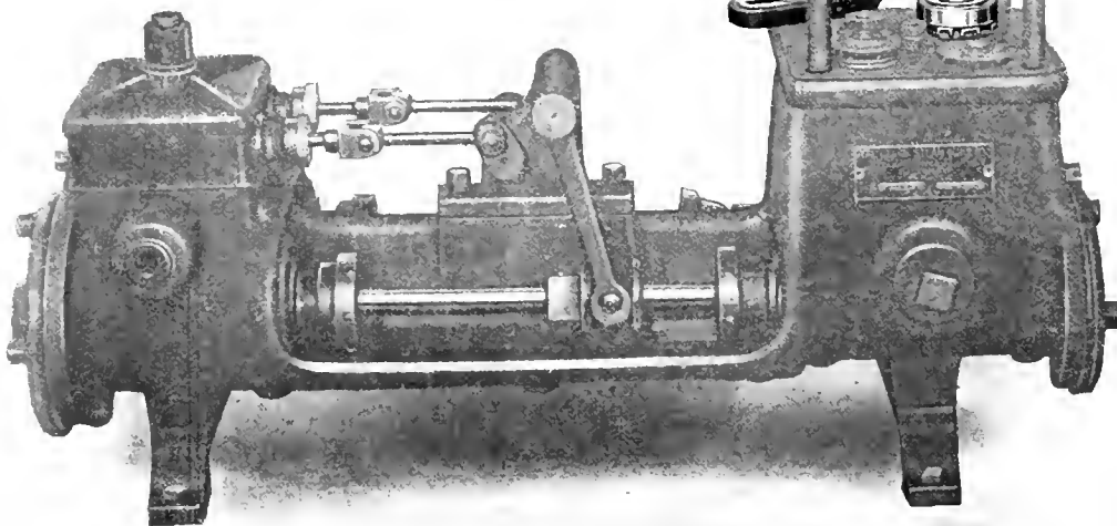
DEXTER SINGLE YOKE PUMP VALVE RESEATING MACHINE REFACING DISCHARGE VALVE SEAT OF DUPLEX STEAM PUMP.
