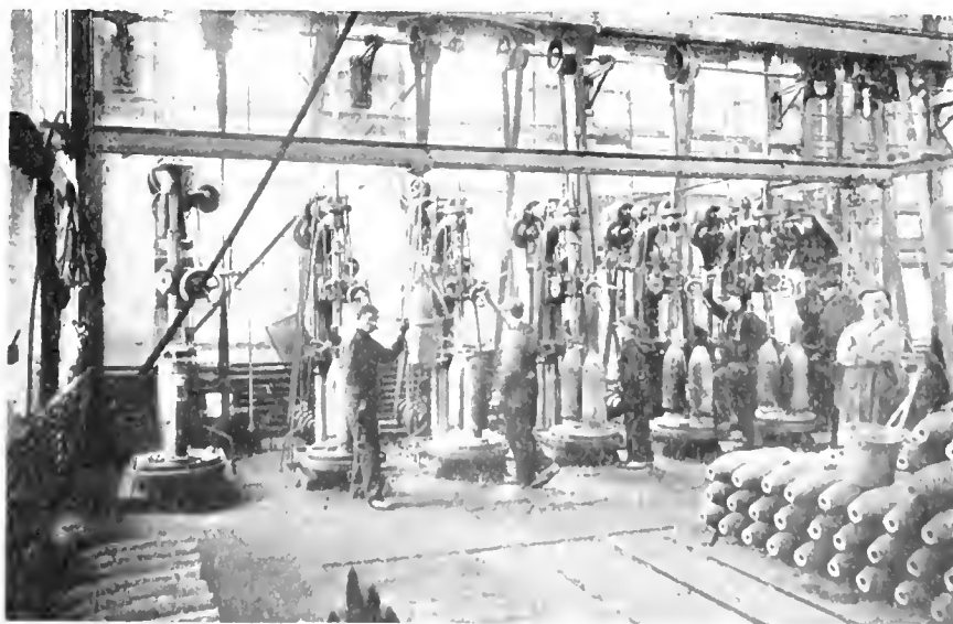
FIG. 3. BATTERY OF DRILL PRESSES WITH REVOLVING TABLE EQUIPMENT DRILLING AND FACING HOLE IN NOSE.
