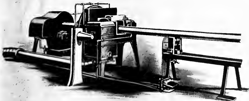
FLUE WELDER WITH GUARDS AND FURNACE ATTACHED.
