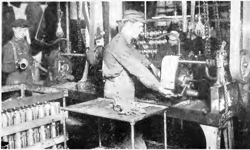
FIG. 12. "LYMBURNER" DOUBLE END CRIMPING MACHINES ROUNDING-OFF CORNERS OF SHELL BASE AND CUTTING SMALL GROOVE JUST BELOW NOSE.
