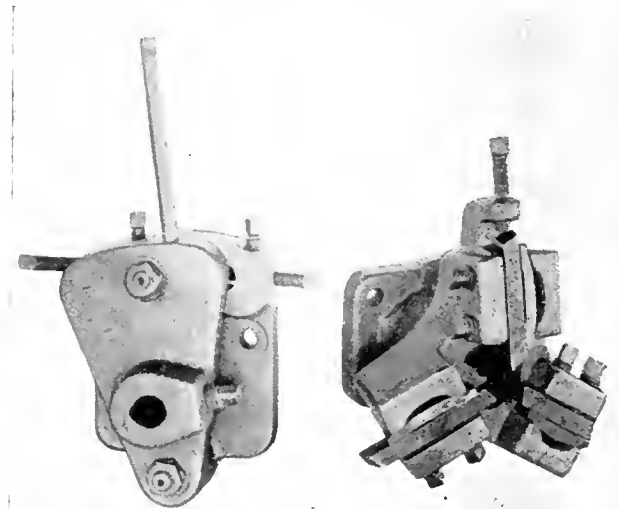
FIG. 2. LEFT, RECESSING TOOL. RIGHT, HOLLOW MILL.
