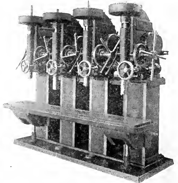
GANG ARRANGEMENT, SINGLE PURPOSE HIGH SPEED DRILLING MACHINE.
