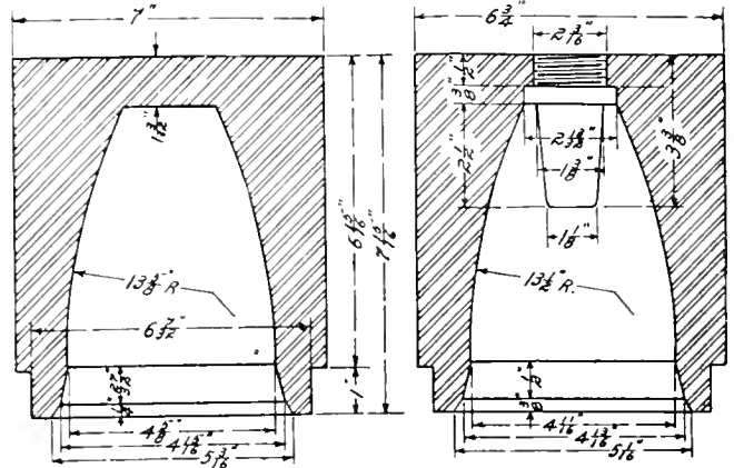
FIG. 5. NOSING DIES.
