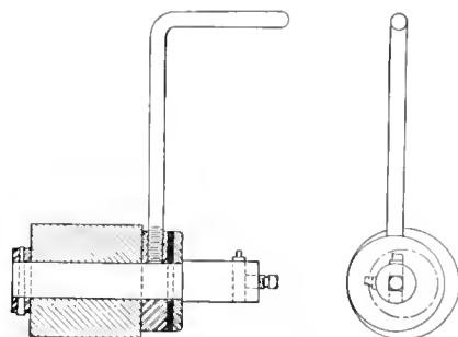
7A. NOSE RECESSING TOOL.
