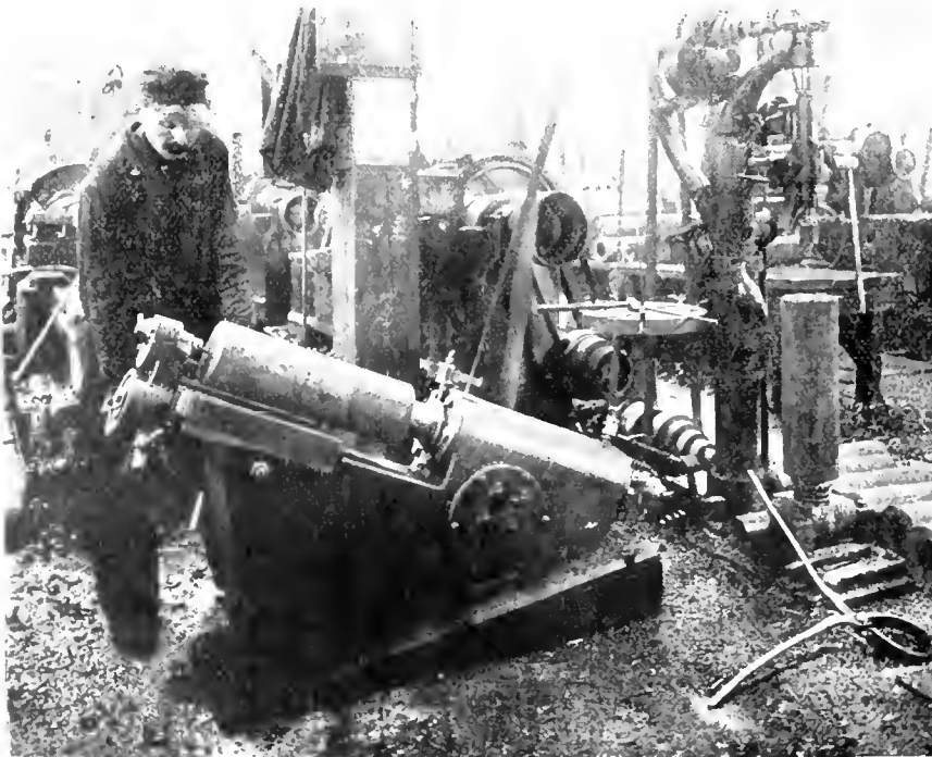
VICTORIA FOUNDRY CO. MACHINE FOR CENTERING BASE OF SHELLS.
