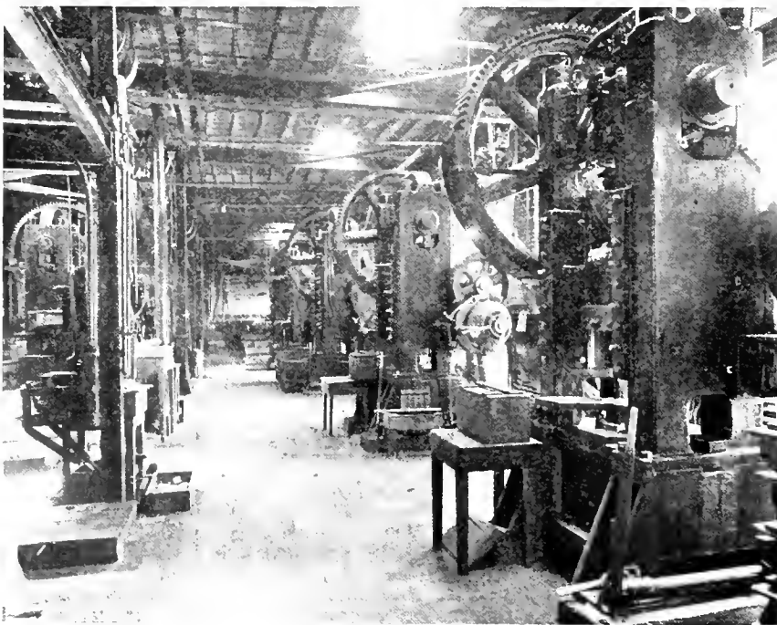
HEAVY DRAW PASSES FOR EARLIER DRAWING OPERATIONS.
