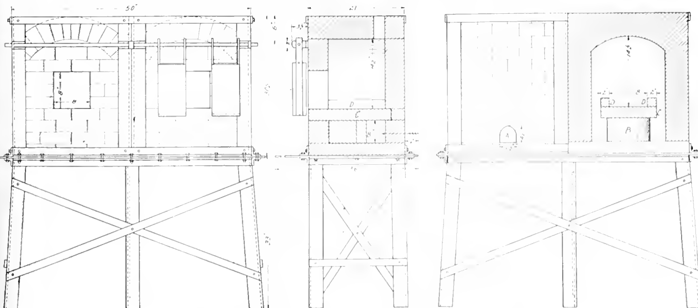
FIG. 2.—DETAILS OF CONSTRUCTION OF TWIN MUFFLE FURNACE.
