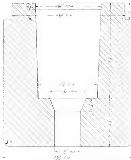
FIG. 2. KNOCK-OFF PROVISION FOR PIERCED BLANK.
