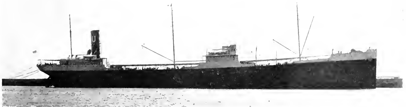
STEAMSHIP "LA BREA" PROPELLED BY 2,600 HORSE POWER "CURTIS" TURBINE DRIVING THROUGH "ALQUIST" REDUCTION GEARS.
