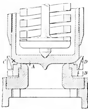
FIG. 5. EXPERIMENTAL VALVE.
