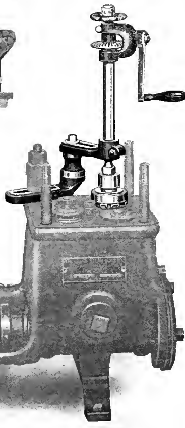
DEXTER SINGLE YOKE PUMP VALVE RESEATING MACHINE REFACING DISCHARGE VALVE SEAT OF DUPLEX STEAM PUMP.
