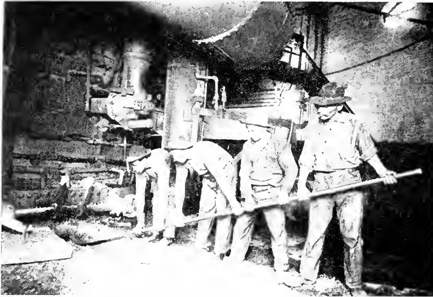
FIG. 13. UNSAFE METHOD OF DRILLING A TAPPING HOLE.
