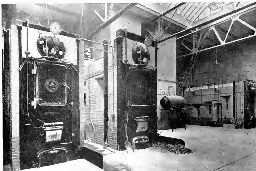
BOILER ROOM ONE 100 H.P. AND TWO 50 H.P. BARBOCK & WILCOX WATER TUBE BOILERS.
