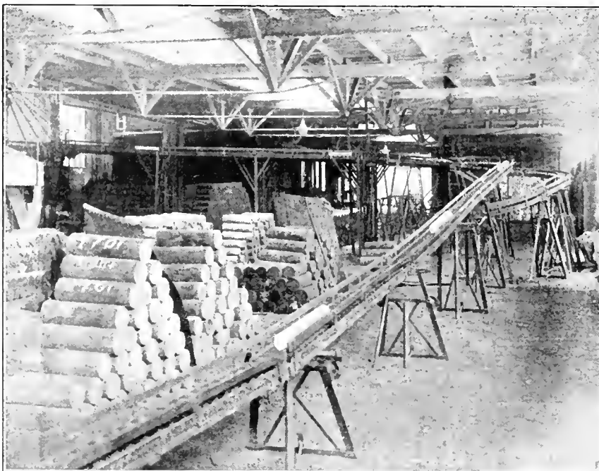
FIG. 2 PORTION OF CONVEYOR TRANSFERRING BILLETS DIRECT FROM CARS TO BATTERY OF CONTINUOUS FURNACES.
