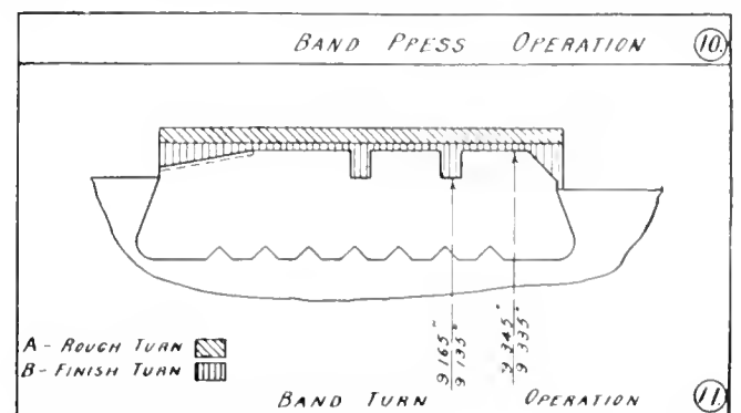
FIG. 14. MACHINING OPERATION SHEETS, .92 INS. HIGH EXPLOSIVE SHELL.
