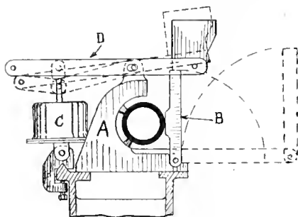
FIG. 5. HYDRAULIC CLAMPING FIXTURE FOR SHELLS.
