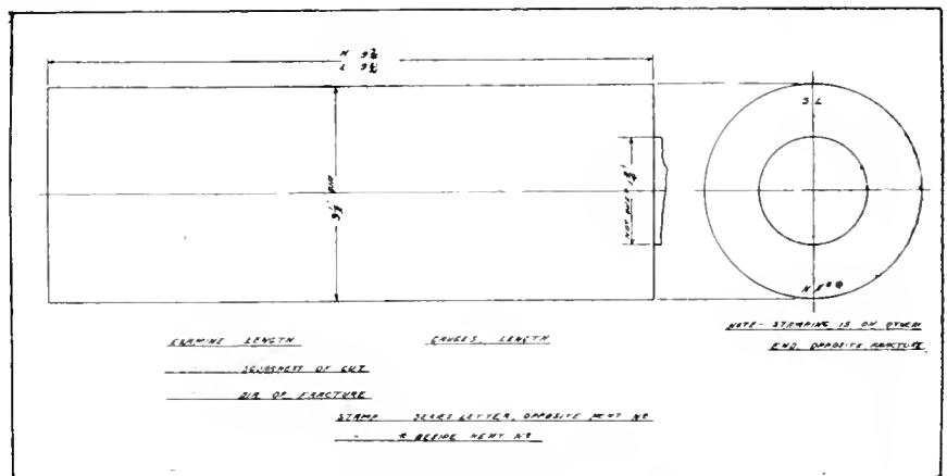
SECOND OPERATION—PART AND BREAK.
