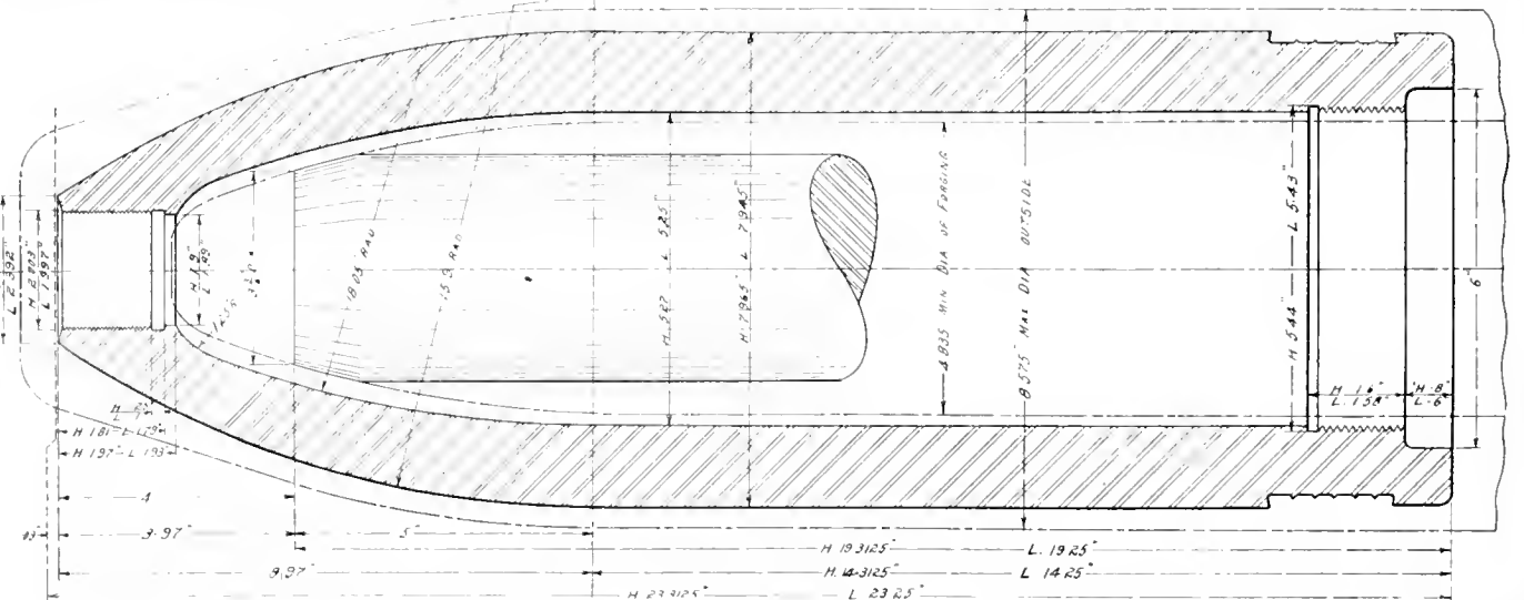
FIG. 4. DIMENSION SHEET FOR PRIMARY OPERATIONS, WITH SECTIONAL VIEW OF FINISHED SHELL, ALSO OUTLINE OF ROUGH FORGING.
