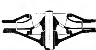
FIGS. 16 AND 17. IMPELLERS BALANCED.
