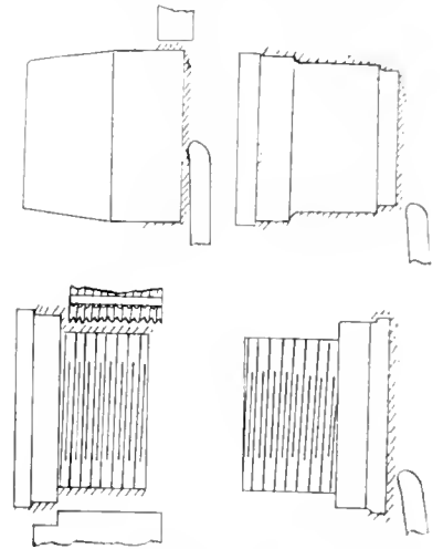
FIG. 15. OUTLINE OF OPERATIONS ON ADAPTER.
