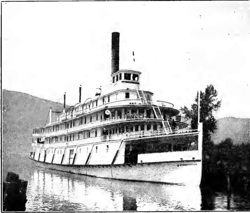
C.P.R. WESTERN LAKE STEAMER "BONNINGTON," BUILT BY POLSON IRON WORKS, TORONTO.
