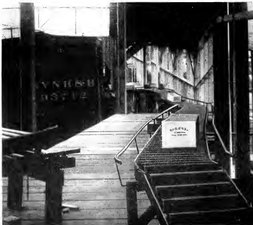
FIG. 2. SYSTEM OF STEEL BALL-BEARING GRAVITY BOX CARRIERS LOADING CARS.
