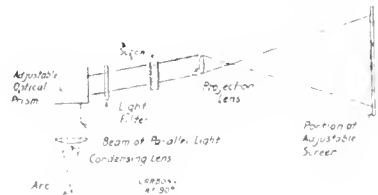
FIG. 6. PRINCIPLE OF THE OPTICAL PROJECTION APPARATUS.
