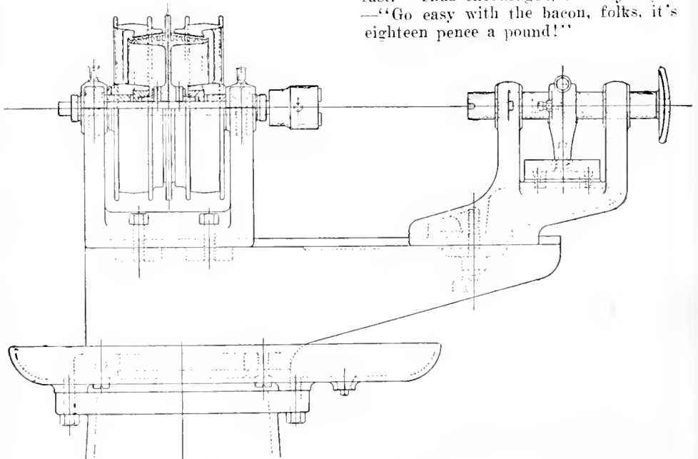
ELEVATION SHOWING DETAILED CONSTRUCTION OF TAPPING MACHINE.
