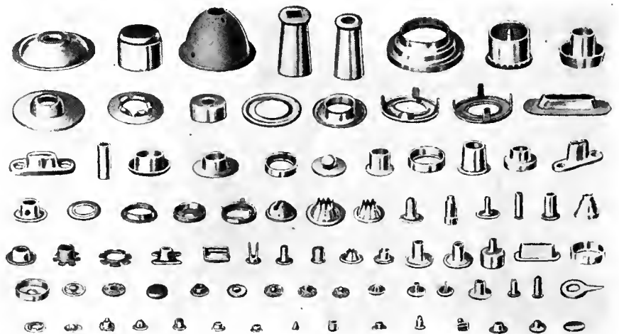
SPECIMENS OF WORK PRODUCED ON MULTIPLE PLUNGER PRESS.
