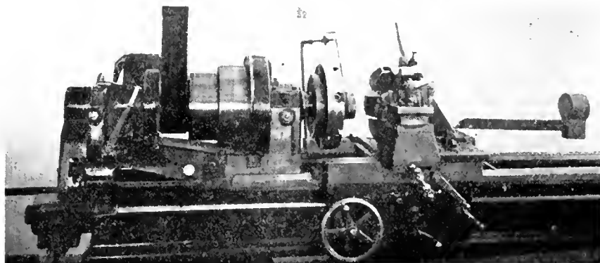
FIG. 14. SPECIAL ATTACHMENT FOR FINISHING ADAPTERS.
