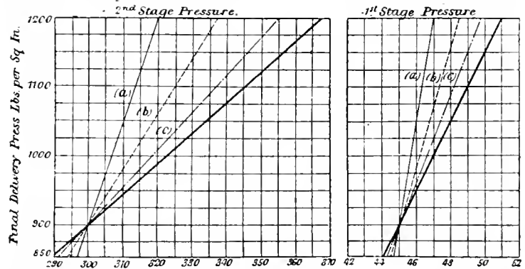
FIG. 10. DIAGRAM SHOWING APPROXIMATELY THE STAGE PRESSURES ATTAINED WHEN THE COMPRESSOR IS DELIVERING AGAINST DIFFERENT FINAL PRESSURES.
