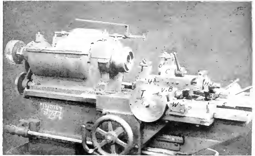
SPECIAL TURNING AND THREADING EQUIPMENT FOR 8-INCH H.E. SHELL ADAPTERS.
