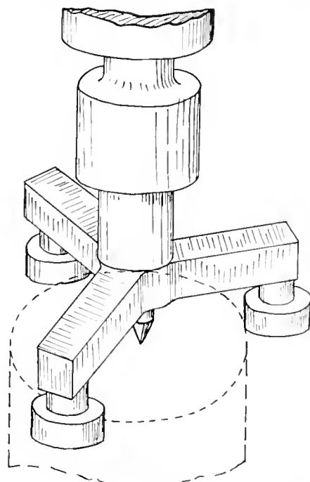
RE-CENTERING DEVICE FOR BASES OF 8-IN. SHELLS.
