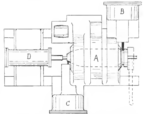
FIG. 4 PLAN OF CUTTING-OFF MACHINE SHOWING FEED AND EJECTOR CYLINDERS.
