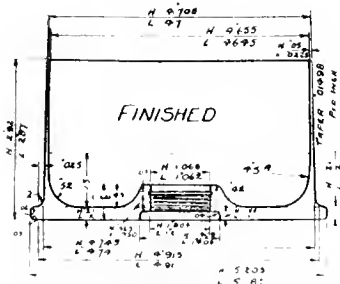
SKETCH OF BRASS CARTRIDGE CASE FOR 4.5 INS. SHELL.
