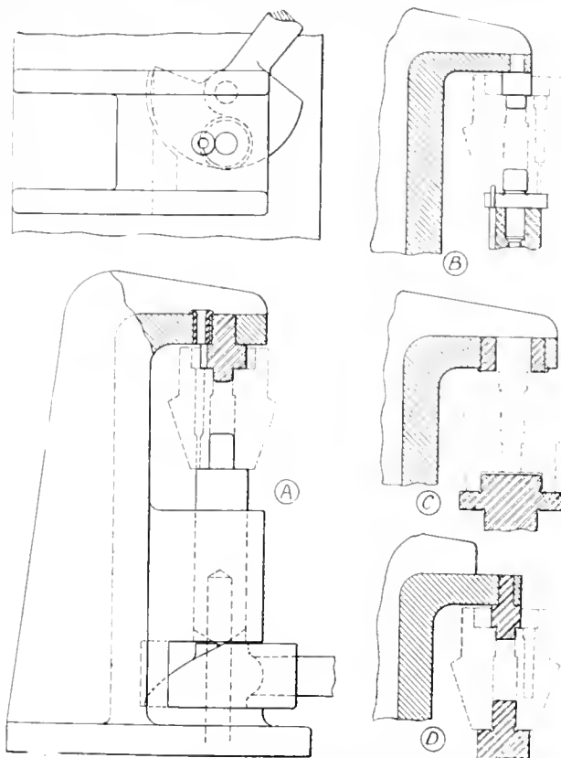
FIG. 6. FIXTURE FOR DRILLING AND COUNTERBORING FUSE HOLES.
