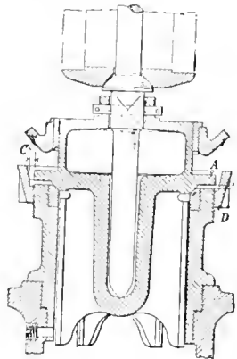
FIG. 4. RECENT TYPE OF MARINE SAFETY VALVE.
