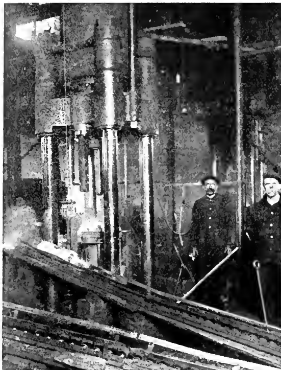
500-TON, 6-INCH SHELL FORGING PRESS WITH GRAVITY CARRIER IN FRONT.
