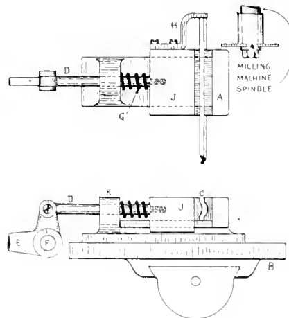
CUTTING OFF STOCK IN THE MILLER.
