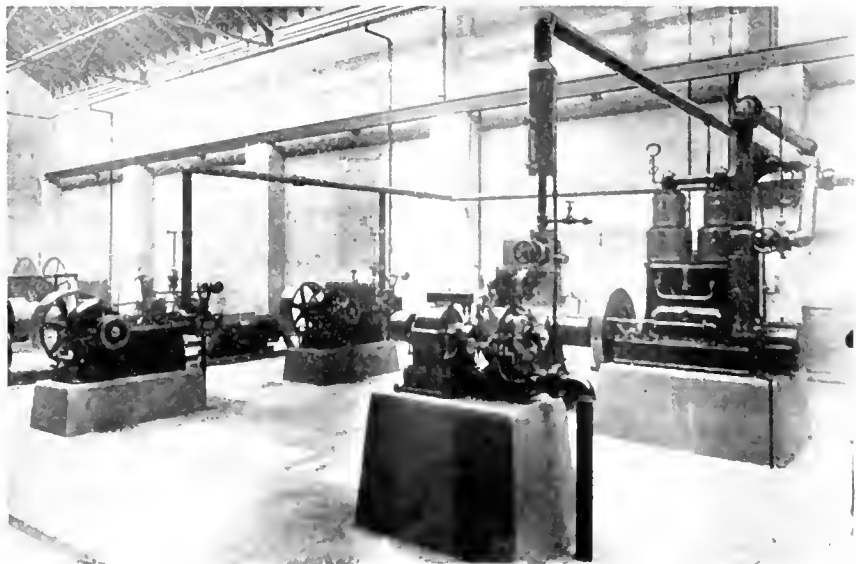
THERMODYNAMIC LABORATORY. THE LAVAL STEAM TURBINE WITH WILLIAMS VERTICAL AND LEONARD HORIZONTAL ENGINES IN BACKGROUND
