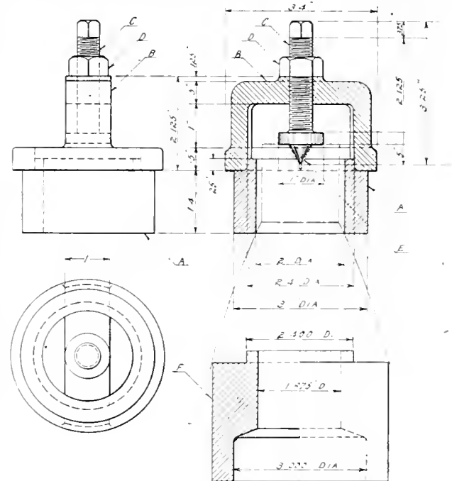
FIG. 8. GAUGE FOR DEPTH OF HOLE IN NOSE.
