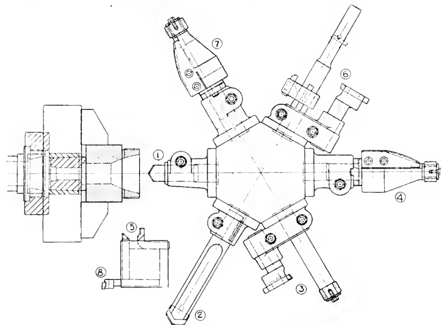
FIG. 2. TOOL LAYOUT FOR FIRST OPERATION.
