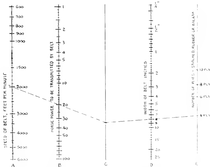
HORSE-POWER WIDTH CHART FOR FABRIC BELTS
