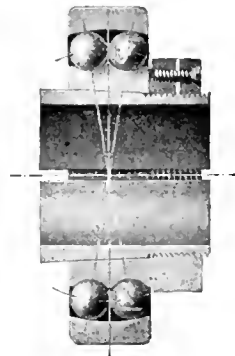
SECTIONAL VIEW, ADAPTER BEARING.
