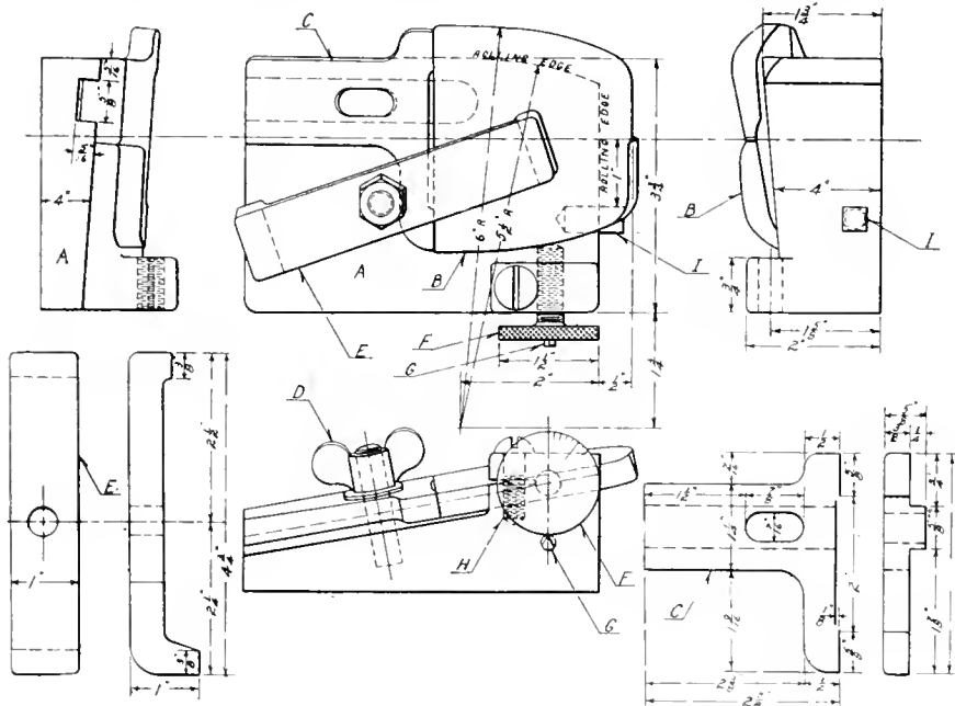
FIG. 2. GRINDING PROFILE CUTTERS.
