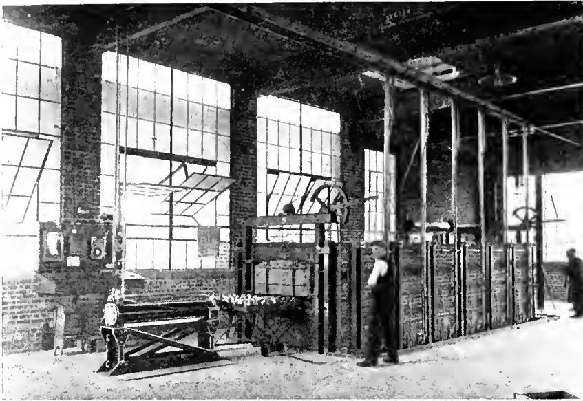
TYPICAL "ROCKWELL" 6-BURNER ANNEALING FURNACE INSTALLED, SHOWING PAN LOADED WITH CASES BEING FED INTO FURNACE BY AIR PUSHER. DUPLICATE PIPES AT SIDE ARE FOR FUEL OIL OR NATURAL GAS.
