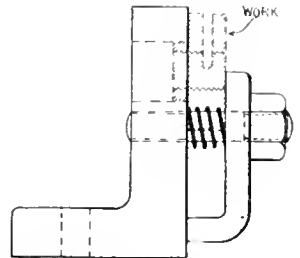
FIGS. 3 AND 4. FIXTURE FOR SLITTING HEXAGONAL NUTS.
