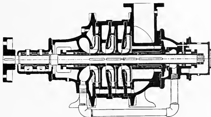
FIG. 12. MODERN FORM OF TURBINE PUMP (MATHER & PLATT).
