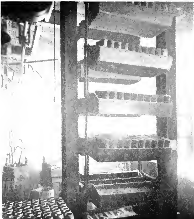
FIG. 11. SPECIAL CONVEYOR IN CONNECTION WITH SHELL NOSE ANNEALING OPERATION.
