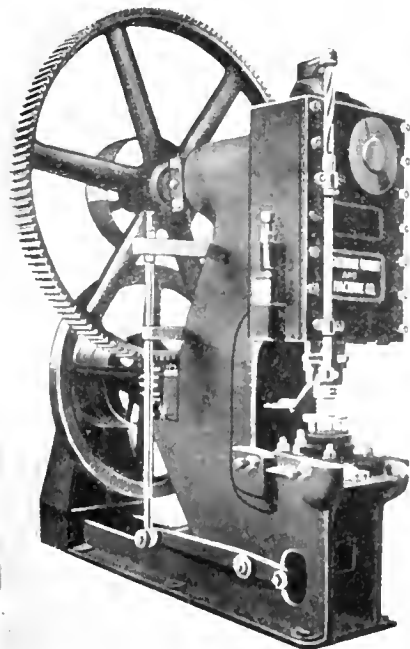
WASHER STAMPING PRESS.
