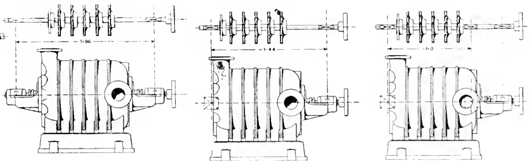
FIG. 30b. FIG. 30a. FIG. 30c. SPAN OF BEARINGS THREE ARRANGEMENTS.
