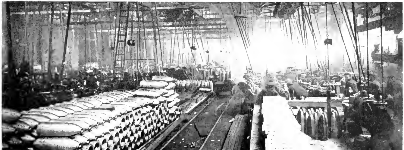
GENERAL VIEW OF SHOP LAYOUT FOR MACHINING THE 9.2 INCH HIGH EXPLOSIVE SHELL.
