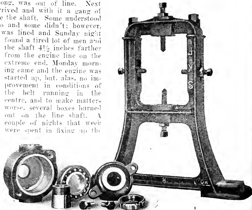
HANGER AND BOX, SHOWING BOX DISASSEMBLED
