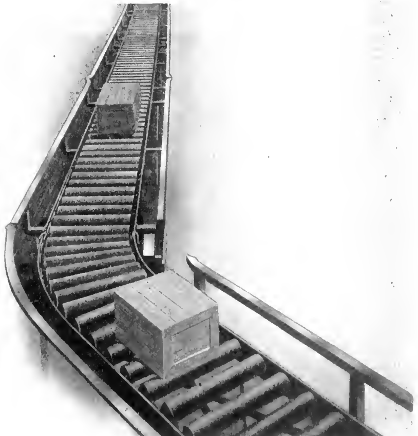
FIG. 1. STEEL BALL-BEARING GRAVITY ROLLER BOX CARRIER OF 1% GRADE.
