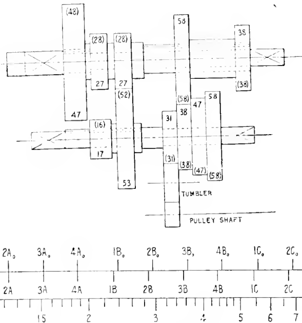
FIG. 12. DIAGRAM OF DRIVING GEAR OF A WELL-KNOWN MAKE OF MILLING MACHINE.
