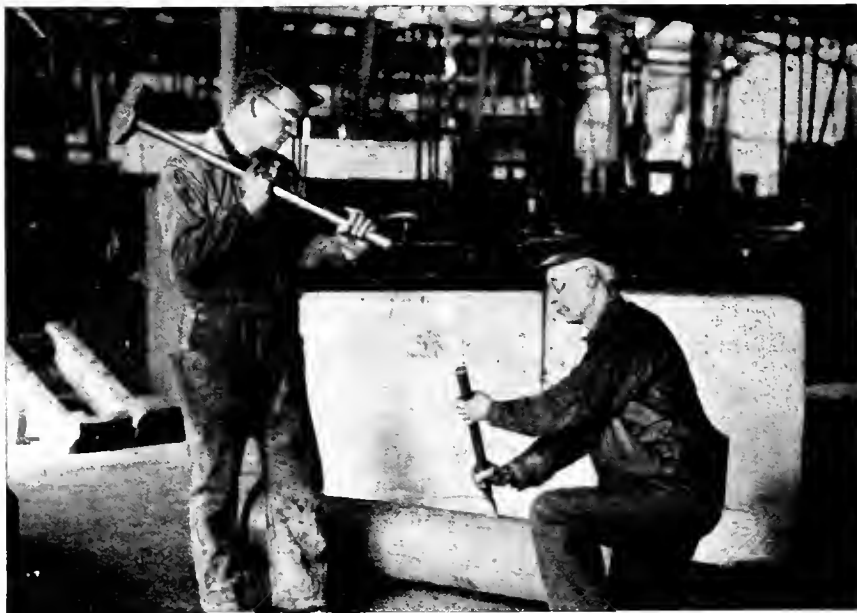
FIG. 37. WORKMEN CUTTING OUT RIVETS AND USING SHIELD. NOTE THAT GOGGLES ARE BEING WORN.
