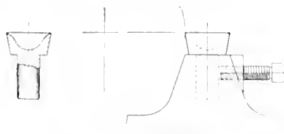
FIG. 6. AUTHOR'S SMALL ANGLE TOOL AND TOOL HOLDER.
