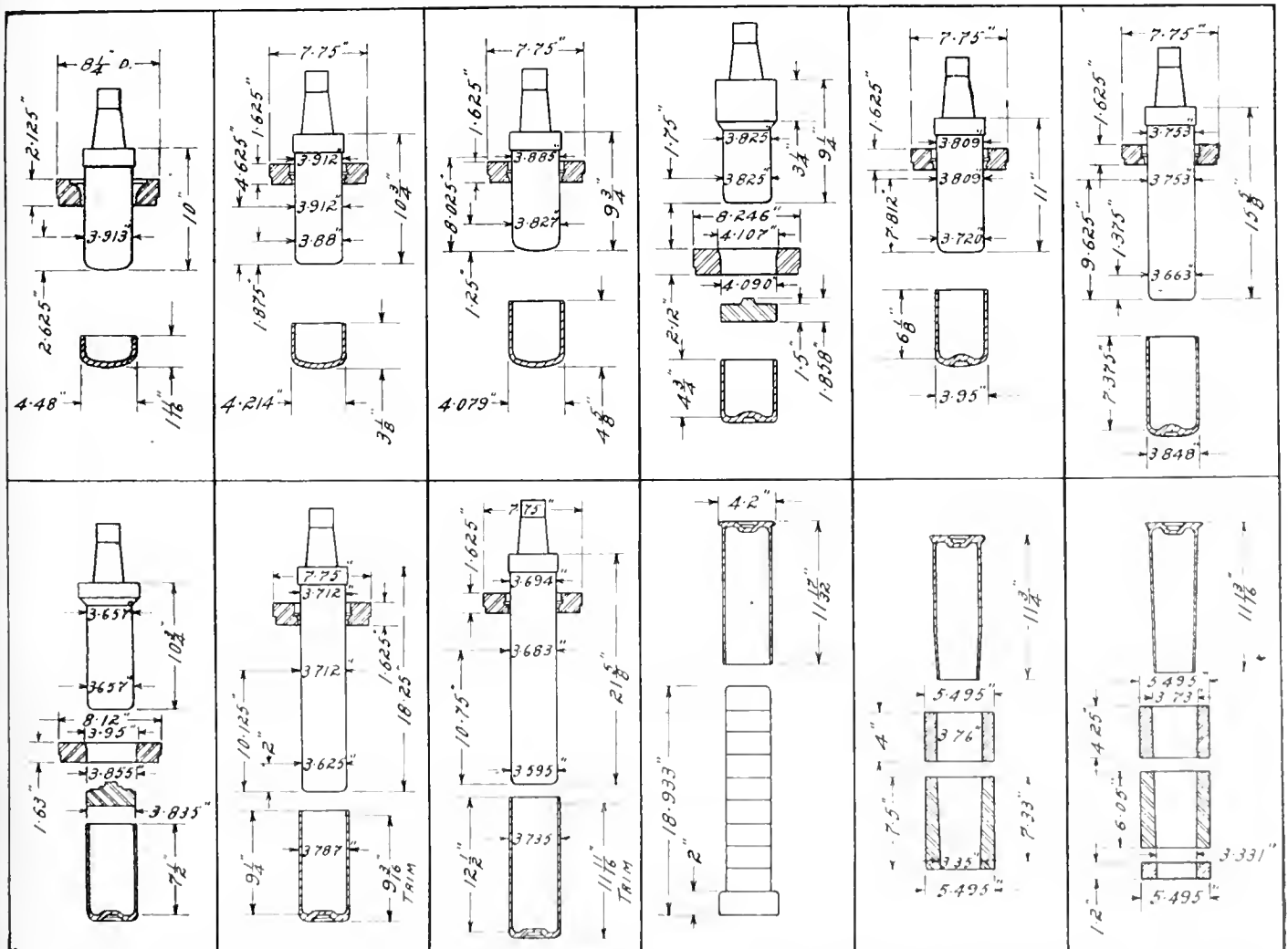
DIAGRAM SHOWING 18-PR. CARTRIDGE CASES DURING THE VARIOUS STAGES OF MANUFACTURE, ALSO THE DETAIL OF PUNCHES AND DIES REQUIRED FOR EACH OPERATION Top Row, left to right—Cupping, first draw, second draw, first indent, third draw, fourth draw. Bottom Row, left to right—Second indent, fifth draw, sixth draw, heading, first taper, second taper.
