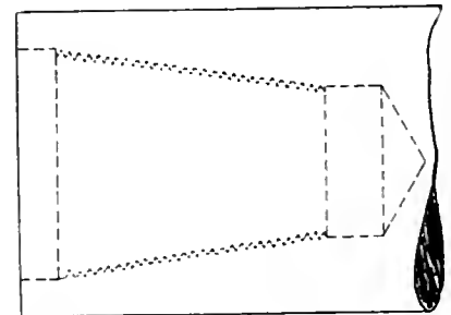
TYPE OF THREAD USED FOR COUPLING OIL WELL TOOLS.
