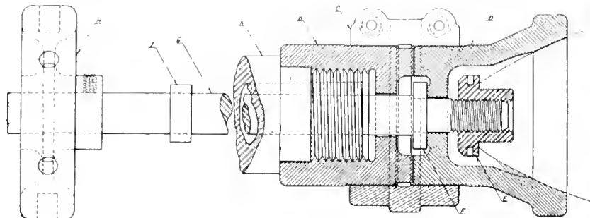
FIG. 12. ASSEMBLY OF DRIVING DEVICE FOR HOB-MILLING BASE.
