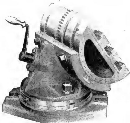
UNIVERSAL ANGLE PLATE WITH WORM ADJUSTING GEAR.
