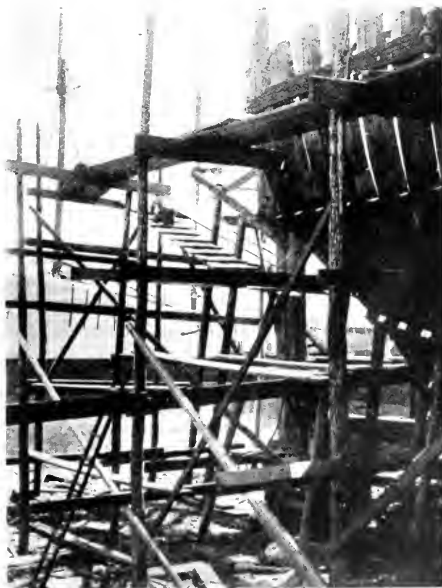
FIG. 3. FOUR DECK STAGING AT STERN OF SHIP. NOTE THE CLEARED RIN'WAY LEADING FROM THE THIRD TO THE FOURTH STAGING
