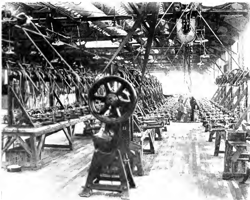
BATTERIES OF MILLING MACHINES WHICH FORM THE GROOVES IN TWIST DRILLS.
