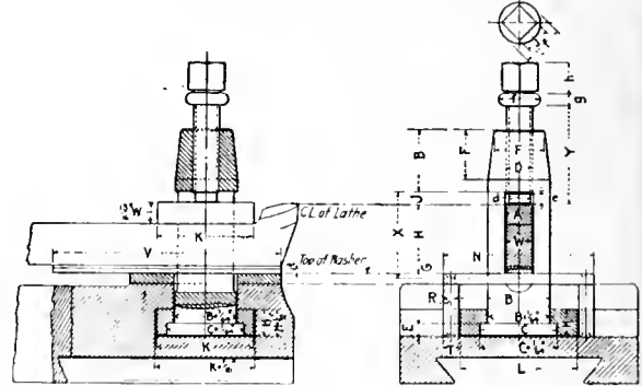
FIG. 13. PROPORTIONS USED BY AUTHOR FOR THE SWIVEL FORM OF TOOL POST FOR MODERATE-SIZED LATHES.
