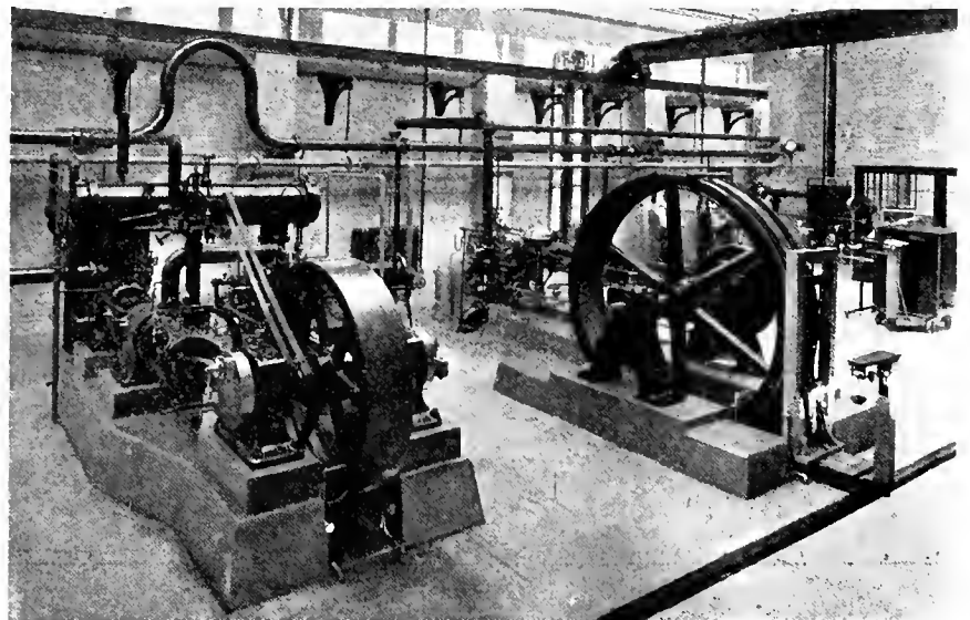
THERMODYNAMIC LABORATORY—CANADIAN RAUD AIR COMPRESSOR AND BROWN STEAM ENGINE.
