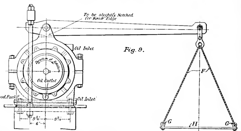
TESTING EQUIPMENT OF MICHELL JOURNAL BEARING.
