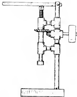
THREE DOLLAR SENSITIVE DRILL.
