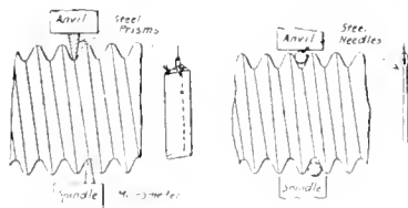
FIG. 5. METHOD OF MEASURING THE CORE DIAMETER AND EFFECTIVE DIAMETER BY MEANS OF A FLOATING MICROMETER.
