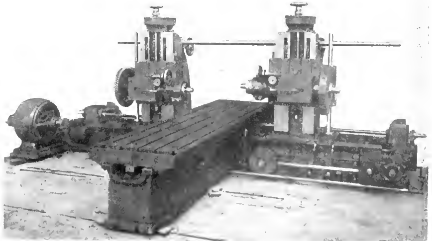
DUPLEX MILLING MACHINE WITH SPECIAL POWER CONTROL, BRACED UPRIGHTS AND SQUARE GIBBED TABLE.
