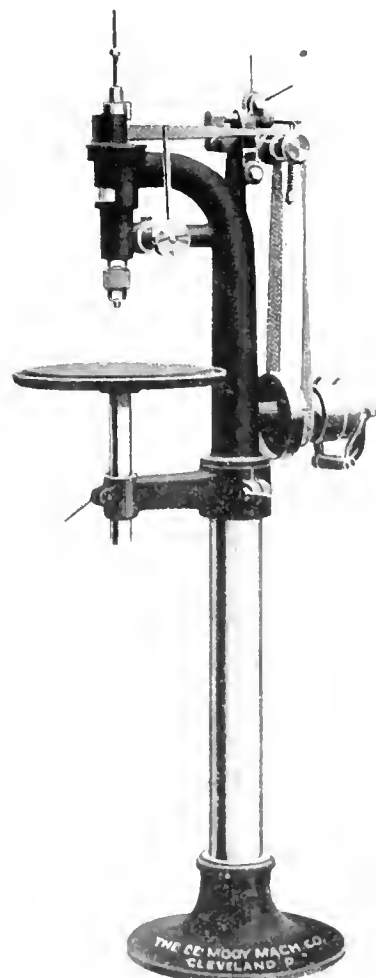
HIGH SPEED BALL BEARING SENSITIVE DRILL.
