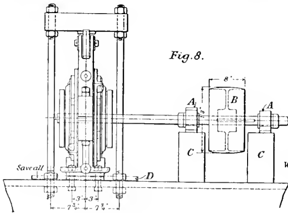
TESTING EQUIPMENT OF MICHELL JOURNAL BEARING.
