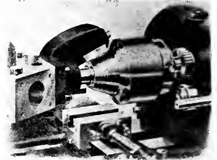
FIG. 4—HERBERT NO. 4 CAPSTAN LATHE ON THIRD OPERATION.
