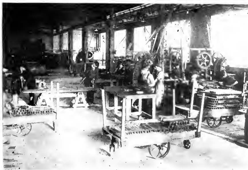
COMPONENT PARTS OF AUTOMOBILE FRAMES IN PROCESS OF MANUFACTURE IN FRAME DEPARTMENT.
