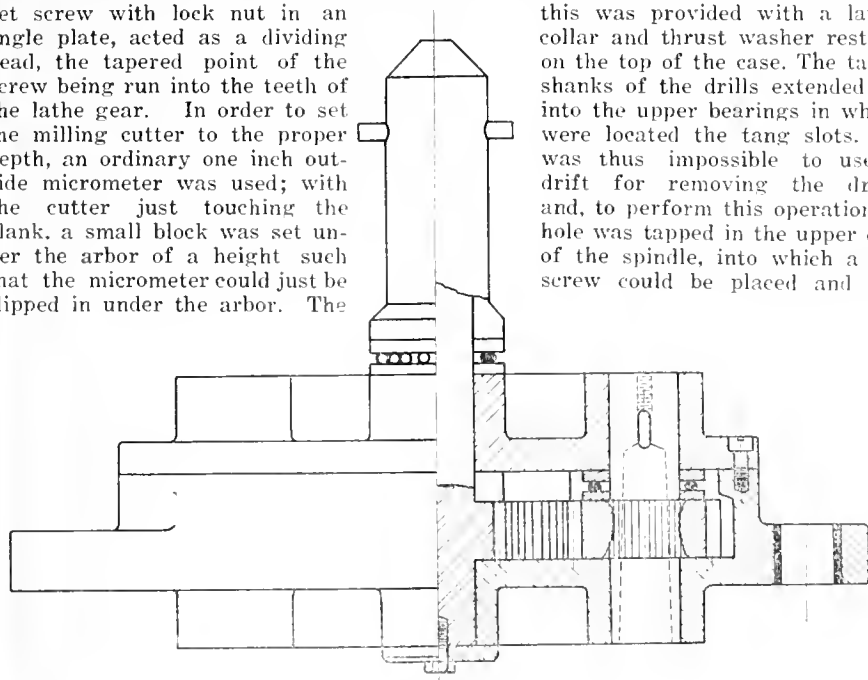
FIG. 3. MULTIPLE DRILL HEADS.
