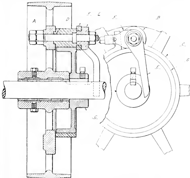
FRICTION CLUTCH FOR COUNTERSHAFT.
