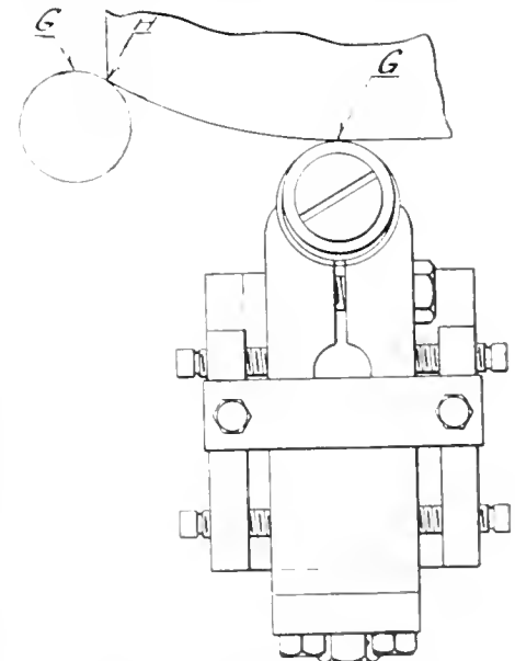
FIG. 2. SPECIAL CIRCULAR TURNING TOOL.
