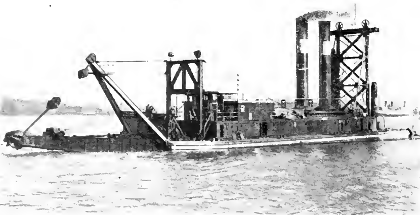
24 INCH HYDRAULIC SUCTION DREDGE BUILT BY POLSON IRON WORKS, TORONTO FOR HARBOR DEVELOPMENT WORK.
