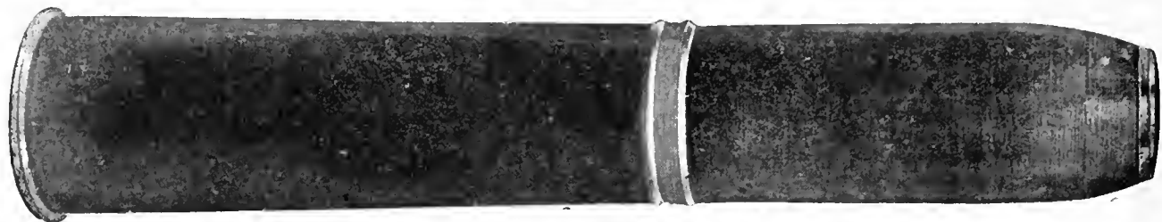
BRASS CARTRIDGE CASE WITH 18-PDR. SHRAPNEL SHELL INSERTED.
