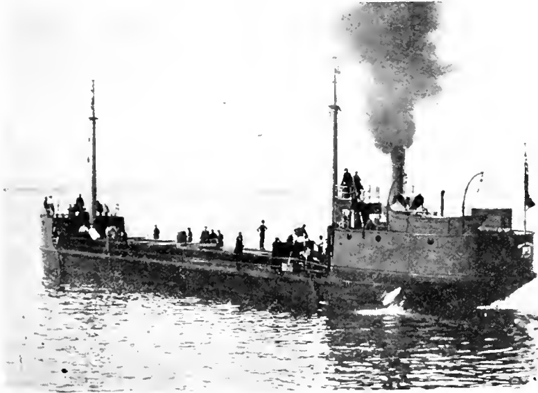
ONE OF THREE LIGHTERS BUILT BY POLSON IRON WORKS, TORONTO, FOR CANADIAN GOVERNMENT SERVICE ON HUDSON BAY.
