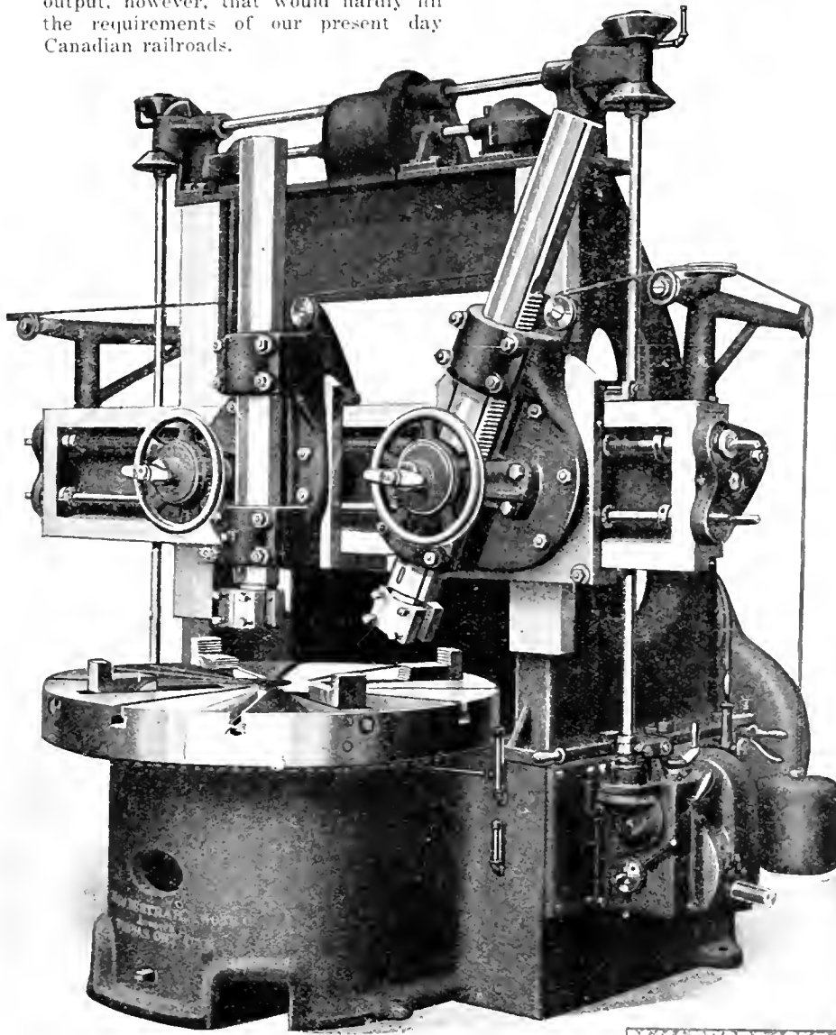
42-INCH VERTICAL BORING AND TURNING MILL.
