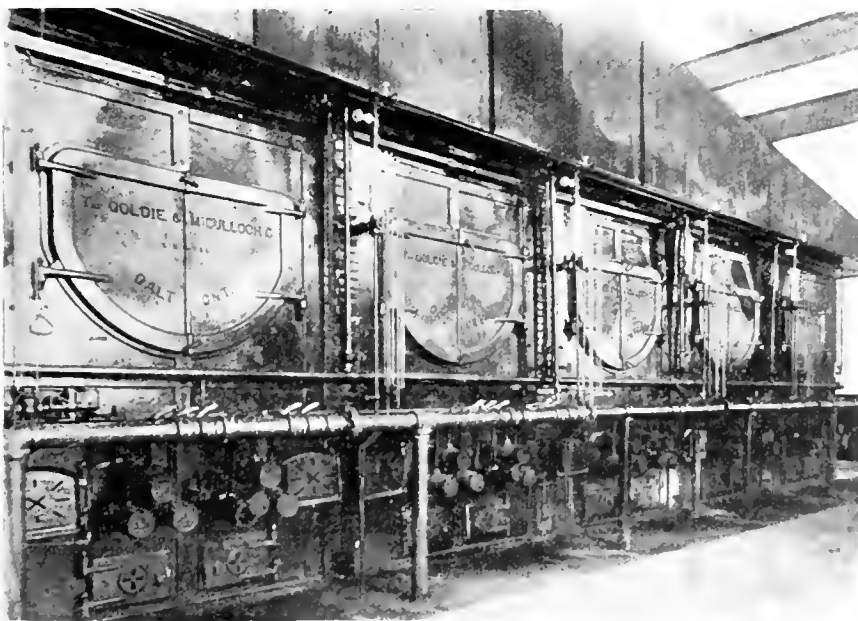
INSTALLATION OF GAS-FIRED BOILERS FOR SUPPLYING STEAM TO THE HAMMERS IN THE FORGE DEPARTMENT.
