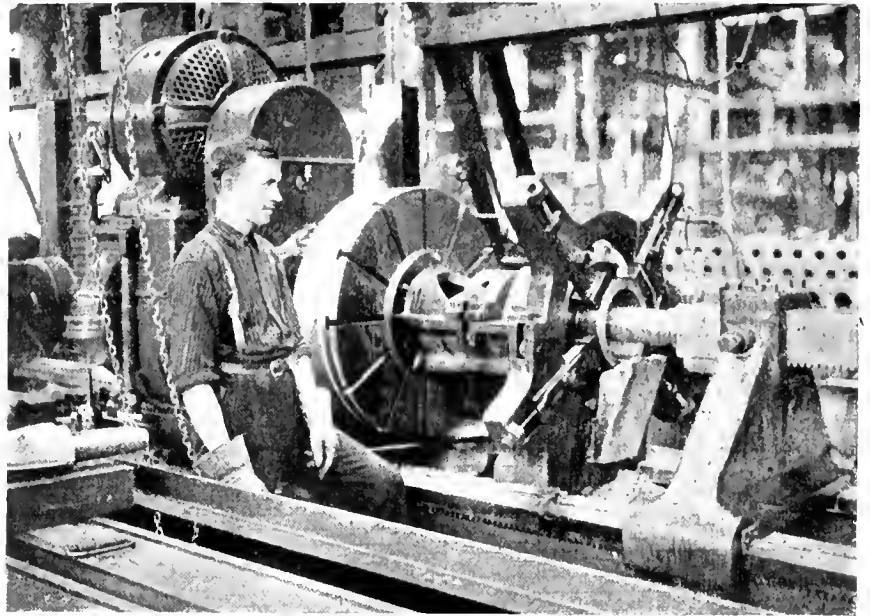
FIG. 6. MACHINING INTERIOR COMPLETE IN SPECIAL BORING LATHIE.
