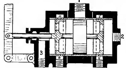
FIG. 2. SECTION OF HYDRAULIC CONTROL VALVE.
