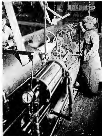
FINISHING PROFILE OF SHELL NOSE. THE CYLINDER IN THE FOREGROUND OPERATES THE RADIAL TOOL-BOX.
