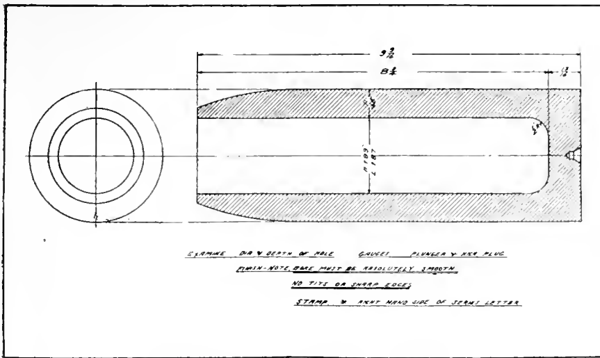
TENTH OPERATION—FINISH BORING.
