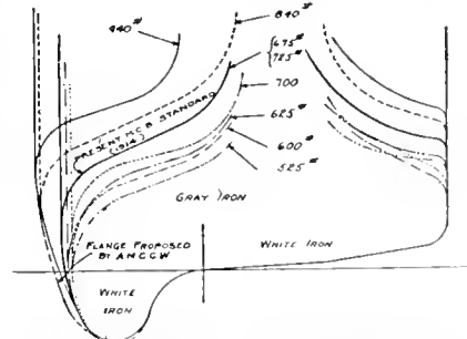
DEVELOPMENT OF FLANGE AND TREAD OF THE CHILLED IRON WHEEL UNDER GROWING REQUIREMENTS.
