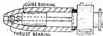
FIG. 8. ARRANGEMENT OF ROUGHING CUTTER BAR FOR RECESSING BASE.
