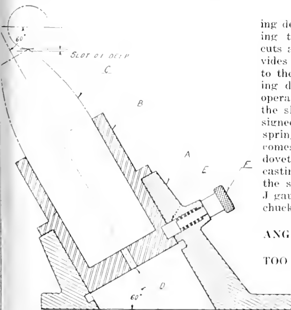
FIG. 1. MILLING SLOTS IN SHELL NOSES.
