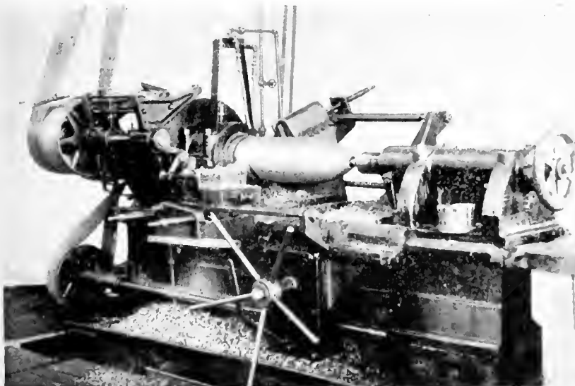
SPECIAL WAVE AND GROOVE MACHINE.
