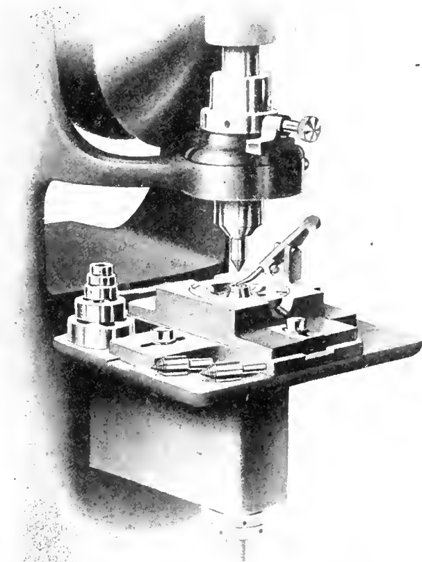
INDEX FINGER, WORK TABLE AND CUTTERS OF DIE MUZZLING MACHINE.
