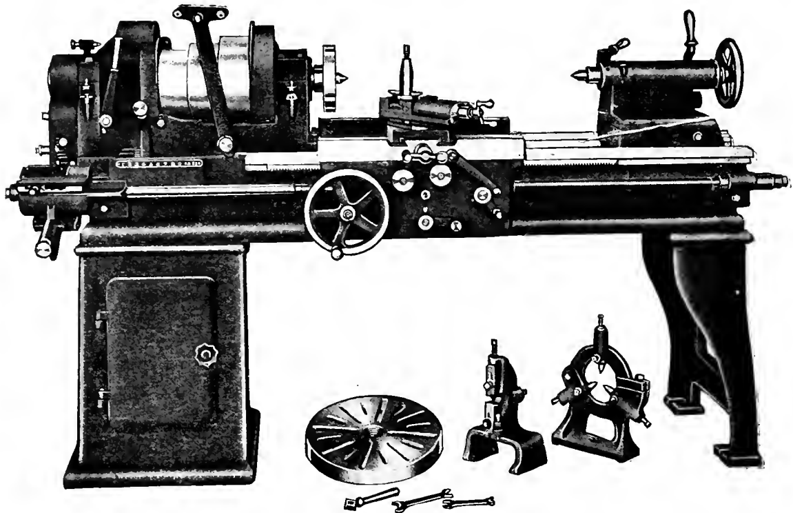
16-INCH QUICK-CHANGE, DOUBLE BACK-GEARED ENGINE LATHE.
