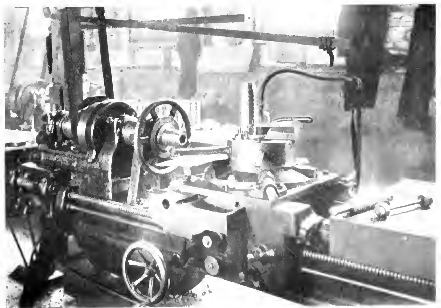
FIG. 5. INSIDE FINISHING OPERATION.
