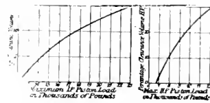
FIG. 12. FIG. 13. Diagram showing effect of clearances on piston loads for a given output at a given pressure.
