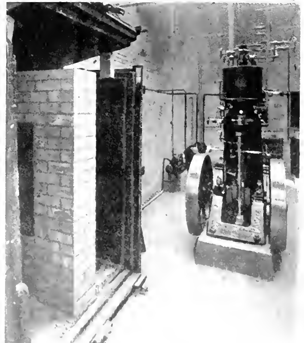
Thermodynamic Laboratory Refrigerating Plant with Test Chamber for Building Materials on Left
