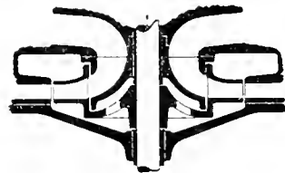
FIGS. 16 AND 17. IMPELLERS BALANCED.
