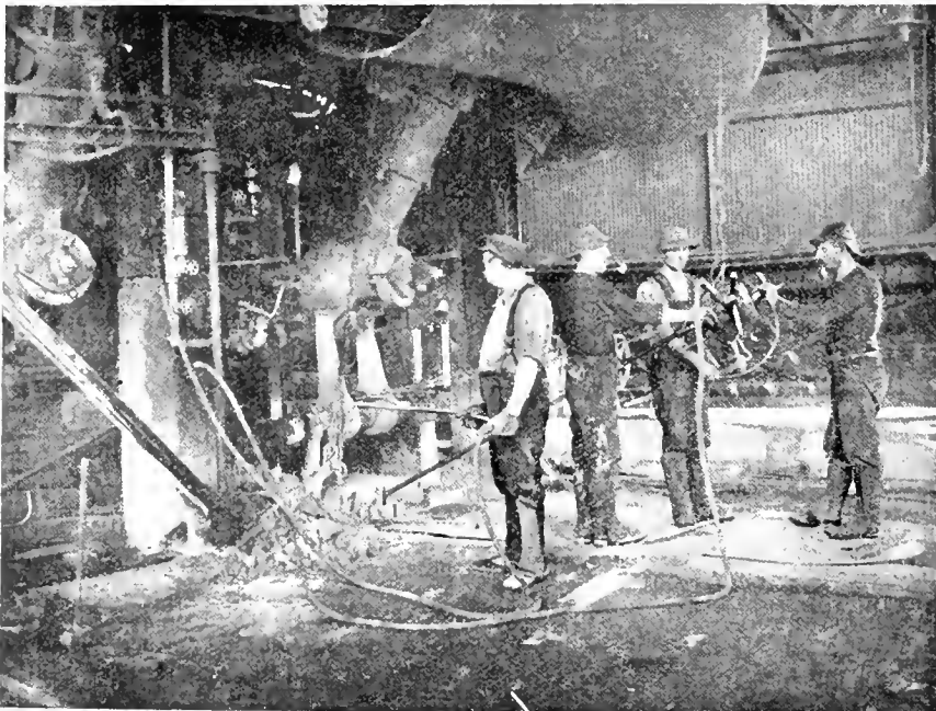
FIG. 14. SAFE METHOD OF DRILLING A TAPPING HOLE.
