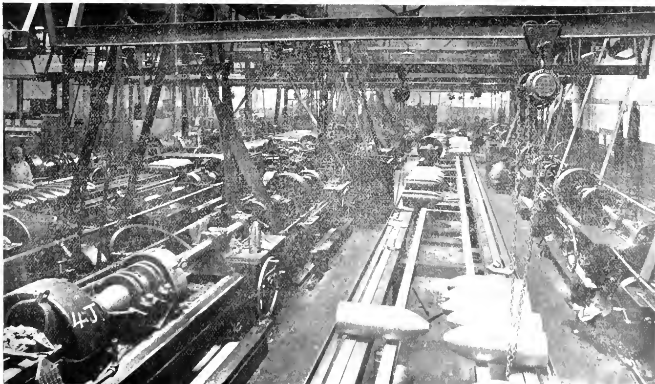
GENERAL VIEW OF "BRIDGEFORD" LATHES ON ROUGH TURNING AND BORING OPERATION—ALSO ARRANGEMENT OF RUNWAYS AND WRIGHT HOISTS FOR EACH LATHE
