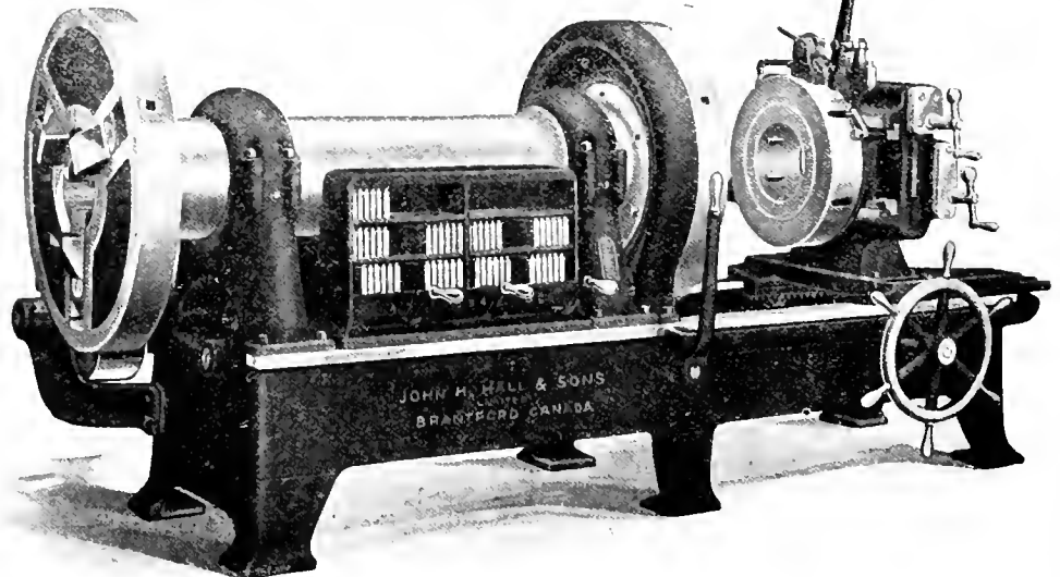
8-IN. PIPE-THREADING MACHINE WITH GEAR BOX DRIVE.
