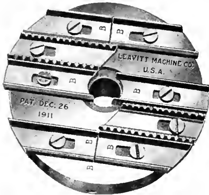
DEXTER IMPROVED TYPE PUMP VALVE CUTTER.
