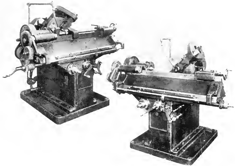
HEAVY DUTY MILLING MACHINE, TRAVELLING TABLE TYPE.
