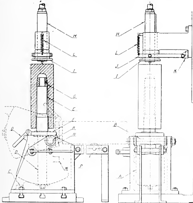
FIG. 1. CENTERING SHELLS.
