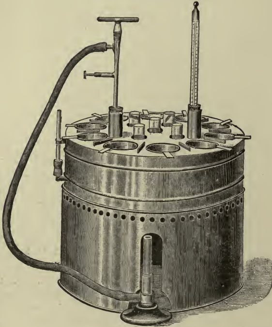
Fig. 15. Paraffine Bath
