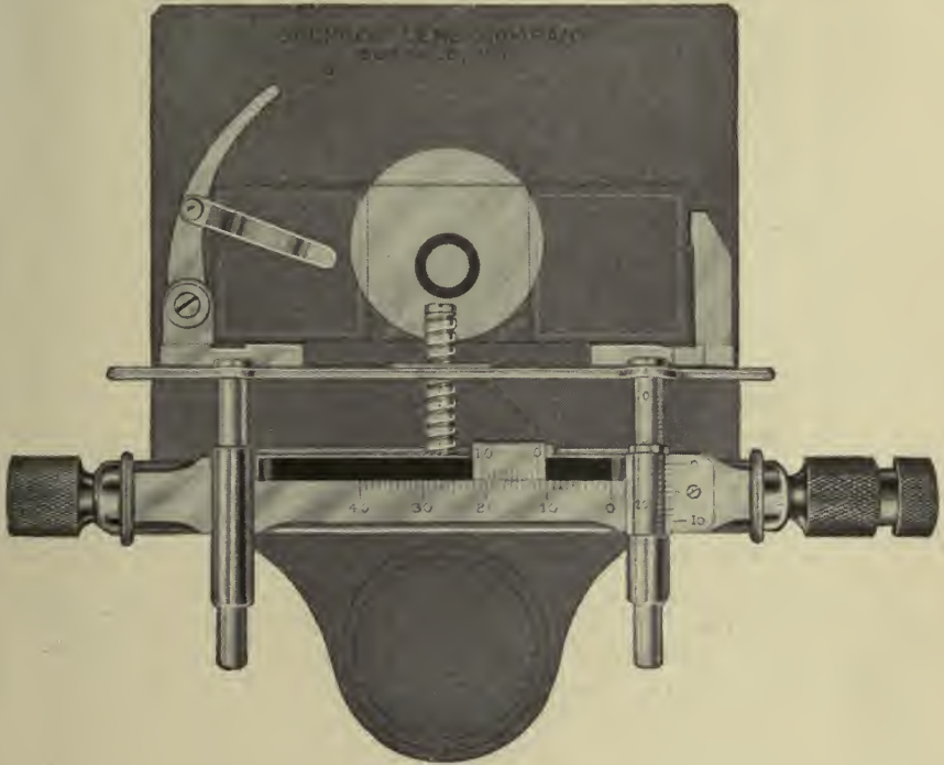
Fig. 2. Mechanical Stage
