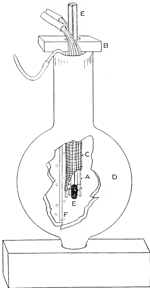
- 16. 4. Details of constant-temperature bath. The tube A, mounted in the block B, and inserted in a bath of warm water in the Dewar flask D, serves as a support for the thermal-junction wires C. The mercury thermometer E is inserted to the depth of the thermal-junctions. The water in the flask is stirred by compressed air entering through the tube F.
