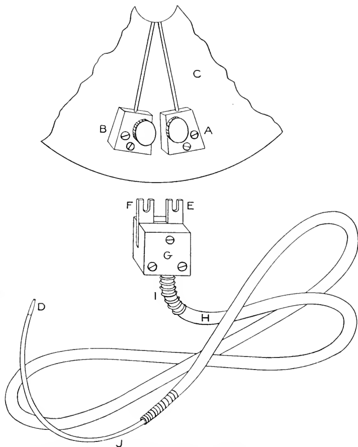
FIG. 8. Detachable thermometer for use inside the calorimeter, with connections. A and E are of constantan; B and F of copper.
