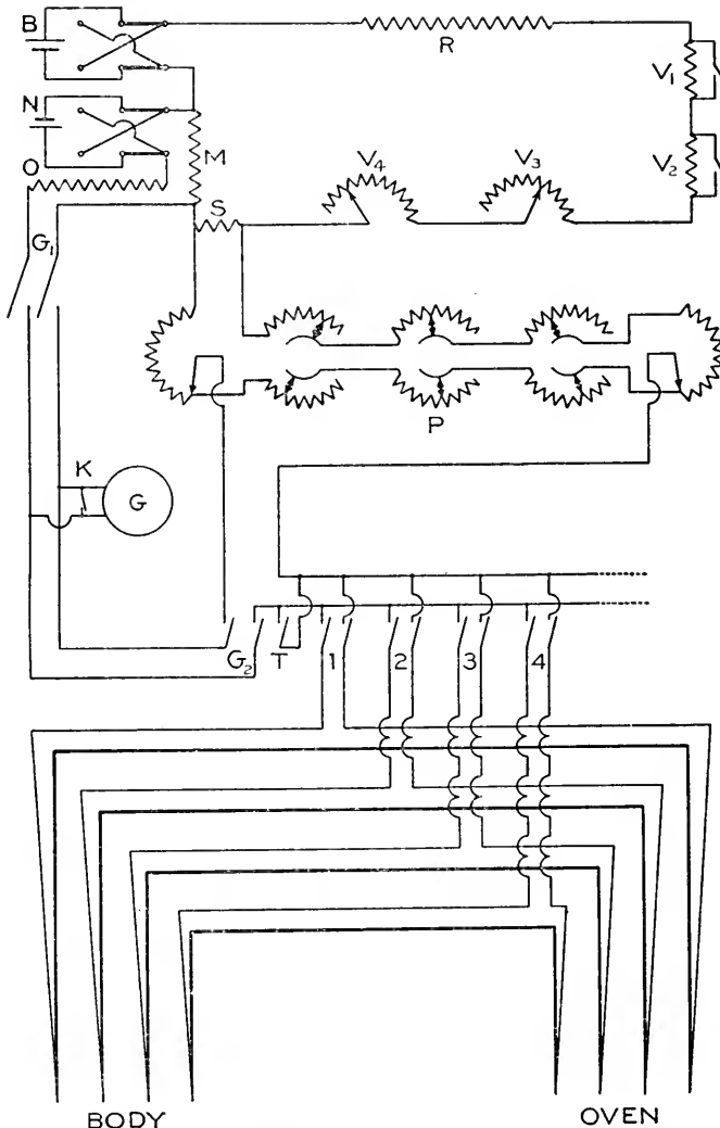
FIG. 2. Complete wiring diagram of apparatus. Current from the battery B flows through the resistances R , V_1 , V_2 , V_3 , and V_4 , and then divides, part flowing through the shunt S and part through the potentiometer P , the total current finally returning to B through the resistance M . The potentiometer, which is composed of 5 variable resistances is joined to the switching arrangement, of which G_2 connects the galvanometer G in circuit, T replaces the thermal-junction system when testing, and 1, 2, 3, 4, etc., are connected to the thermal-junctions at the body and the constant-temperature oven. The constantan wires are indicated by the heavy lines. N is the standard cell, protected by the high resistance O , and connected to the circuit through the double-contact key G_1 . The switch K is for convenience in bringing the galvanometer to rest.
