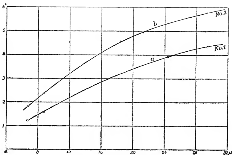
FIG. 19. — Wire-grating calibration.
