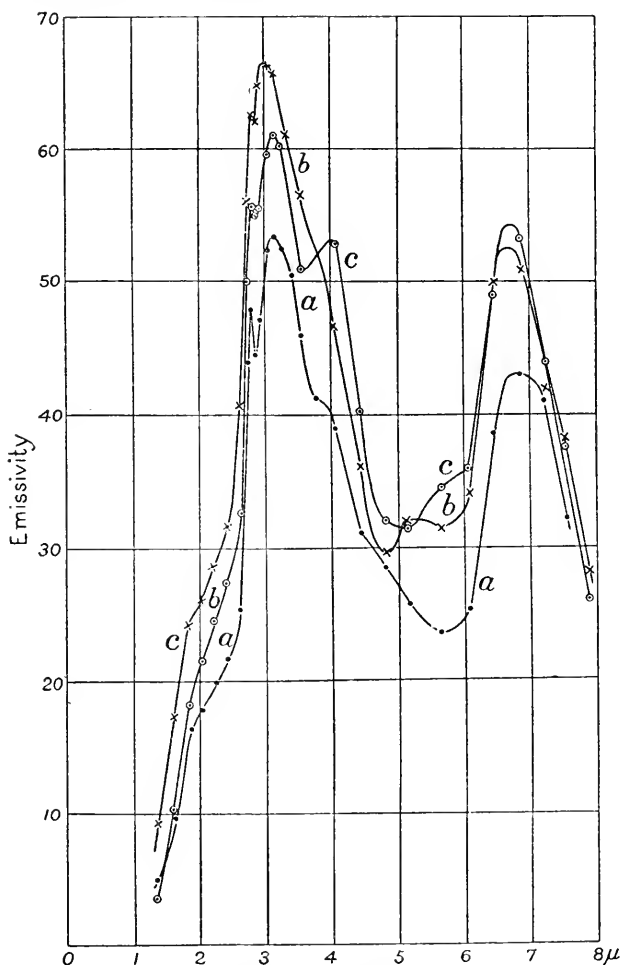
FIG. 84. — Yttrium oxide.
