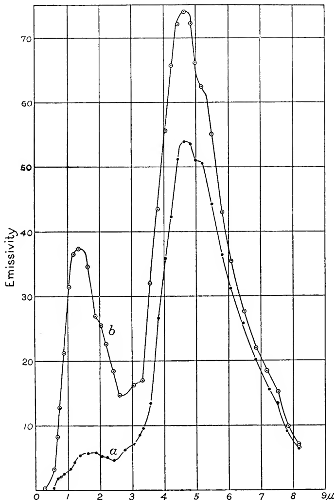
FIG. 76. — Aluminum oxide.
