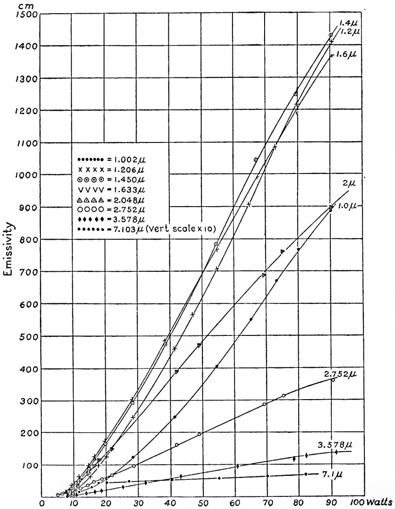
FIG. 95.— Isochromatic radiation curves of Nernst glower.
