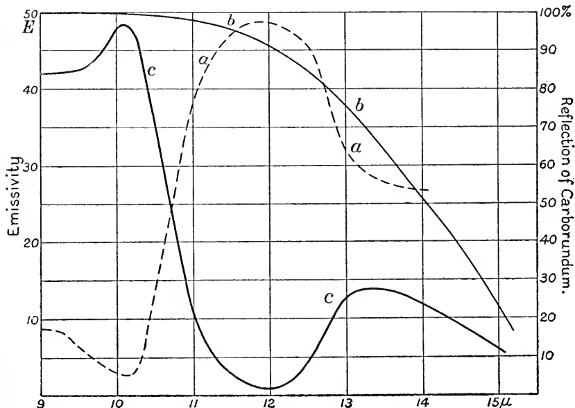
FIG. 99. — Reflection from carborundum (a); Radiation of complete radiator at 300° abs. (b); Radiation from carborundum at 300° abs. (c).
