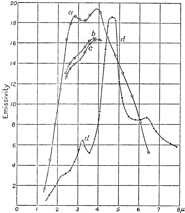
FIG. 90.— Nickel oxide (a), (b), (c); Calcium sulphate.
