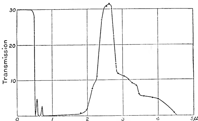
FIG. 38. — Blue-violet glass.
