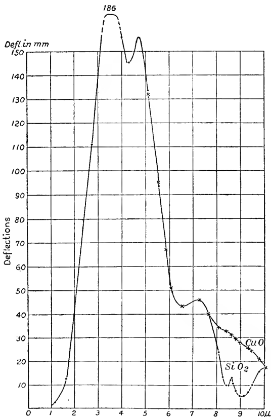
FIG. 98. — Emission spectrum of copper oxide and of quartz, 325° C. (Rosenthal).
