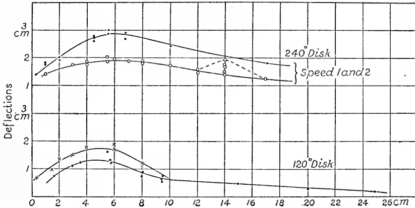
FIG. 105. — Radiation due to rotating sector disk.
