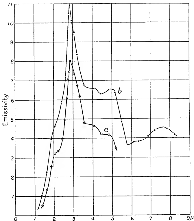
FIG. 85. — Erbium oxide.
