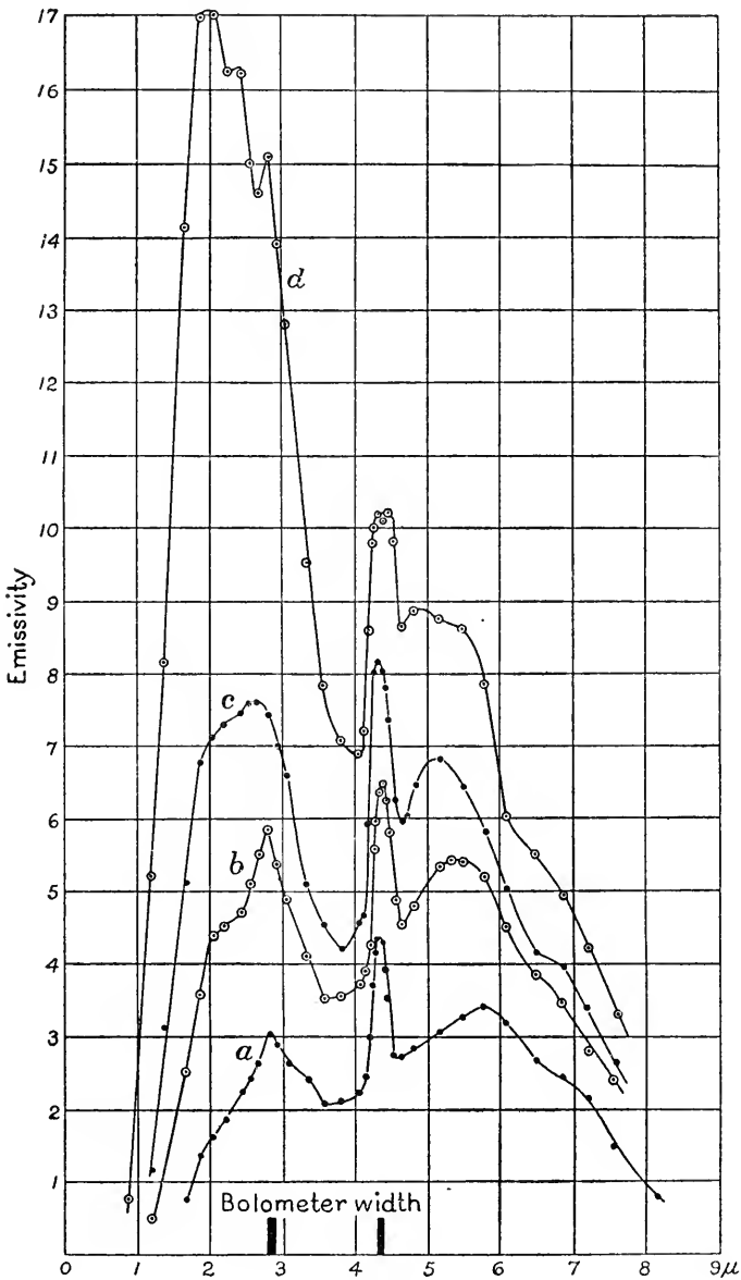
FIG. 77. — Zirconium oxide.
