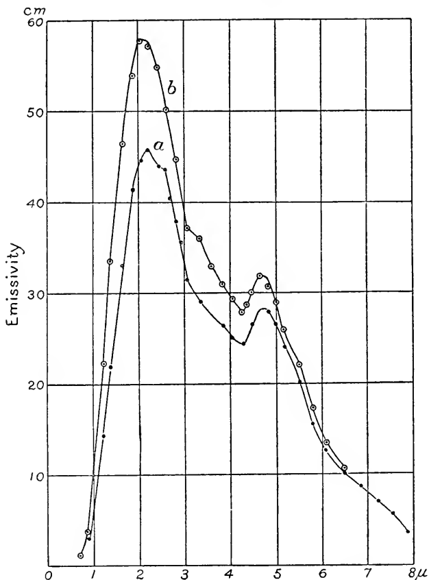
FIG. 67.—Amphibole.
