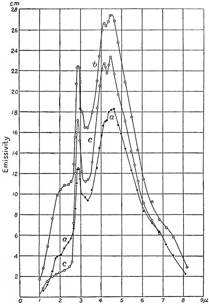
FIG. 66.—Oligoclase.
