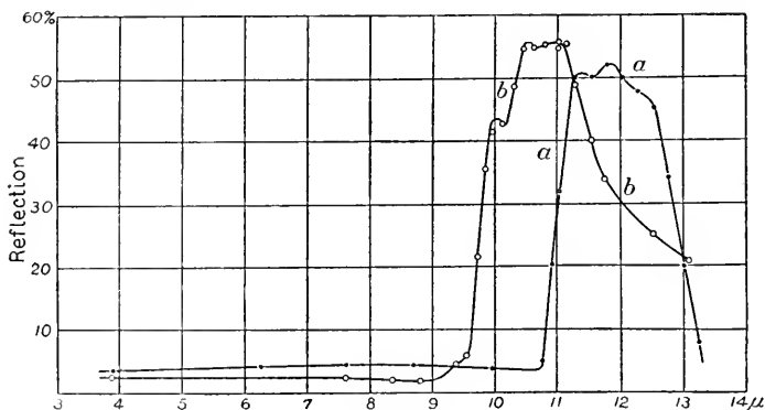
FIG. 8. — Scheelite ( a ); Zircon.
