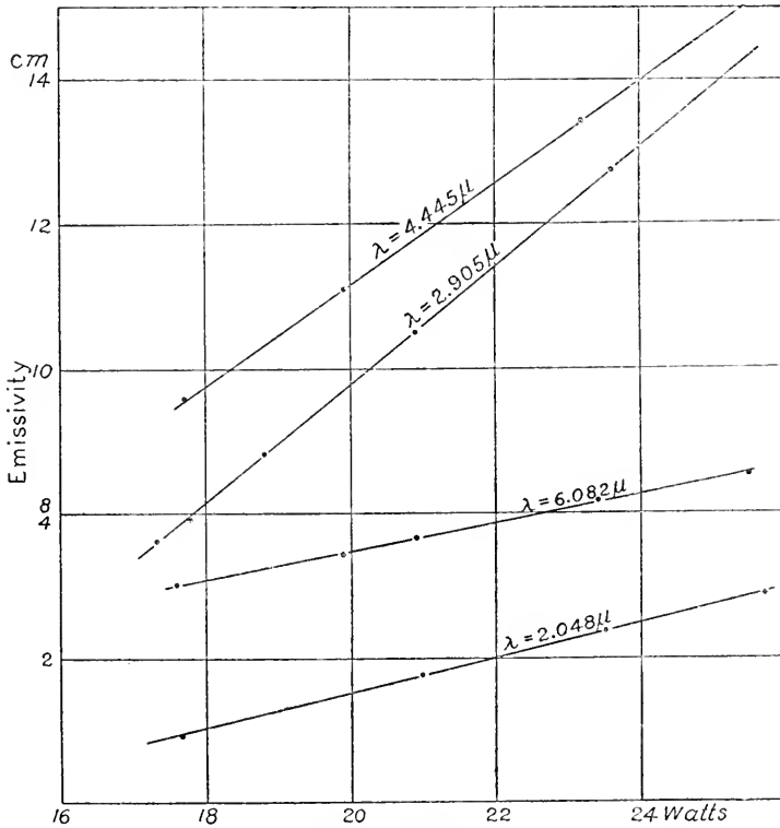
FIG. 96. — Isochromatic radiation curves of oligoclase.
