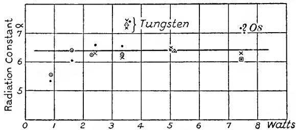
FIG. 61. — Radiation constant ( \alpha ) of osmium.
