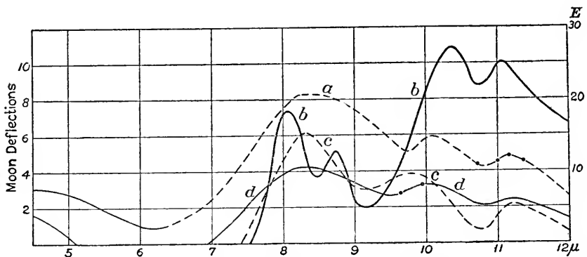
FIG. 103. — Emission of quartz ( b ); Emission from moon (Langley).
