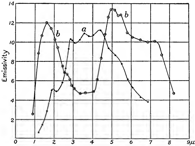
FIG. 70. — Glass (a); Magnesia.
