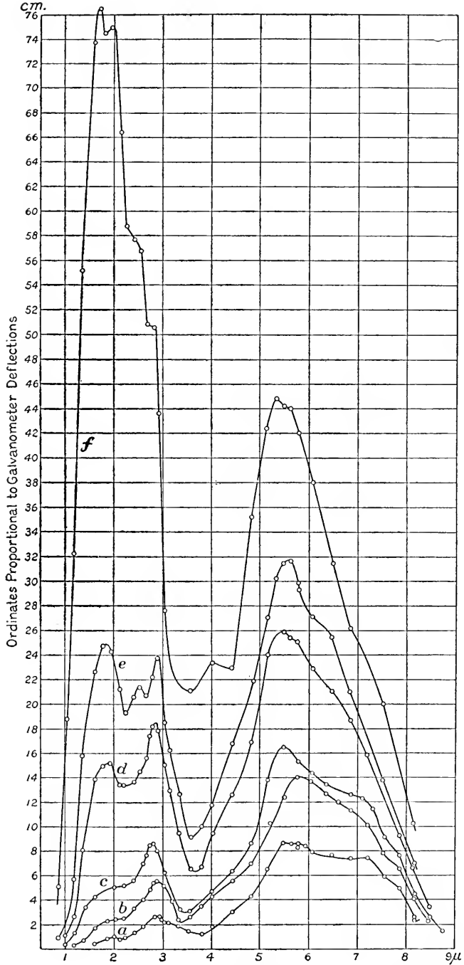
FIG. 57. — Emission spectrum of Nernst glower. a = 2 , b = 3 , c = 4.2 , d = 6.2 , e = 7.1 , and f = 10.6 watts, respectively.
