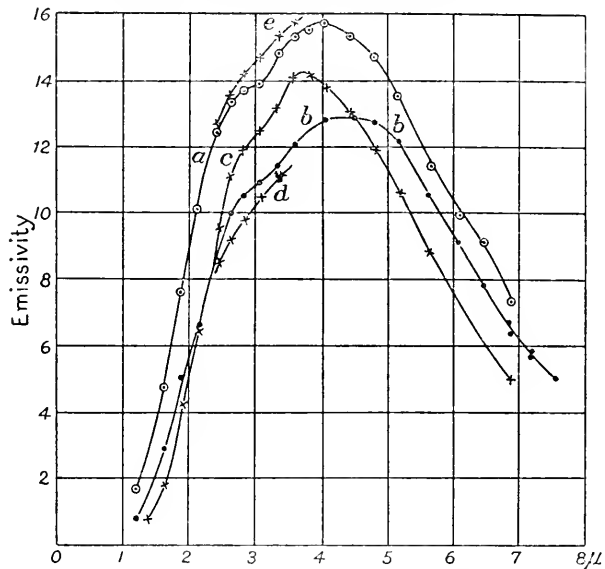
FIG. 88. — Iron oxide, (a) (b); Copper oxide.
