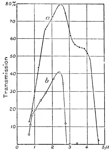
FIG. 41. — Black glass.
