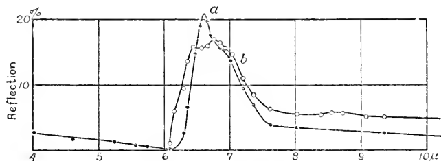
FIG. 5. — Calcite ( a ); Magnesite.
