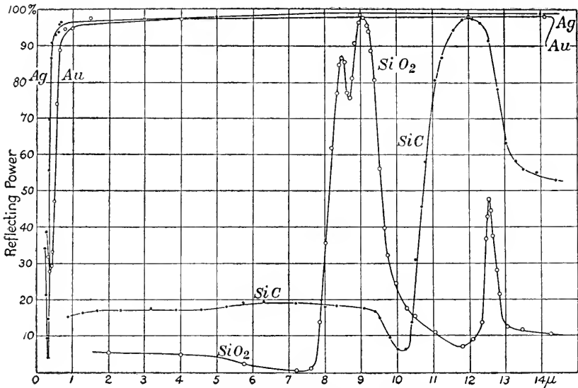
FIG. 24. — Reflecting power; gold, silver, quartz, carborundum.
