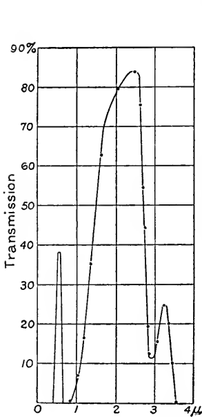
FIG. 39. — Green glass.
