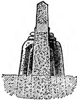
CROSS SECTION OF CISTERN WALL. FROM DAUX.
