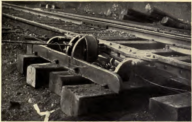
TRACK APPARATUS FOR ASCERTAINING WHEEL AND RAIL PRESSURES.
