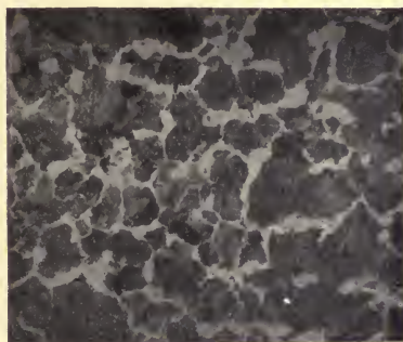
NO. 64. STRUCTURE \frac{1}{2} IN. BELOW TREAD.
