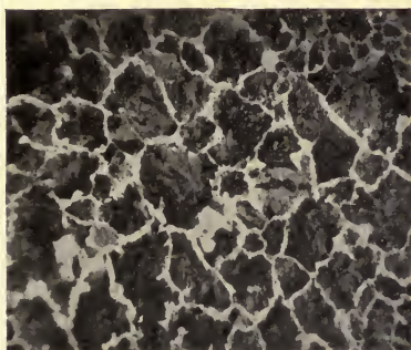
NO. 63. STRUCTURE \frac{1}{8} IN. BELOW TREAD.
