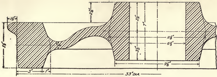
33-IN. STEEL WHEEL.
