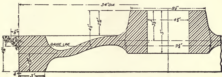
34-IN. WHEEL FOR CITY AND INTERURBAN SERVICE, DESIGNED FOR SANDERSON & PORTER, CONTRACTORS AND ENGINEERS.
