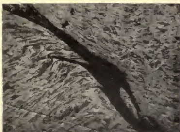
NO. 57. SLAG AT EDGE OF SOLID METAL.
