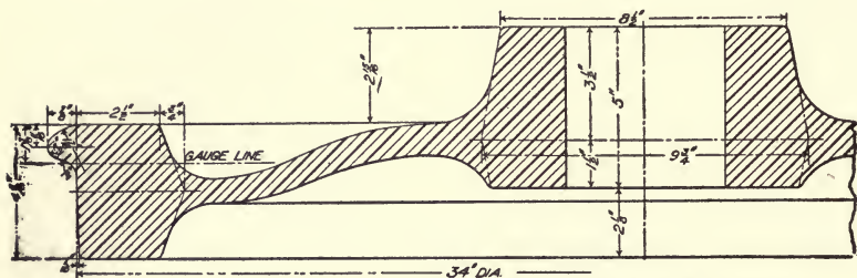
84-IN. STREET-CAR WHEEL FOR PENNSYLVANIA AND MAHONING VALLEY TRACTION CO.
