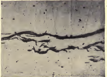
NO. 44. \frac{1}{4} IN. BELOW TREAD OF SOLID METAL.
