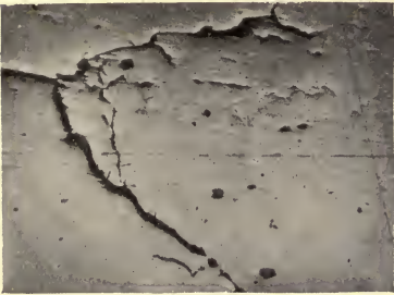
NO. 41. SHOWING SLAG CRACKS.
