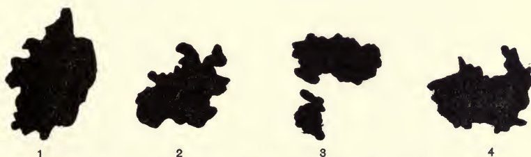
CONTACTS OF 35-IN. STEEL-TIRED WHEEL UNDER CAFÉ CAR. WEIGHT ON WHEEL, 6,075 LBS.
