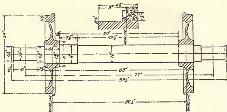
AXLE AND WHEEL DESIGN SUBMITTED BY THE SCHOEN STEEL WHEEL CO. AS REQUESTED BY THE CENTRAL ELECTRIC RAILWAY COMMITTEE ON STANDARDIZATION FROM THEIR REPORT DATED MAY 23, 1807.
