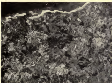
No. 49. AT EDGE OF SHELLED-OUT SPOT.
