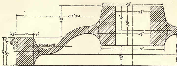
33-IN. WHEEL FOR THE UNITED ELECTRIC RAILWAYS AND ELECTRIC CO. OF BALTIMORE, MD.
