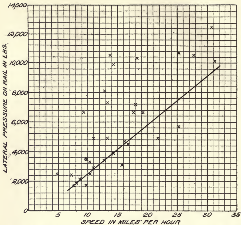
DIAGRAM OF LATERAL THRUST OF LEADING WHEEL OF FORWARD TRUCK OF LOADED COAL CAR. TOTAL WEIGHT, 142,300 LBS., ON 4° 25' CURVE.
