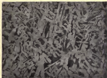
NO. 58. STRUCTURE \frac{1}{2} IN. BELOW TREAD.
