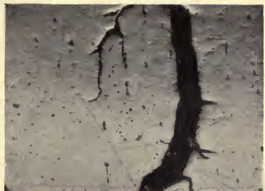
No. 46. SLAG CRACK IN SOLID SECTION OF TIRE.
