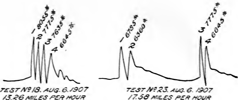
EXAMPLES OF LATERAL THRUST DIAGRAMS OF LOADED COAL CAR. TOTAL WEIGHT, 142,000 LBS., OR 4° 25' CURVE.
