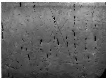
No. 48. MANGANESE BISULPHIDE SPOTS.
