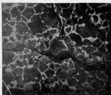
NO. 62. SLAG \frac{1}{4} IN. BELOW SHELLLED OUT SPOT
