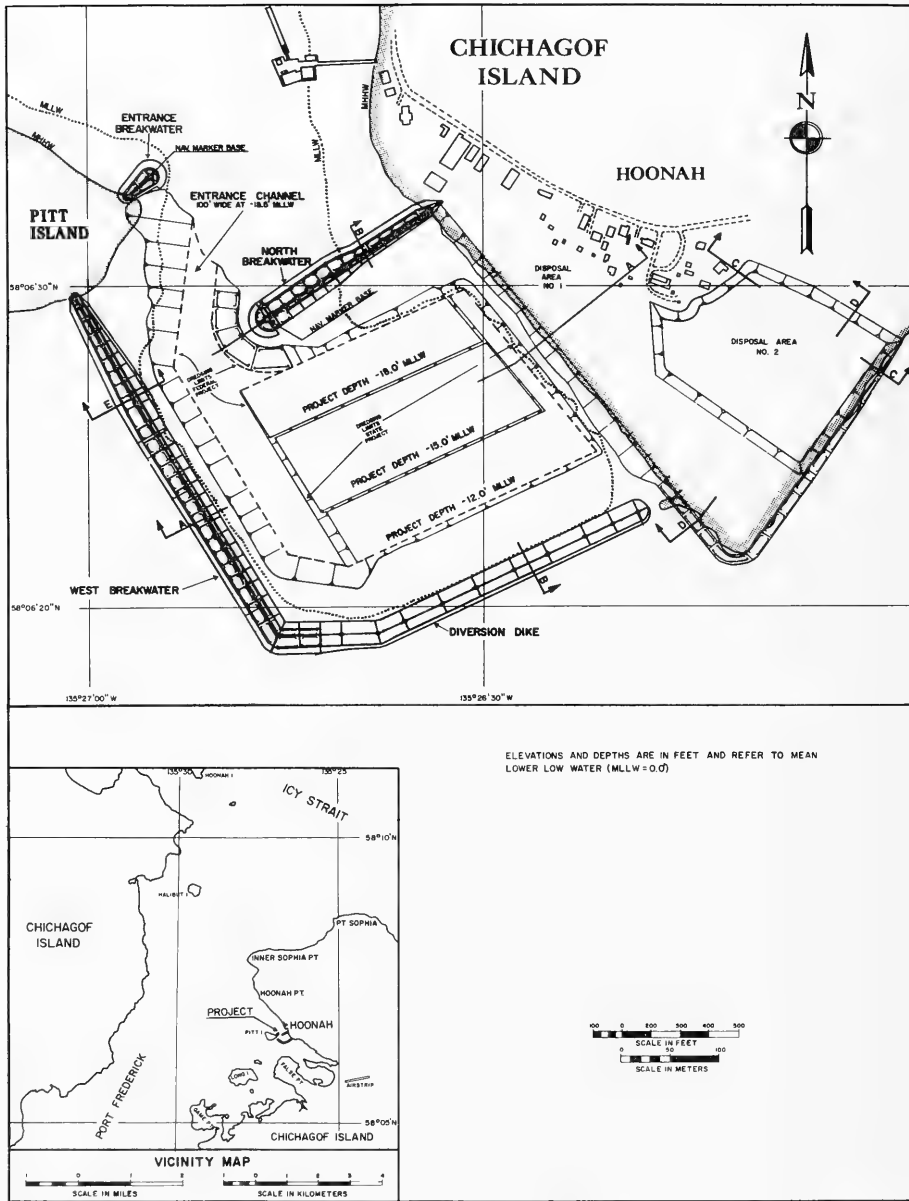
Figure 16. Site layout of Hoonah Harbor, Alaska (revised 1981)
