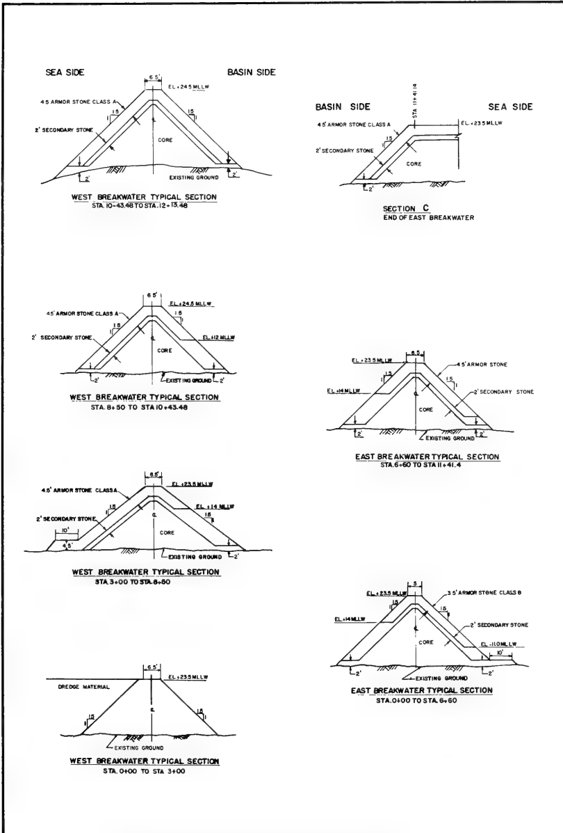
Figure 32. Breakwater cross sections, Metlakatla New Harbor, Alaska
