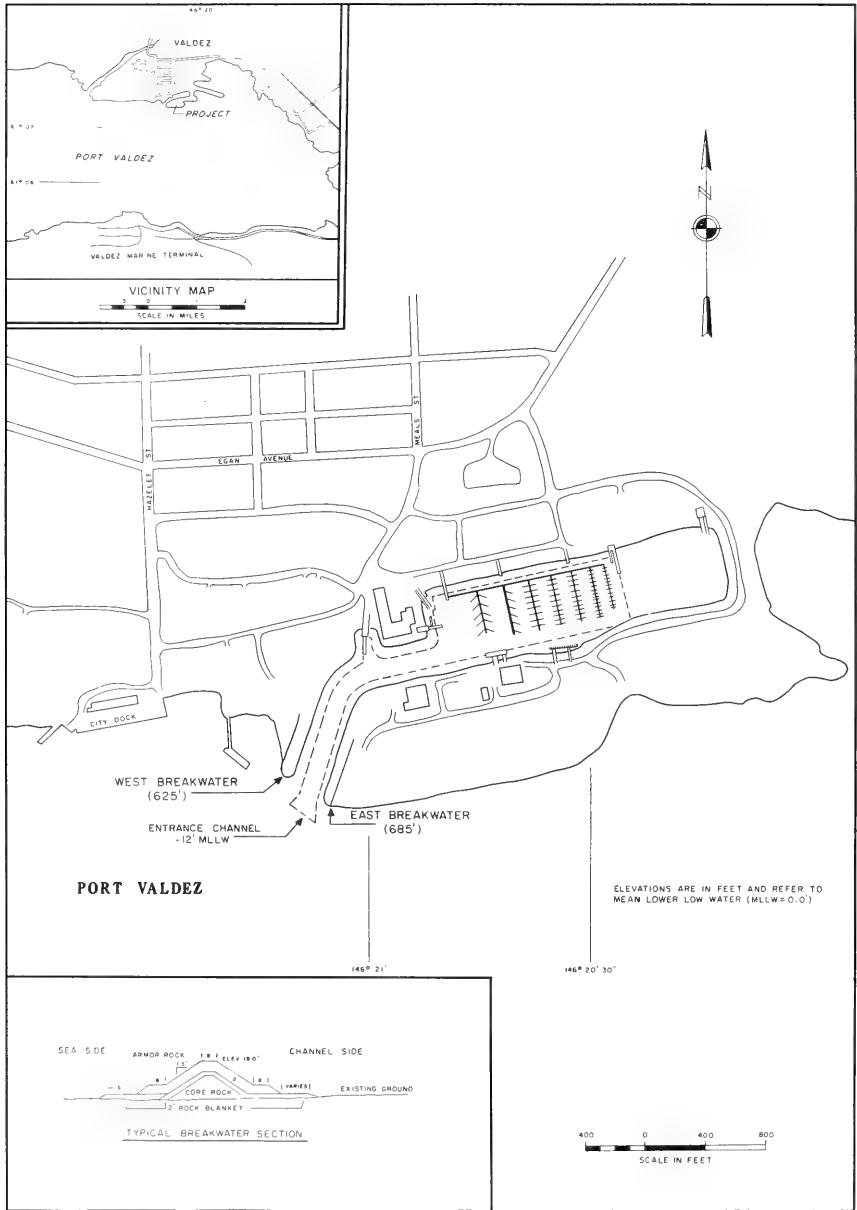
Figure 48. Site layout of Valdez Harbor, Alaska, 1985
