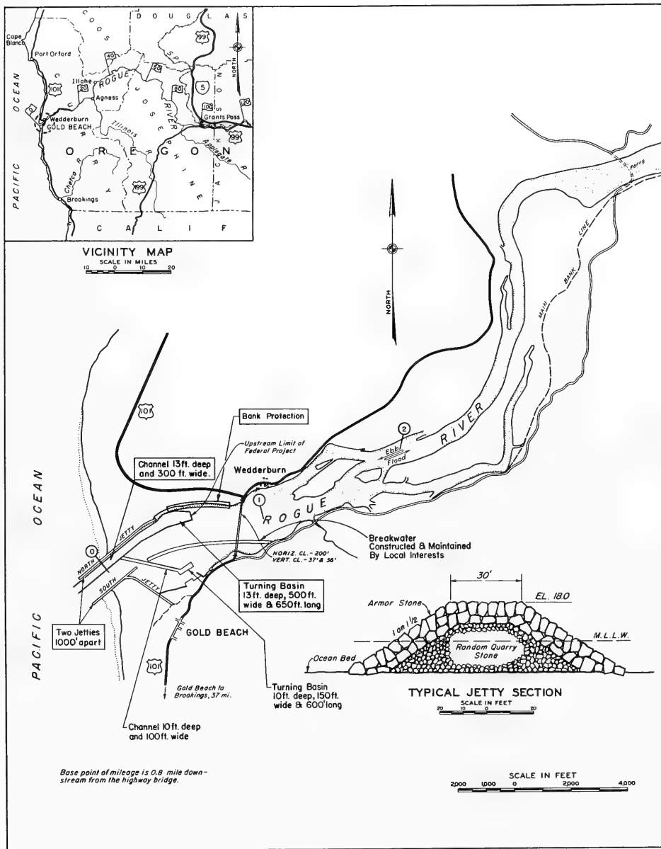
Figure 59. Site layout at Rogue River, Oregon (revised 1977)
