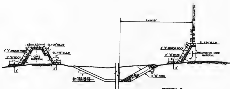
SECTION E NOT TO SCALE TYPICAL ENTRANCE BREAKWATER AND NORTH BREAKWATER STA 6+00 TO STA 7+00
