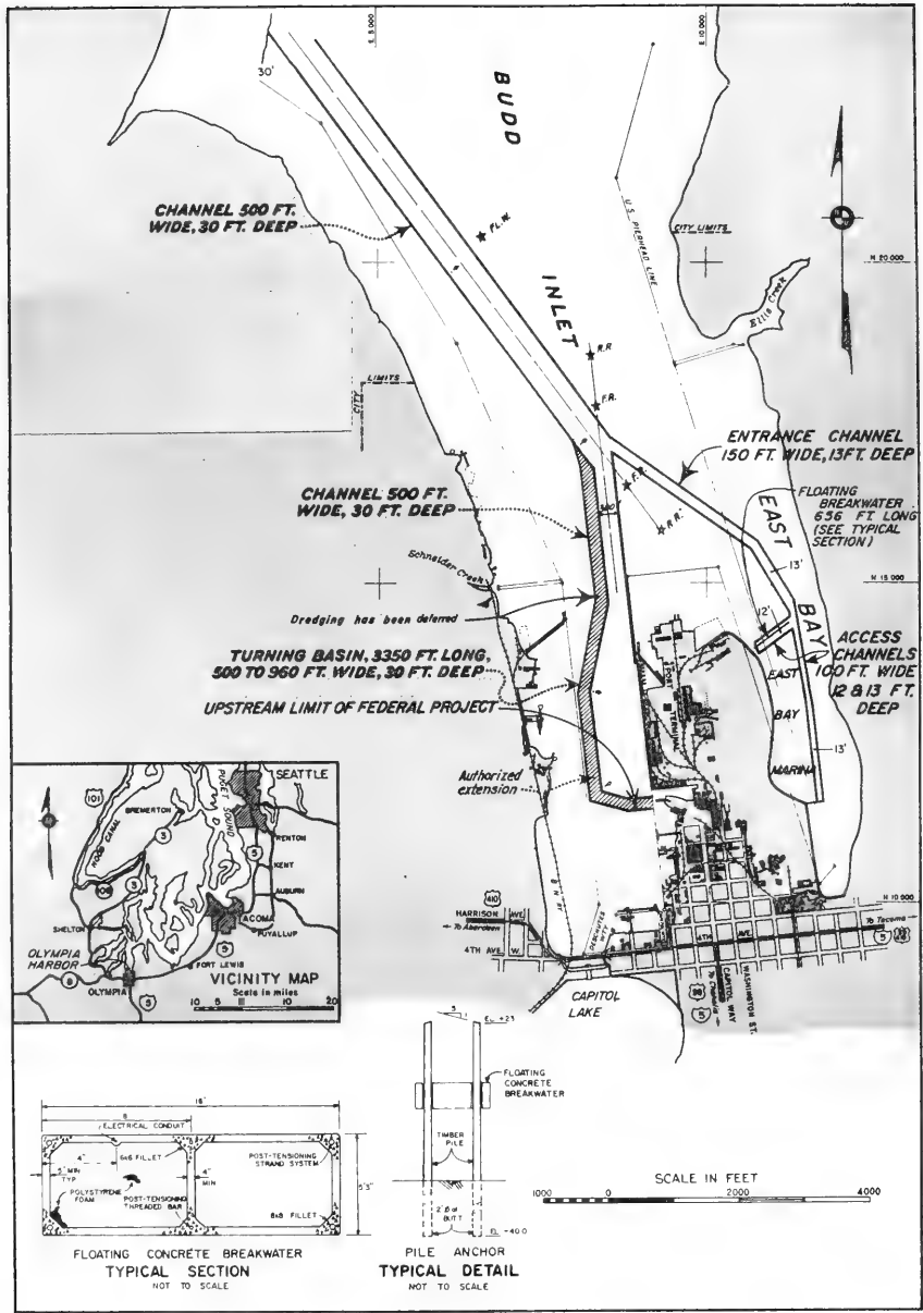
Figure 74. Site layout of Olympia Harbor, Washington (revised 1982)
