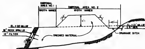
SECTION D E.T.S.
