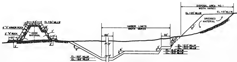
SECTION A NOT TO SCALE TYPICAL WEST BREAKWATER STA 0+00 TO STA 15+07.09
