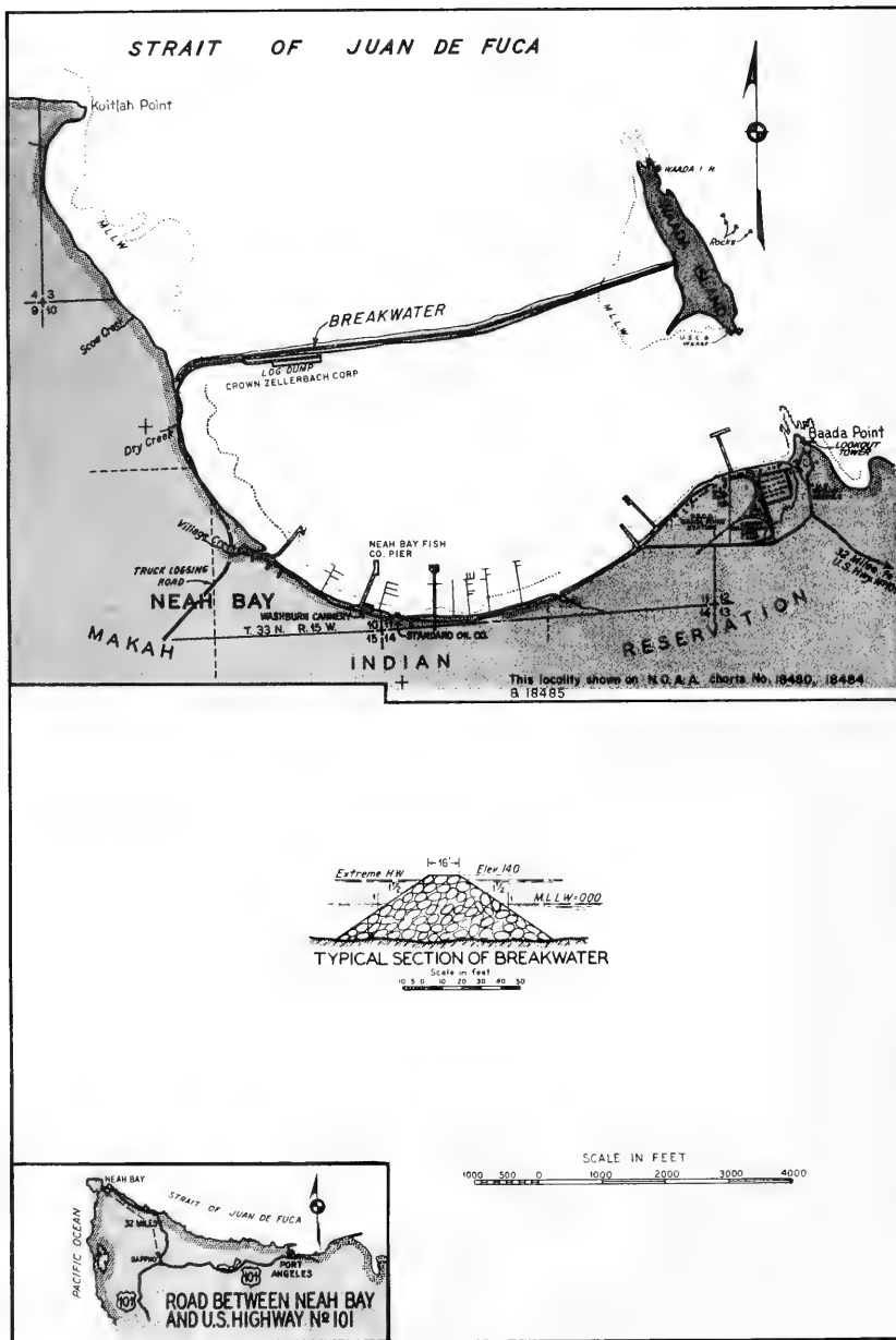
Figure 73. Site layout at Neah Bay, Washington (revised 1979)
