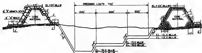
SECTION B
