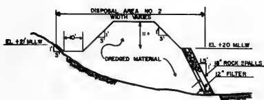
SECTION C E.T.S.
