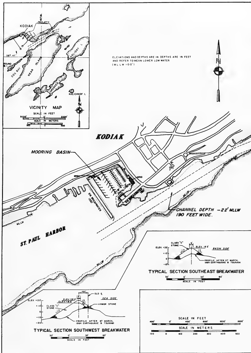
Figure 27. Site layout of Kodiak Harbor, Alaska (revised 1978)
