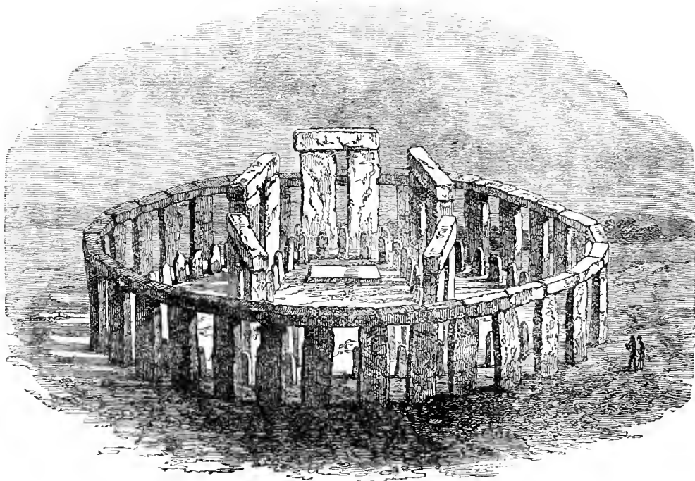
Stonehenge (restored).
