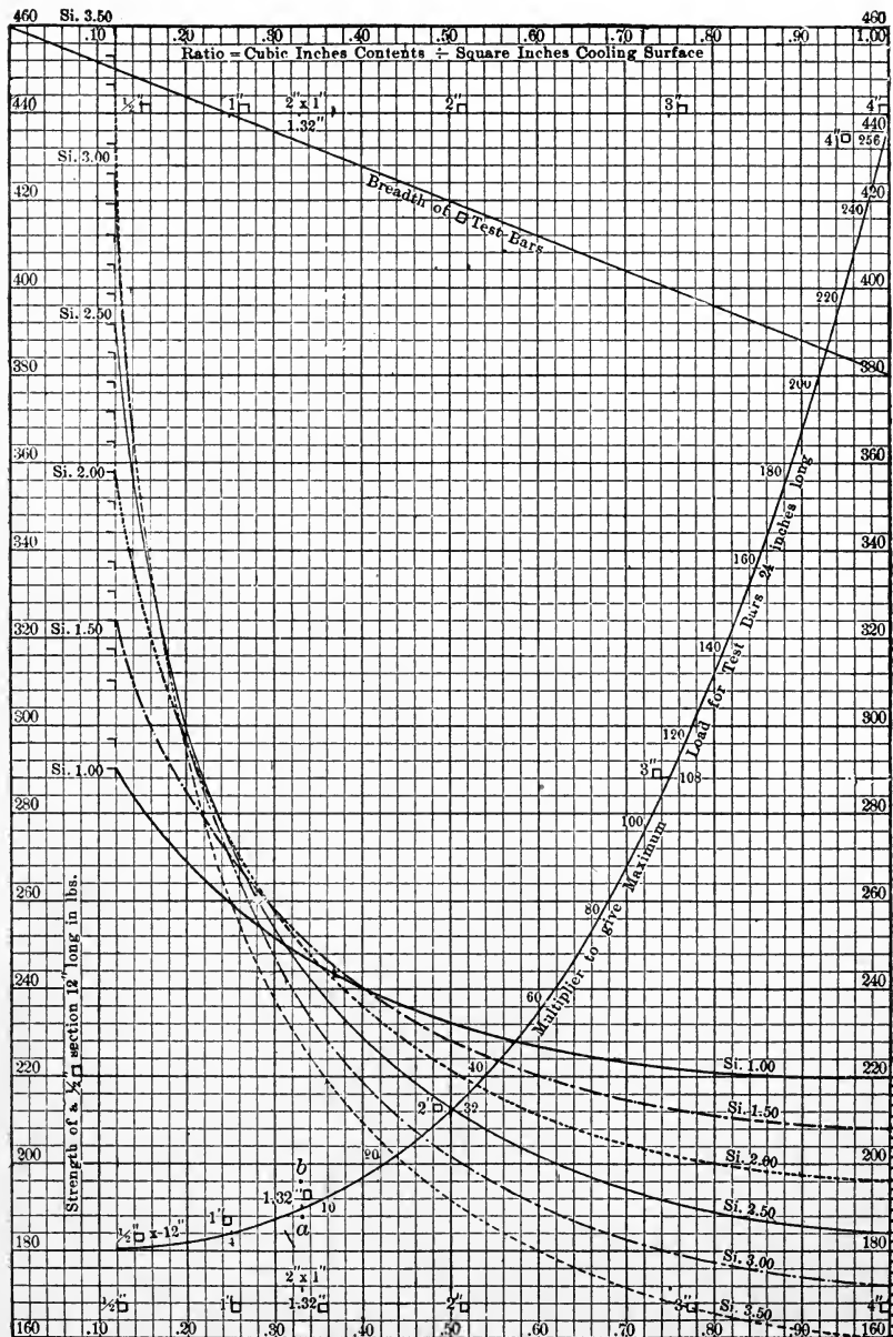
FIG. 82.—Keep's Strength Chart.—Approximate Relation of Strength to Size and Percentage of Silicon. (Strength of a \frac{1}{2}'' \square \times 12'' section of each Size of Test-bar.)
