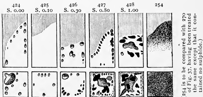
FIG. 40.—White Pig Iron + Iron Sulphide.
