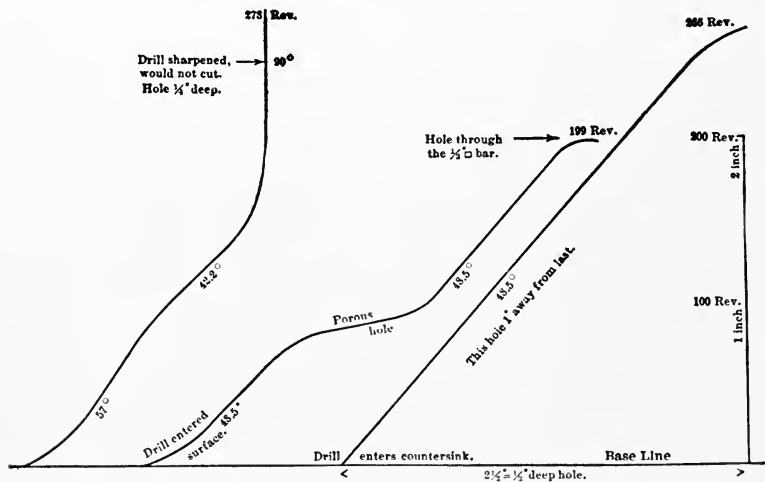
FIG. 84.—Hardness Diagram.
