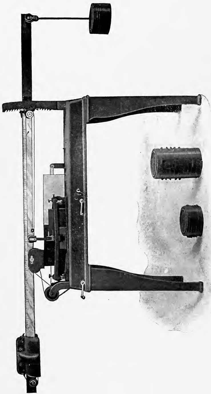
FIG. 92.—Keep's Dead-load Testing Machine, No. 40.
