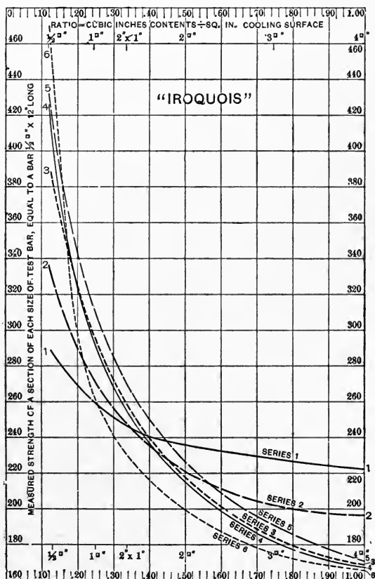
FIG. 57.—Curves of Fig. 56 made uniform.
