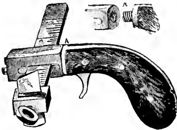
No. 52—Draw Gauge, Latta's Pattern, with Trigger. Each . . .
