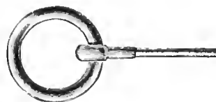
No. 975—Back Strap Rings, Polished Welded Steel, 1 1/2 inch stock, 1 1/2 inch ring, 2-11/16 inch Stud. 2 Dozen in Box. Per Dozen.....
