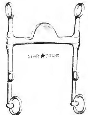
1779 No. 1779-WEYMOUTH- Light weight, 4 5/8" Mouth, 7 1/2" Solid Cheeks, (Tom Bass Pattern), Solid Port so that it rests evenly on the horse's tongue. Also increases strength. Star Steel Silver. Each .....
