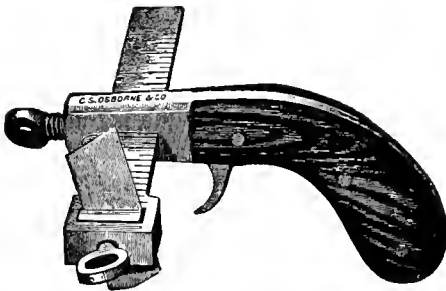
No. 52 1/2—Draw Gauge, Iron Frame with Trigger Each . . .
