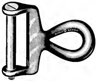
465—SCREW COCKEYE
