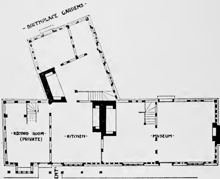
-GROUND PLAN-
