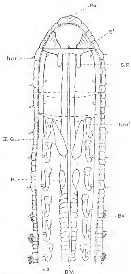
Fig. 47.— A. glacialis . Diagram of a dissection of the anterior portion. Br¹, First gill; D.V. Dorsal blood-vessel; H. Heart; Not¹, First notopodium; NPH¹, First nephridium; E.G.L., Esophageal gland; PR, Prostomium; S¹, First septum; S.P. Septal pouch.
