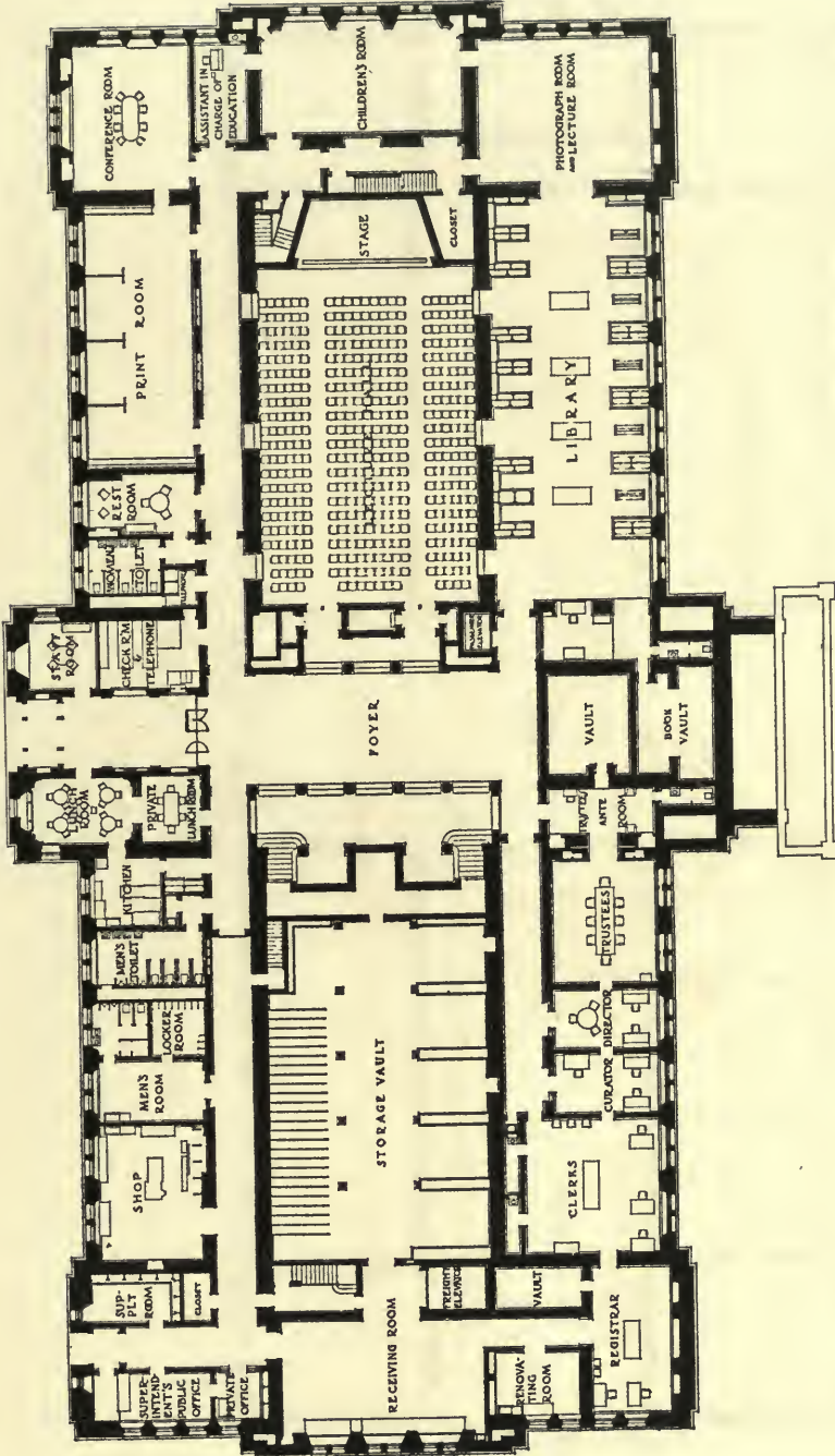
GROUND STORY PLAN SCALE 1/8" = 1'-0"
