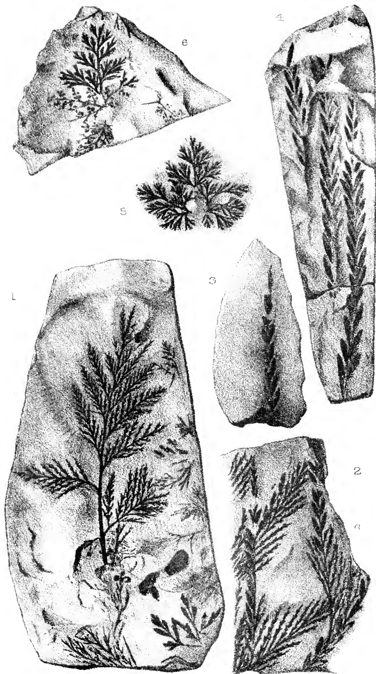
Onychiopsis & Ruffordia .
