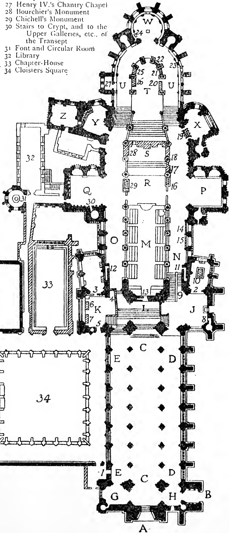
PLAN OF CANTERBURY CATHEDRAL
