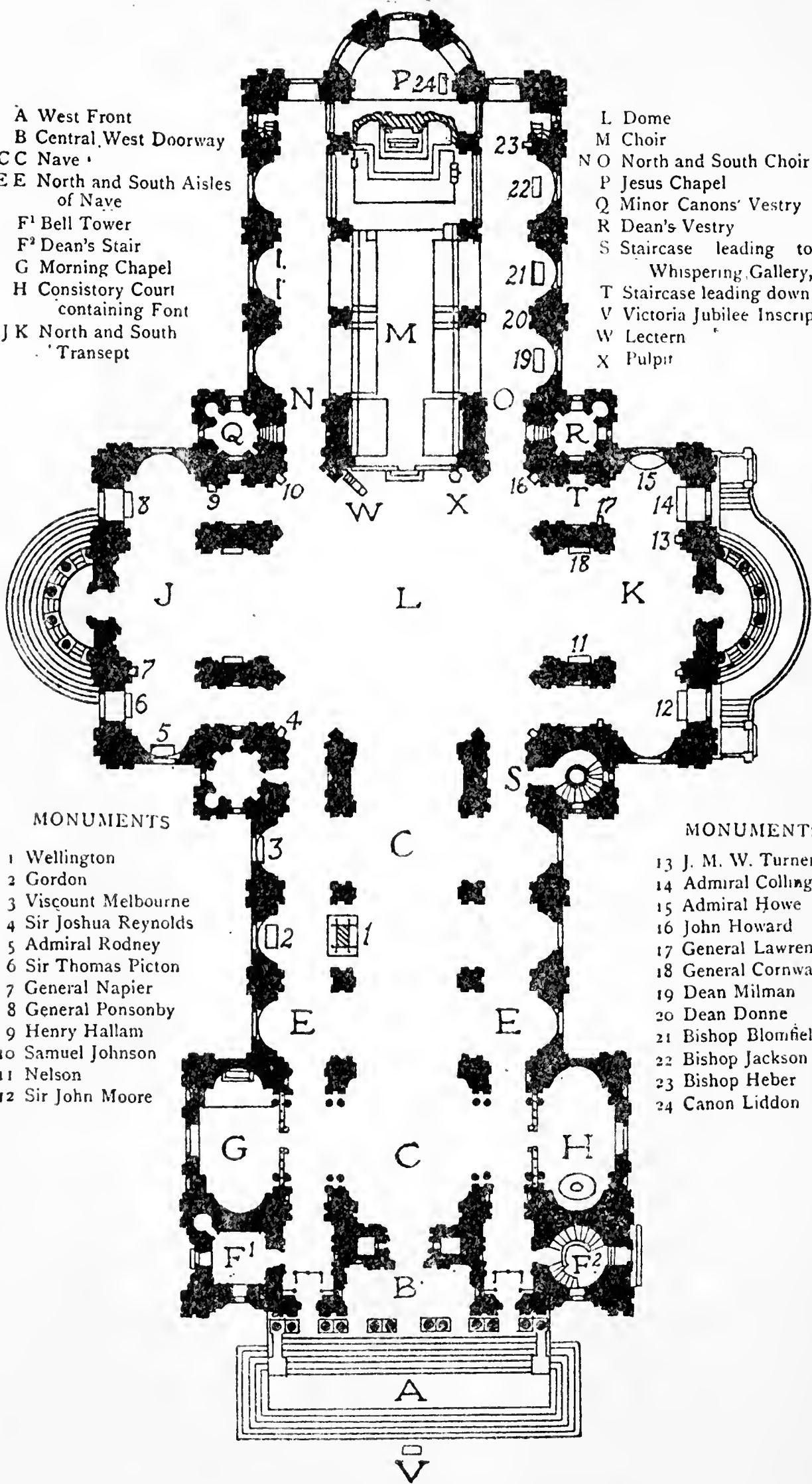
PLAN OF ST. PAUL'S CATHEDRAL
