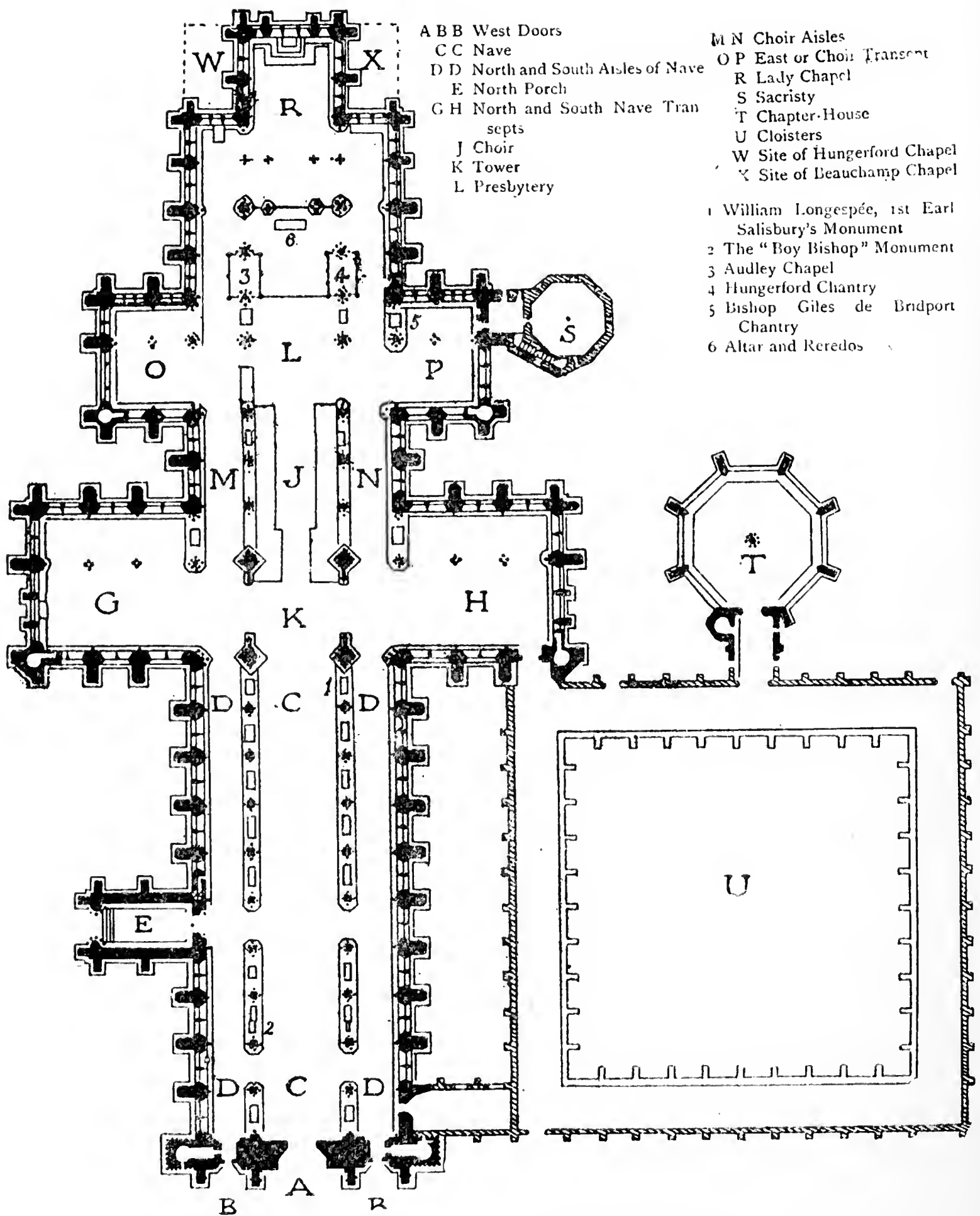
PLAN OF SALISBURY CATHEDRAL
