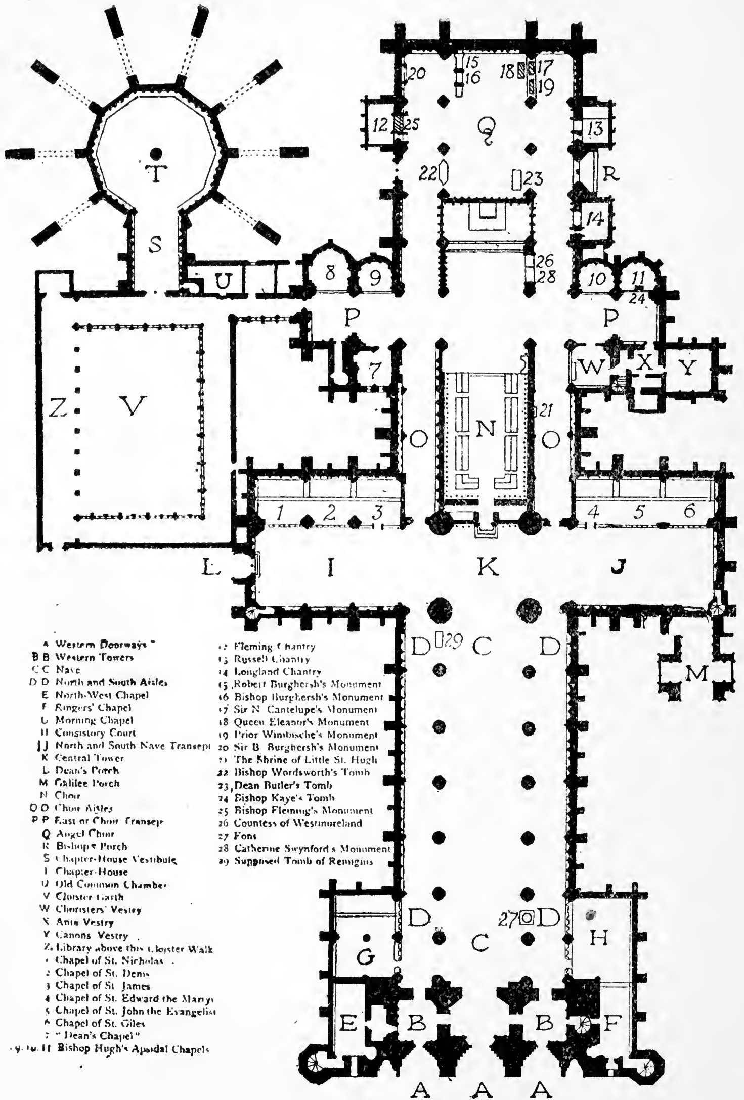
PLAN OF LINCOLN CATHEDRAL
