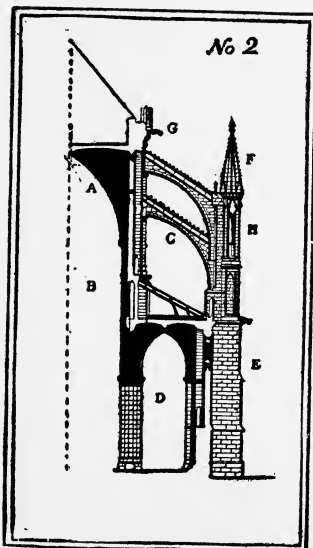
No. 2. CROSS SECTION
