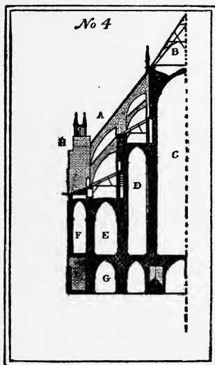
No. 4. CROSS SECTION
