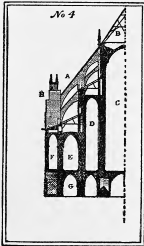
No. 4. CROSS SECTION
