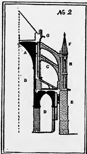
No. 2. CROSS SECTION
