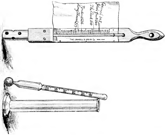
SUGAR THERMOMETER AND STICK GAUGE. (SEE PAGE 510.)
