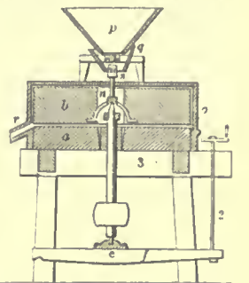
Grinding-mill.
