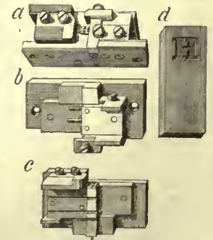
Details of Type-mold. a , the two halves of the mold united but without the matrix, showing the face of the type H as formed in the mold; b , one half of the mold; c , the other half of the mold, showing the body of the letter H in position; d , the matrix relatively enlarged, showing the face of the letter H.
