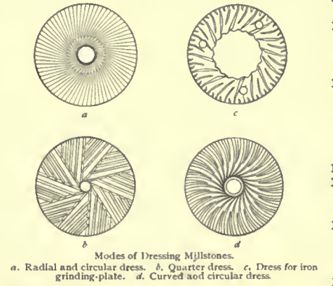
Modes of Dressing Millstones.
