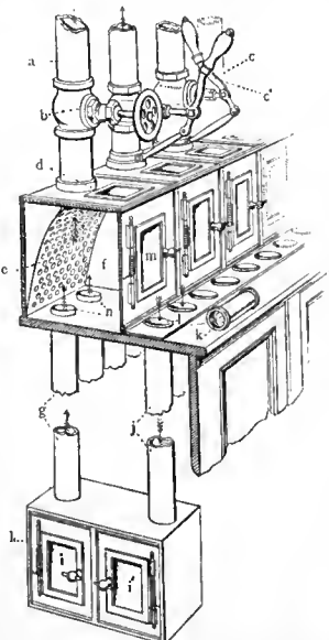
Pneumatic Tubes.
