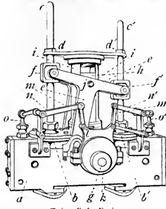
Twin-cylinder Engine.
