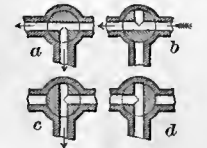
Two-way Cock. a, position which distributes water to two branches; b, c, positions in which the water is passed through only one branch; d, position for stopping flow.
