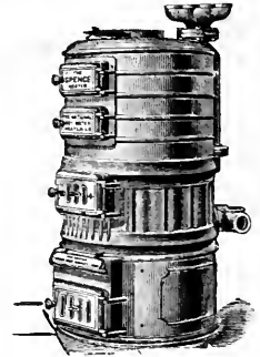
THE "SPENCE."
