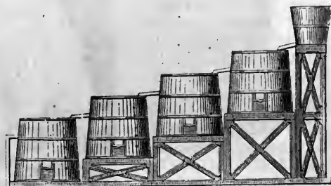
"FLOATING" GRAPHITE THROUGH THE TUBS.
