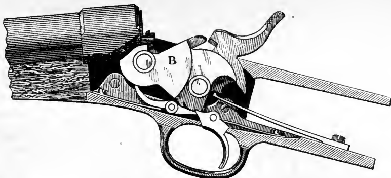
BREECH MECHANISM OF THE REMINGTON RIFLE.
