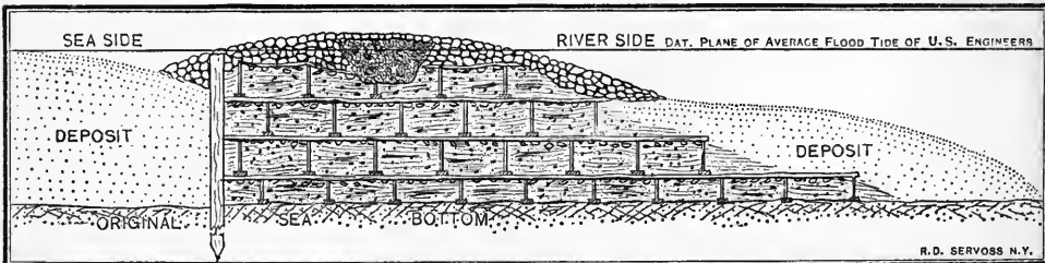
SECTION OF JETTY, 7,500 FEET SEAWARD FROM LAND'S END. SCALE, TEN FEET TO ONE INCH.
