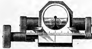
WIND SIGHT AND SPIRIT LEVEL.
