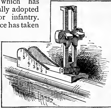
SPRINGFIELD REAR SIGHT.
