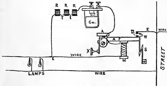
FIG. 12. DIAGRAM OF METER AND SYSTEM.
