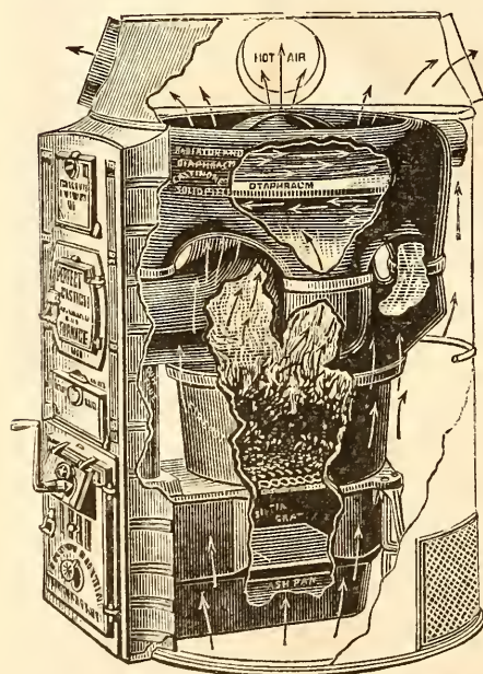
"PERFECT" WARM AIR FURNACE.
