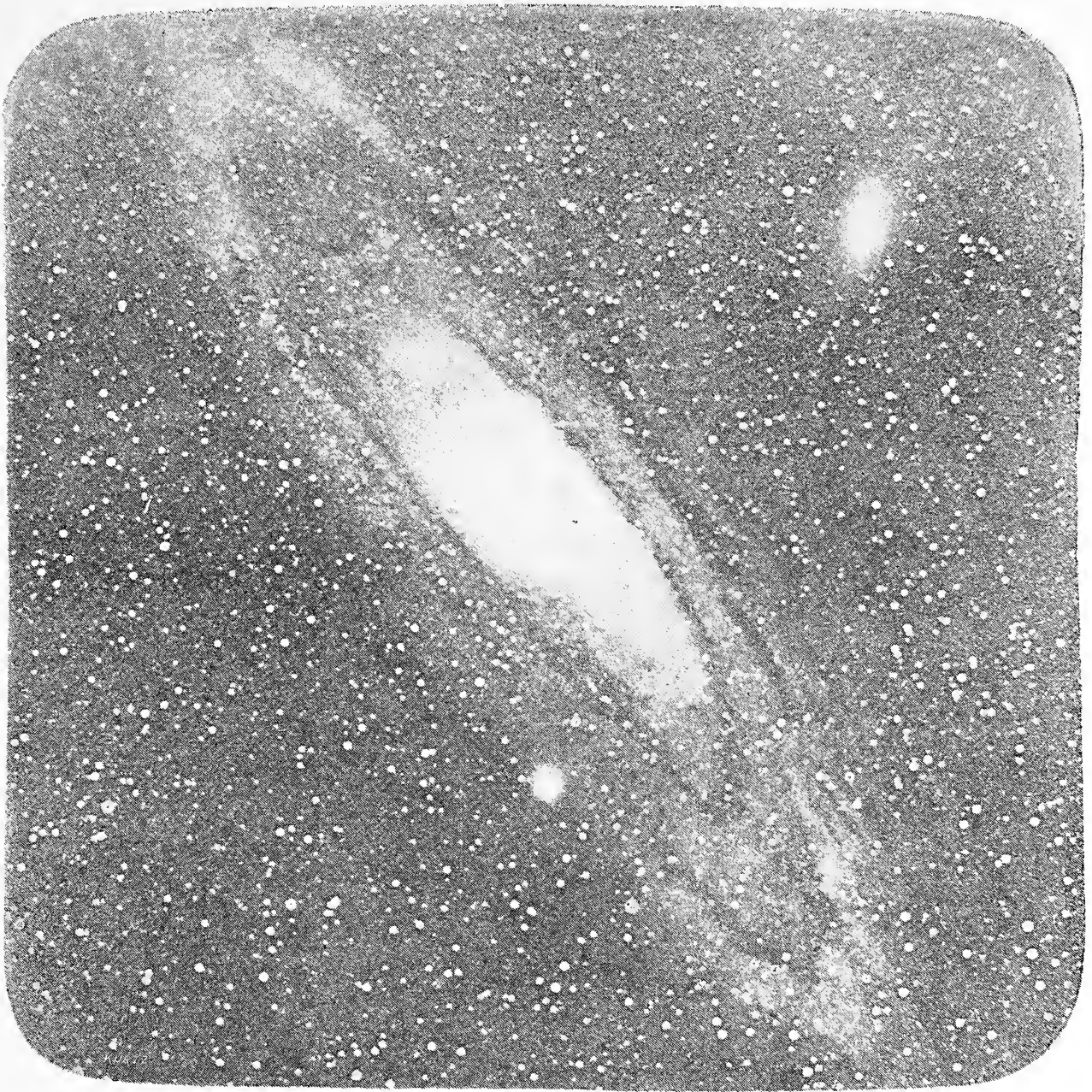
NEBULA IN ANDROMEDA.
