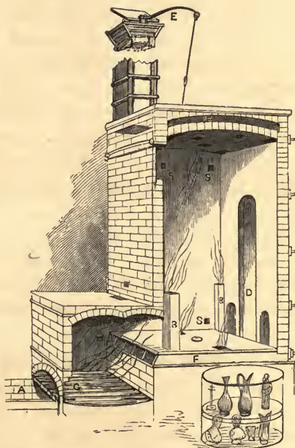
Fig. 29.—Broome's Improved Porcelain or Parian Kiln. A, ash-pit; G, grate; F F, flues; B B, bags for the flames; D, door for filling the kiln; E, damper, or draught regulator; S S S, spy-holes for watching, or trials while burning.
