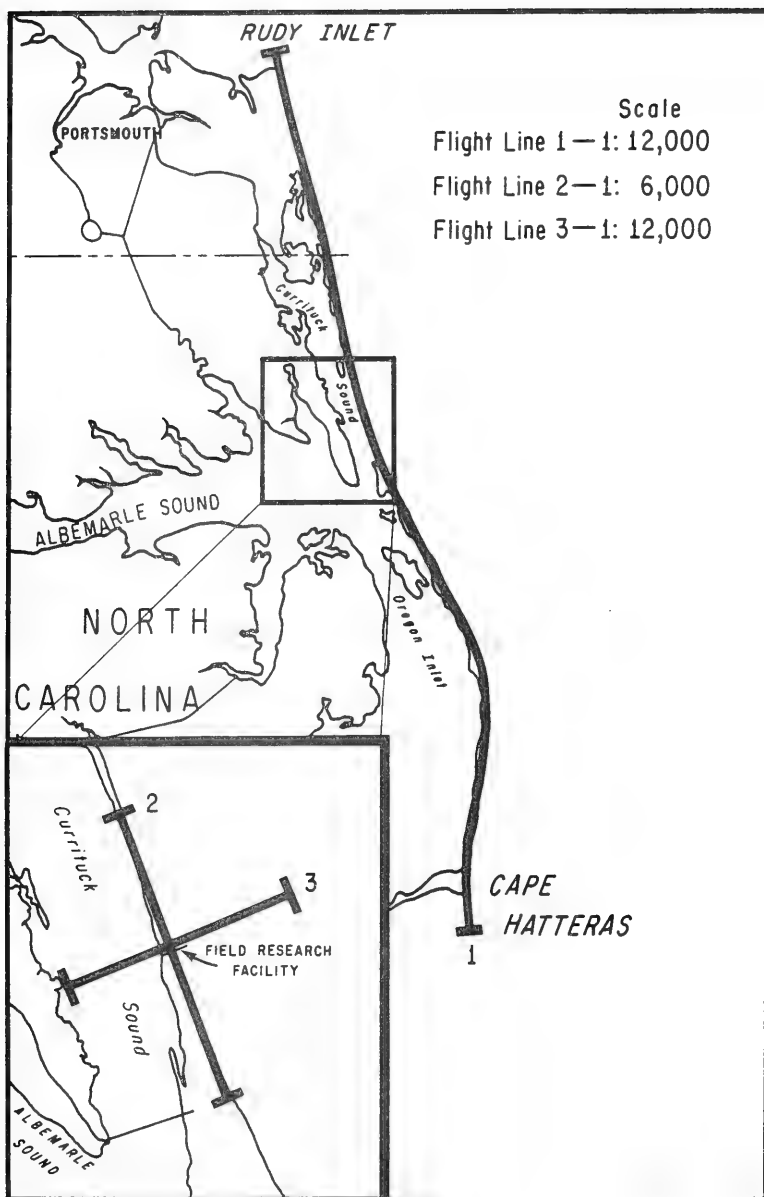
Figure 5. Flight lines for aerial photography missions.
