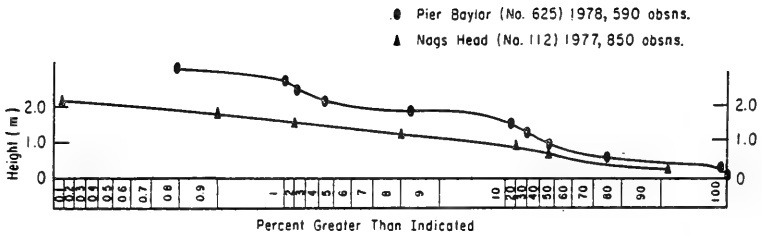
Figure 8. Annual cumulative significant wave height distributions at Nags Head and the FRF pier-end Baylor gages.
