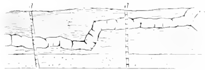
Fig. 3.—Intrusive Sheet and Dykes: i , igneous intrusive sheet; d, d , dykes; s, s , sedimentary strata.
