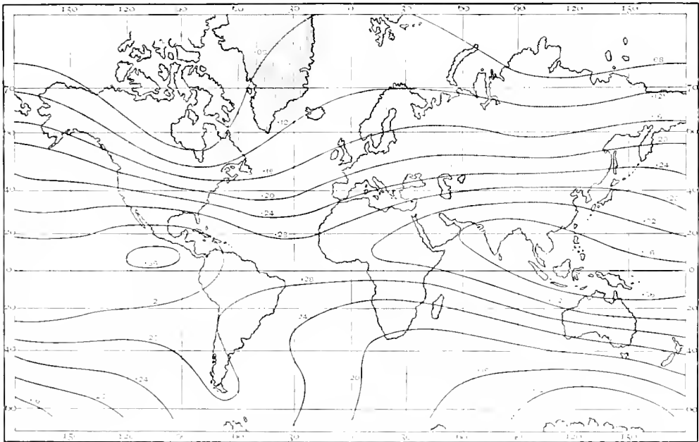
Fig 4.—Lines of equal Horizontal Force, 1855.
