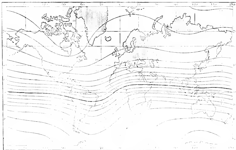
Fig. 1.—Lines of equal Magn. Dip. 1887.
