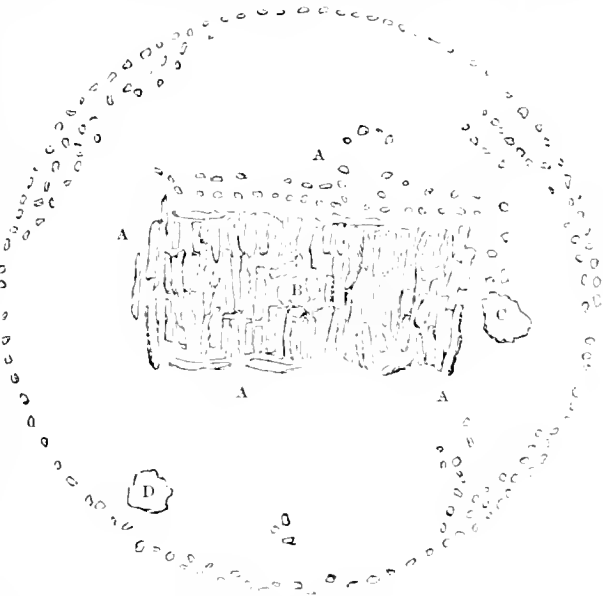
Fig 2.—Ground-plan of Crannog in Drumaleague Lough.
