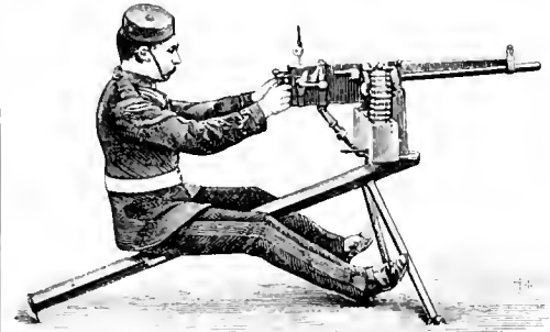
Fig. 5.—Rifle-calibre Maxim Gun.
