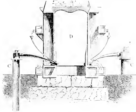
Fig. 7.—Finery.
