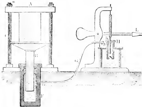
Hydraulic Press.
