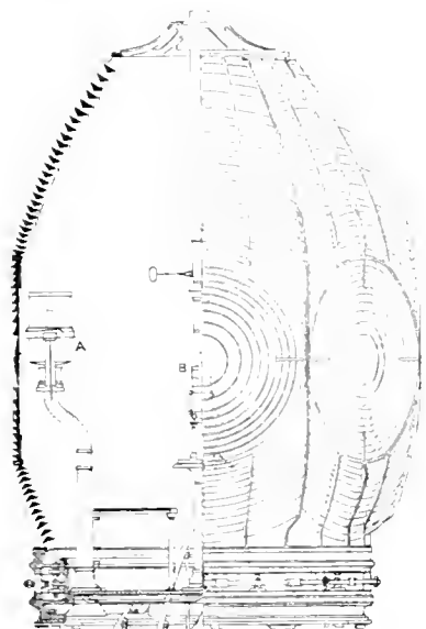
Fig. 6. Stevenson's Hyper-radiant Light.
