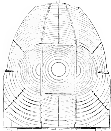
Fig. 5.—Holophotal Triple-flashing Light, first order.
