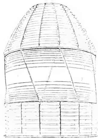
Fig. 7. Fixed Light, first order.
