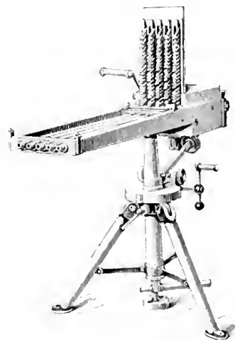
Fig. 3. Five-barrelled Gardner Gun on Tripod Stand.
