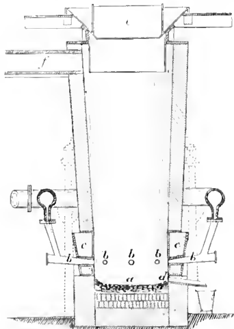
Fig. 2. Vertical Section of the Pilz Blast-furnace for melting lead: a, hearth; b, tuyères, by which air-blast enters; c, water-jacket; d, tap-hole; e, cover; f, flue.
