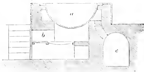
Fig. 3.—Desilverising Pot: a, pot; b, fireplace; c, main flue.
