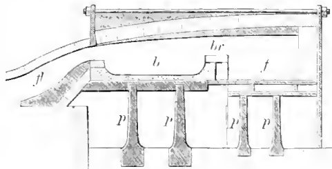
Fig. 8.—Puddling Furnace, vertical section.
