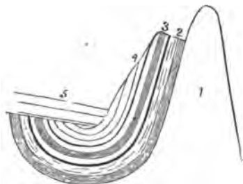
Fig. 2.—Principal System of the Alps : 1, Granitic rocks; 2, Palæozoic; 3, Secondary; 4, Tertiary; 5, Recent.
