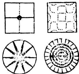
Nodal Points.
