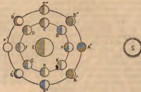
Fig. 1.—Phases of the Moon:
