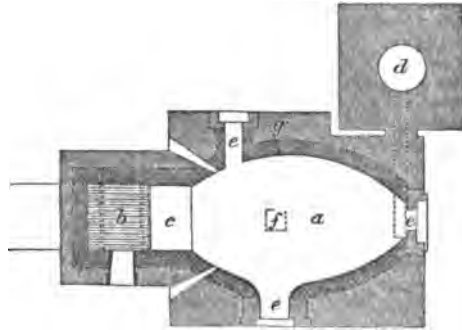
Fig. 2.—Plan of a Reverberatory Lead Furnace: a, hearth on which the ore is spread; b, fireplace or grate; c, the fire bridge; d, chimney; e, working doors; f, opening for supplying ore; g, tap-hole.
