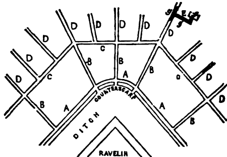
Fig. 3.—System of Countermines:
