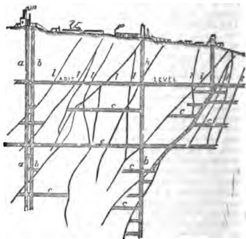
Fig. 2.—Cross-section of a Cornish Mine.
