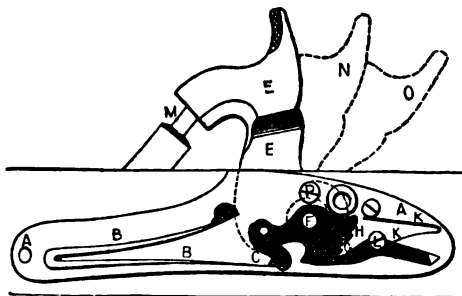
Percussion-lock.
