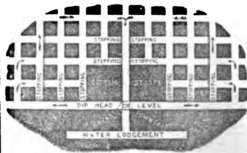
Fig. 8.—Plan of part of a Coal Mine, shewing 'Stoop-and-Room' Workings.
