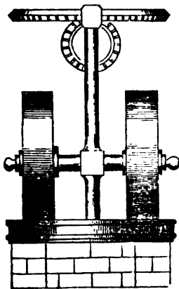
Fig. 4.—Edge-stone Mill
