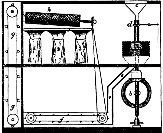
Fig. 3.—Elementary Section of a Flour-mill.
