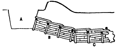
Fig. 2.—Mine supported by Frames, in process of construction from a Trench: A, trench; B, descending gallery; C, gallery; a, roofing plank not yet pushed out to its full length.
