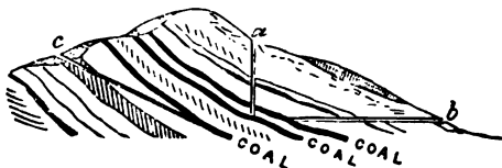
Fig. 7.—Diagram shewing methods of 'winning' the Coal.
