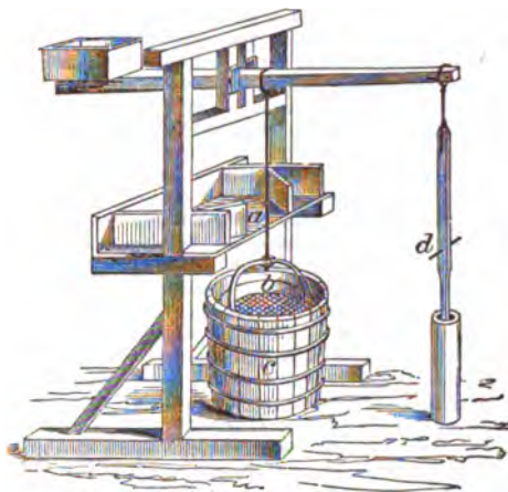
Fig. 3.—Jiggling Sieve.
