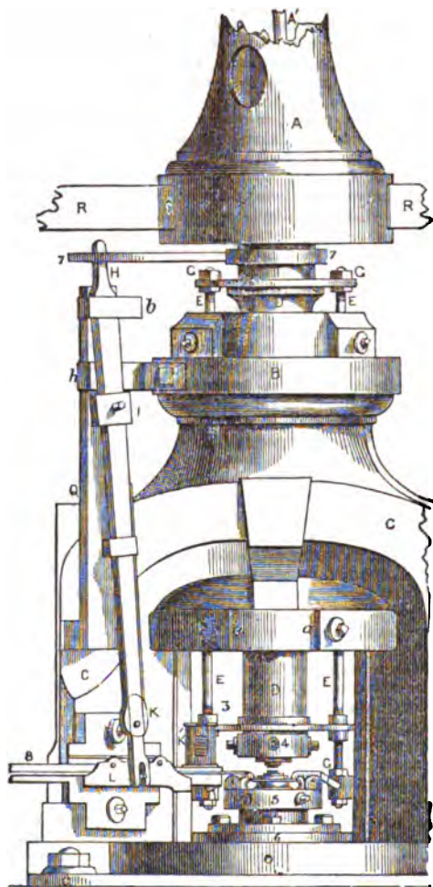
Coining-press.
