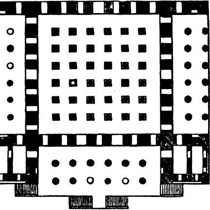
Fig. 2—Plan of Great Hall of Xerxes at Persepolis.
