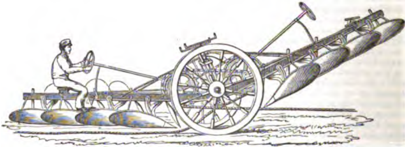
Fig. 11.—Fowler's Plough.
