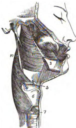
Fig. 2. —External View of the Muscles of Pharynx : 1, the orbicularis oris muscle; 2, the Buccinator muscle; 3, portion of lower jaw, part of which is cut away; 4, pyriform-mazillary ligament; 5, the hyoid bone; 6, the thyroid cartilage; 7, the bicoid cartilage; 8, the trachea; 9, the œsophagus, with the recurrent laryngeal nerve lying between it and the trachea; 10, the stylo-pharyngeal muscle; 11, 12, 13, the superior, middle, and inferior constrictor muscles.
