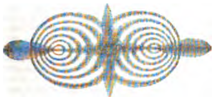
Fig. 4.—Biaxial Crystal; Black Cross.
