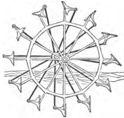
Feathered Paddle-wheel.
