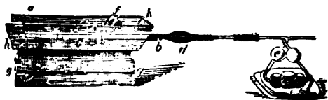
a, b, the combustion tube; c, the central portion, in which the mixture to be analysed is placed; d, the bulb-tube, containing chloride of calcium; ee, Liebig's potash apparatus; f, a movable iron screen; gg, bricks supporting AA, the furnace.
