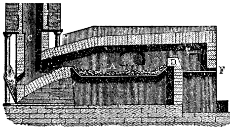
Fig. 3.—Puddling Furnace.
