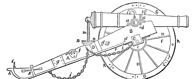
Field Gun and its Carriage :
