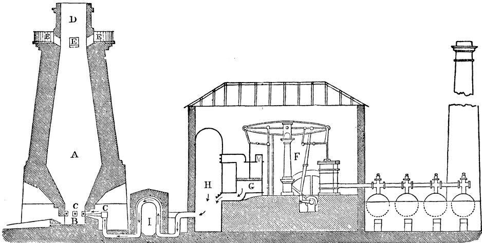
Fig. 1.—Hot Blast-furnace.
