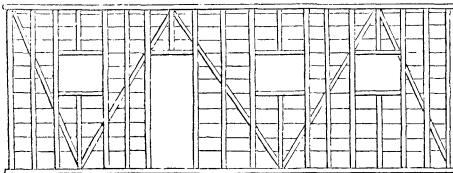
Fig. 3.—Side of a framed Hut.
