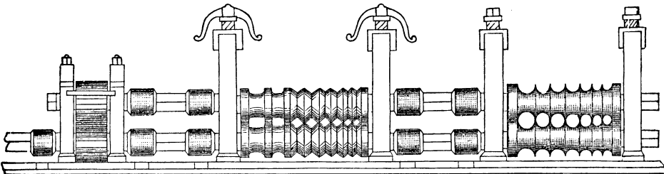
Fig. 5.—Rough and Finishing Rolls.
