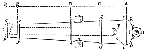
32-pounder Gun :
