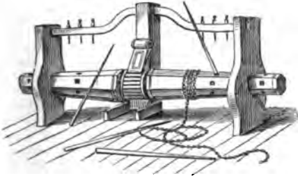
Fig. 1.—Ship's Windlass.
