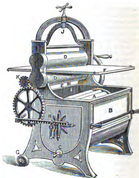
Dash-wheel Washing-machine :
