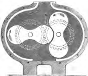
Fig. 9.—Roots' Blowing-machine.
