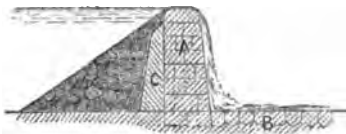
Fig. 5. A, masonry; B, pitching; C, clay puddle.
