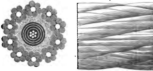
Section and External Appearance of Atlantic Cable of 1866.
