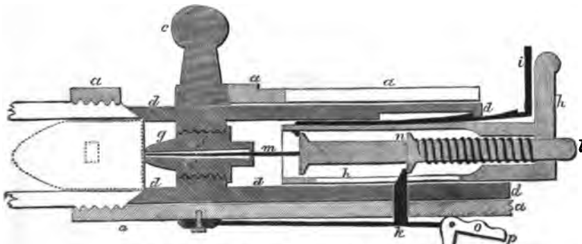
Fig. 6.—Section of Prussian Needle-gun: Half-cock.
