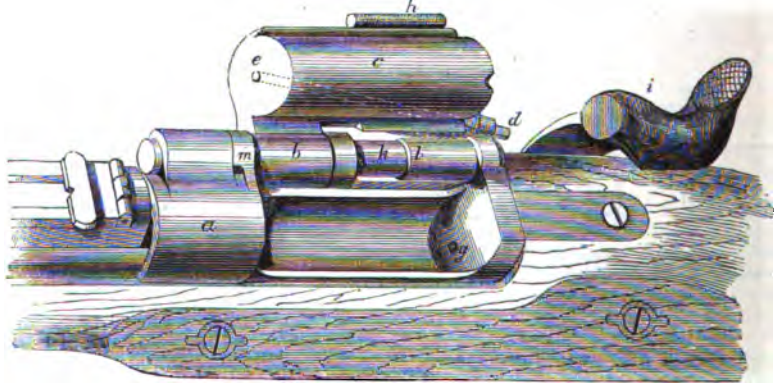
Fig. 8.—Snider : Open.
