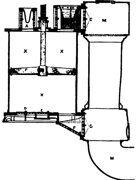
Fig. 5.—Section of a Blowing Cylinder, Shelton Iron-works, Stoke-upon-Trent.
