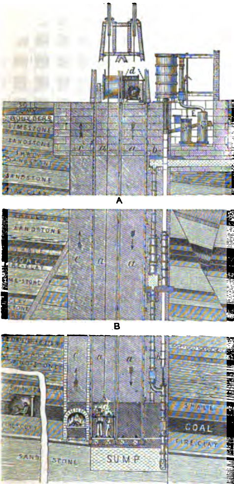
Fig. 9.—Vertical Section of the Shaft of a Coal-pit, with a Detached Portion, shewing a Miner at work on the Coal Seam.
