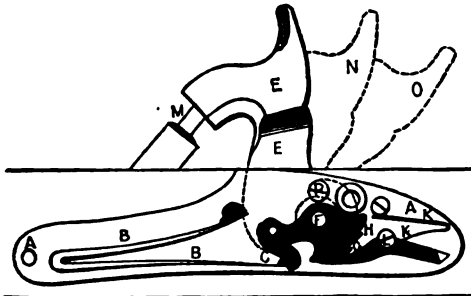
Percussion-lock.
