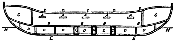
Fig. 1.—Section lengthwise.
