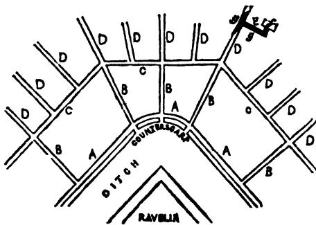
Fig. 3.—System of Countermines:
