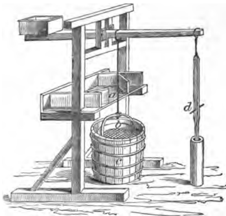
Fig. 3.—Jiggling Sieve.
