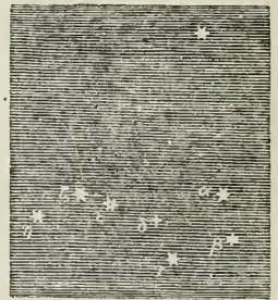
Constellation of the Plough.
