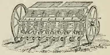
Corn-drill.
