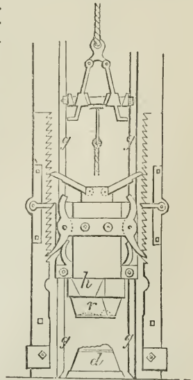
Stamping-machine.
