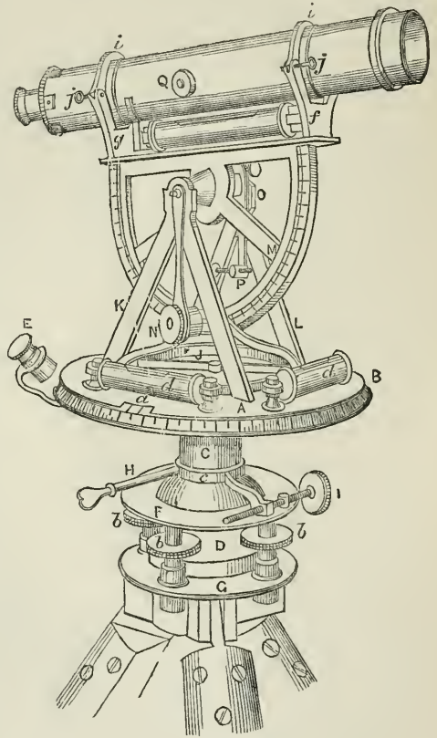
Theodolite:
