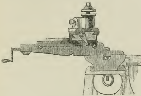
Fig. 2.—Slide-rest.
